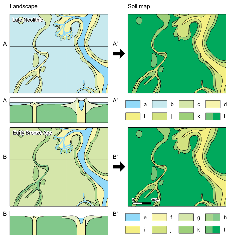
Figure 3.13: The relation between the former landscape and the present day soil map of eastern West-Frisia. Legend: a salt to brackish water, b brackish to freshwater and or reed swamps, c irregularly flooded levees and creekridges, d regularly flooded flats, splays and residual gullies, e salt to brackish water, f tidal flats, g irregularly flooded tidal marsh, h regularly flooded tidal marsh and former gully, i loamy sand to sandy loam, j sandy loam to loam, k (silty) clay loam with intercalated layers of loamy sand or sandy loam, l (silty) clay loam.
