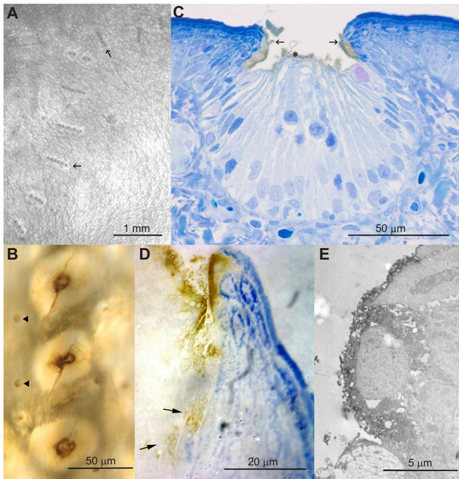
Fig. 1. Melanopsin immunostaining of Xenopus laevis neuromasts. (A) Low power wet mount of the dorsal skin showing linear arrays of stained neuromasts (arrows) forming lateral line stitches. (B) Higher power wet mount of three neuromasts within one stitch emphasising dense staining at the centre of the neuromast, with fine processes emanating from it. Arrowheads indicate putative melanopsin-positive melanophores. (C) Light microscopic section through the centre of a stained neuromast highlighting the presence of melanopsin in cells at the pore margin (arrows). The superficial immunostaining in the region of hair cell stereocilia and kinocilia (asterisk) is most likely artefactual. (D) Section showing the lateral region of a stained neuromast highlighting melanopsin location deeper in peripheral cells of the organ (arrows). (E) Electron micrograph through a stained cell at the pore margin. The darker areas of the cytoplasm indicate the intracellular location of melanopsin. The nucleus is the spherical lighter (unstained) area. The regions depicted in D and E are from an area equivalent to the stained (brown) tissue at the upper right corner of the neuromast shown in C.
