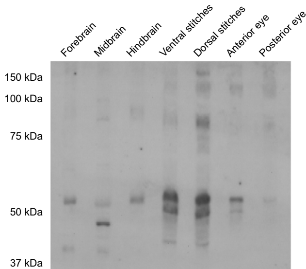
Fig. 2. Western blot analysis of melanopsin expression in various tissues of Xenopus laevis . The blots were screened with antibody CERN972. The upper immunoreactive bands near 55 kDa represent full-length OPN4m and/or OPN4x. The lower immunoreactive bands may either represent full-length OPN4m (complete sequence is not known currently), or smaller splice variants of OPN4m and/or OPN4x. See body of text for further details.
