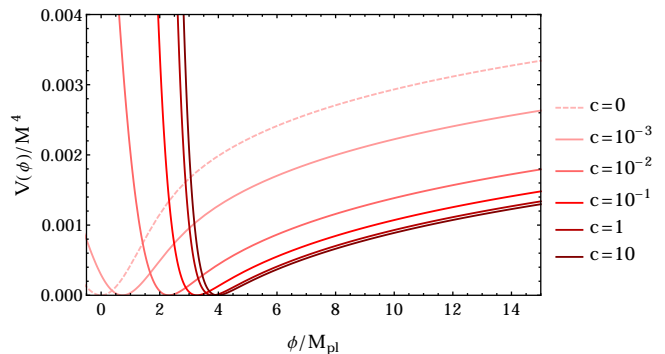
FIG. 1. The dependence of the potential from Eq. (44) on the parameter c . Note that the shape does not change for c \gtrsim \mathcal{O}(1) . Here, we choose E \sim -10^{-3} .
