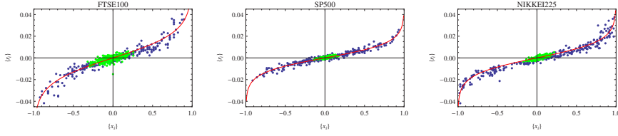
Figure 1.12: Characterization of empirical relations between binary and non-binary properties in financial time series. Nonlinear relationship between the average daily increment (weighted return) and the average daily sign (binary return) over all stocks in the FTSE100 (left), S&P500 (center) and NIKKEI225 (right) in various years (2003, 2007, and 2004 respectively). Here each point corresponds to one day in the time interval of 250 trading days (approximately one year). The red curve is our non-parametric prediction based on the fit shown in fig.1.11, and the green points are the same properties measured on the shuffled data.
