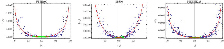
Figure 1.13: Characterization of empirical relations between binary and second-order non-binary properties in financial time series. Nonlinear relationship between the average daily coupling (weighted coupling) and the average daily sign (binary return) over all stocks in the FTSE100 (left), S&P500 (center) and NIKKEI225 (right) in various years (2003, 2007, and 2004 respectively). Here each point corresponds to one day in the time interval of 250 trading days (approximately one year). The red curve is our non-parametric prediction based on the fit shown in fig.1.11, and the green points are the same properties measured on the shuffled data.
