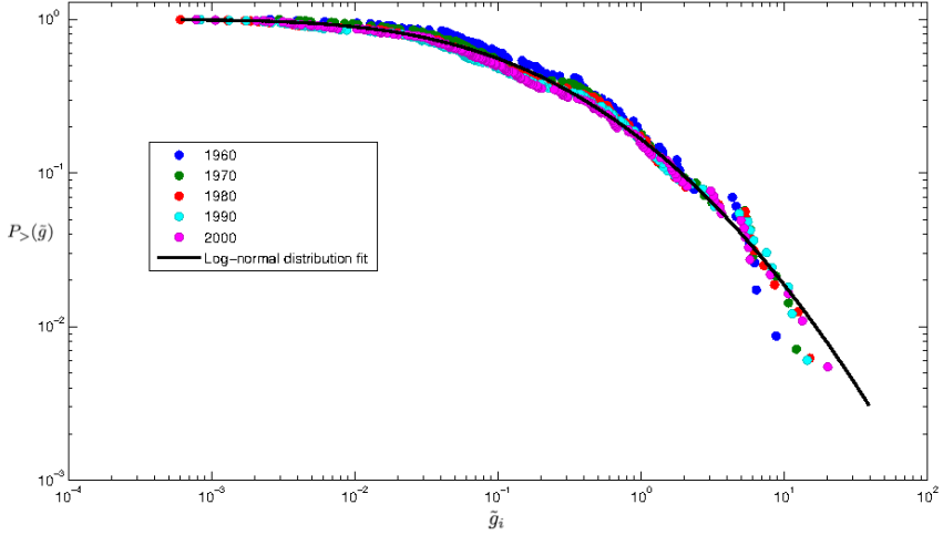
Figure 2.3: Cumulative Distribution of countries GDP for different decades. Empirical cumulative distributions P_{>}(\tilde{g}) of the GDP rescaled to the mean, for different years. The curve is a log-normal distribution fitted to the data.
