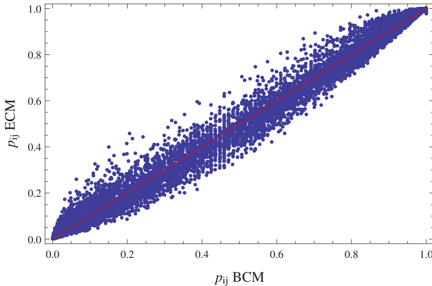
Figure 2.7: Link formation probability for the different models. The probability of forming a link in the ECM p_{ij} \text{ ECM} compared to the probability in the BCM p_{ij} \text{ BCM} for the undirected binary aggregated ITN in the 2002 snapshot. The red line describes the identity line.
