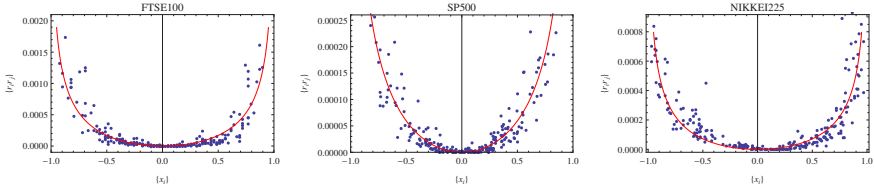
Figure 1.3: Empirical relations between binary and second-order non-binary properties in financial time series. Nonlinear relationship between the average daily coupling (weighted coupling) and the average daily sign (binary return) over all stocks in the FTSE100 (left), S&P500 (center) and NIKKEI225 (right) in various years (2003, 2007, and 2004 respectively). Here each point corresponds to one day in the time interval of 250 trading days (approximately one year). The red line represents the best fit with the function y = b \cdot (\text{artanh}x)^2 , whose use is theoretically justified later in sec. 1.6.
