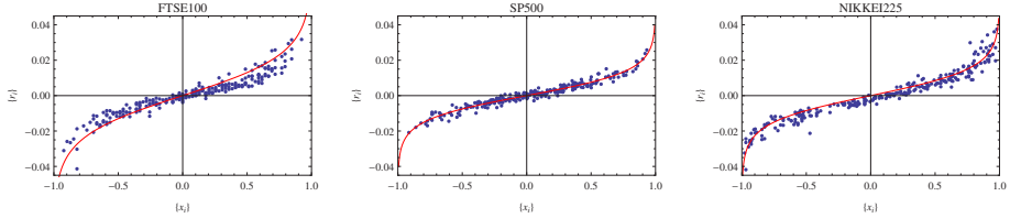
Figure 1.2: Empirical relations between binary and non-binary properties in financial time series. Nonlinear relationship between the average daily increment (weighted return) and the average daily sign (binary return) over all stocks in the FTSE100 (left), S&P500 (center) and NIKKEI225 (right) in various years (2003, 2007, and 2004 respectively). Here each point corresponds to one day in the time interval of 250 trading days (approximately one year). The red line represents the best fit with the function y = a \cdot \text{artanh}x , whose use is theoretically justified later in sec. 1.6.
