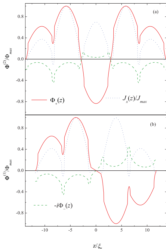
FIG. 10. (Color online) Eigenvector functions and supercurrent density J_s(z) calculated for the F/[5(S/F)] multilayer with (a) enlarged thickness of the two central F layers and (b) with reduced thickness of the central S layer.
