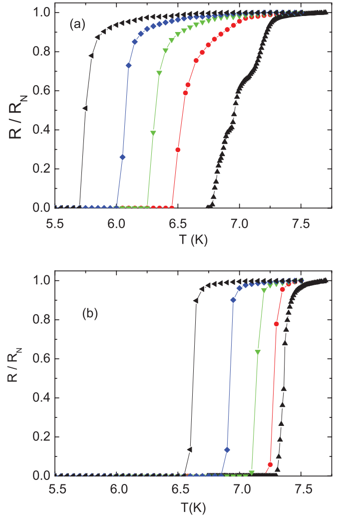
FIG. 12. (Color online) Resistance R vs temperature T for two different sets of multilayers consisting of building blocks \text{Cu}_{0.41}\text{Ni}_{0.59} (3 nm)/Nb(30 nm), and in different applied magnetic fields; from right to left: (0, 0.25, 0.5, 0.75, 1) T. (a) is an asymmetric set of type F/[9(S/F)]; (b) is a symmetric set where the outer F layers have half the thickness of the inner ones.
