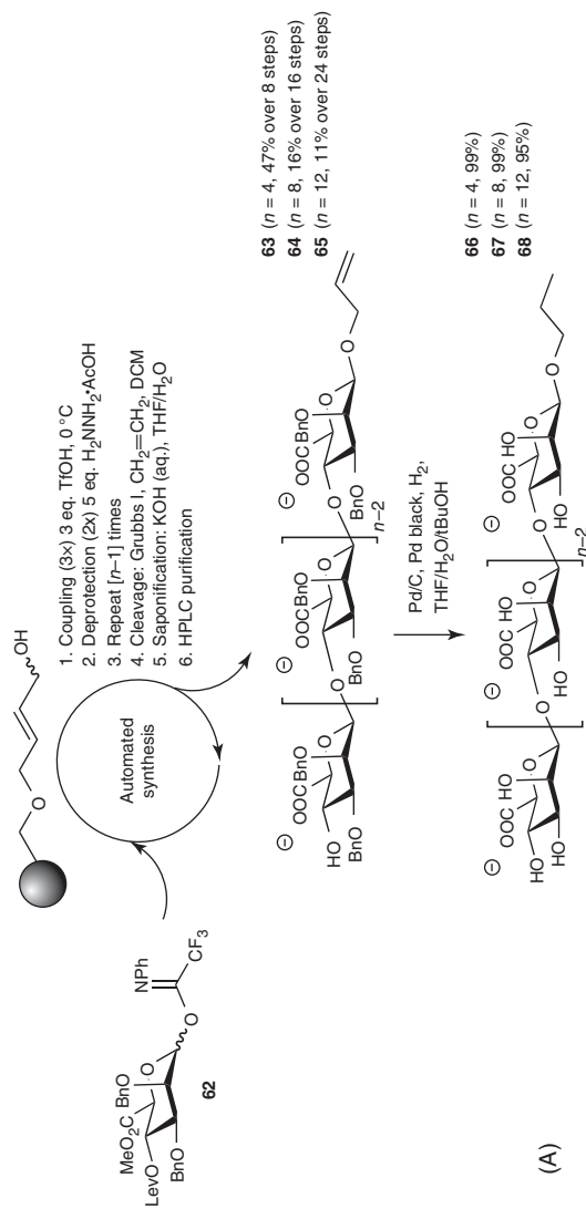
Scheme 1.11 Automated synthesis of oligomannuronic acids. (A) Solid-phase approach. (B) Fluorous-phase approach.
