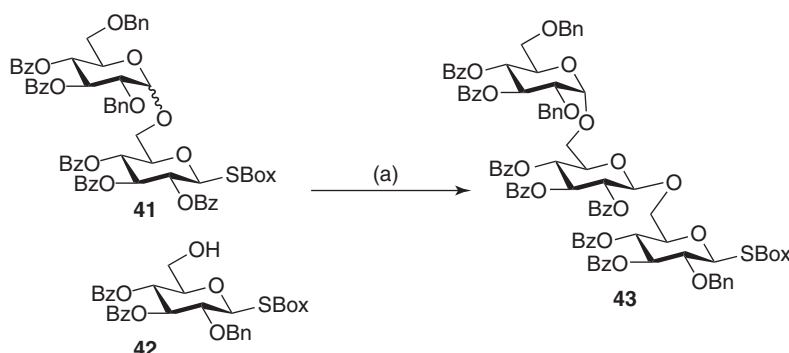
Scheme 1.8 Neighboring group participation-assisted selective activation: (a) \text{Cu}(\text{OTf})_2 , \text{TfOH} , and DCM (70%).
