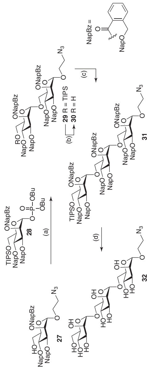
Scheme 1.6 Global deprotection using TFA in toluene: (a) TMSOTf and DCM, -20°C (97%); (b) HF/pyridine and pyridine (91%); (c) 28 , TMSOTf, and DCM, -20°C (94%); (d) TFA/toluene (10 : 1, v/v), 0°C to RT (100%).
