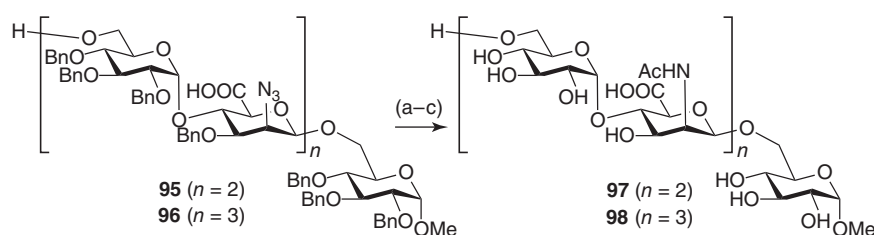
Scheme 1.15 Birch reduction of teichuronic acid oligosaccharides in which cleavage of the mannosaminuronic acid linkages was encountered; (a) Na (s), liquid \text{NH}_3 , and THF, -60^\circ\text{C} ; (b) HPLC purification; (c) \text{Ac}_2\text{O} , \text{NaHCO}_3 , and THF/ \text{H}_2\text{O} ( 97 : 35% over 2 steps; 98 : 14% over 2 steps).
