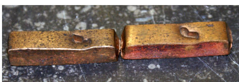
Figure A5.5 Raw matrices that look like the strikes were made in pre-cut copper bars.
