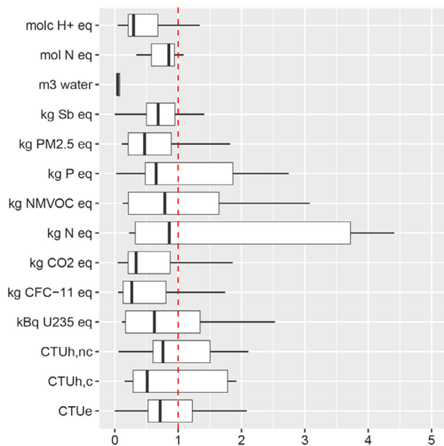
Figure 4. Relative LCA impact scores compared with a reference single-Si PV rooftop system as modeled in ecoinvent v3.4 [27] (single-Si impact score = 1, indicated by the red dotted line).
