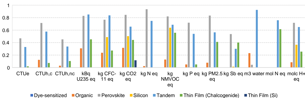
Figure 7. Average relative contributions of PV cells as compared with the corresponding PV system.
