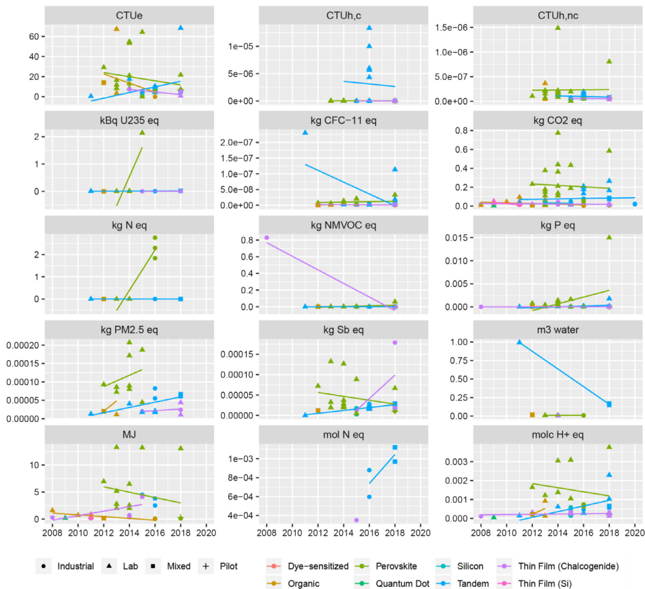
Figure 3. Harmonized LCA impact scores of PV technologies as a function of time. CTUe, freshwater ecotoxicity; CTUh,c, human toxicity—cancer effects; CTUh,nc, human toxicity—noncancer effects; kg CFC-11 eq, ozone depletion; kg CO 2 eq, climate change; kg N eq, marine eutrophication; kg NMVOC eq, photochemical oxidation; kg P eq, freshwater eutrophication; kg PM 2.5 eq, particulate matter; kg Sb eq, mineral resource depletion; kg U235 eq, ionising radiation; m 3 water, water use; MJ, cumulative energy demand; mol H + eq, acidification; and mol N eq, terrestrial eutrophication.
