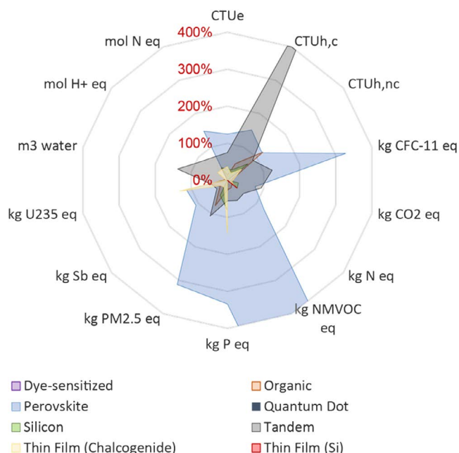
Figure 8. Relative ILCD impact scores for different PV technologies, compared with a reference single-Si roof-mounted PV system as modeled in ecoinvent v3.4 (=100%). The plot is truncated at 400% for visualization purposes.
