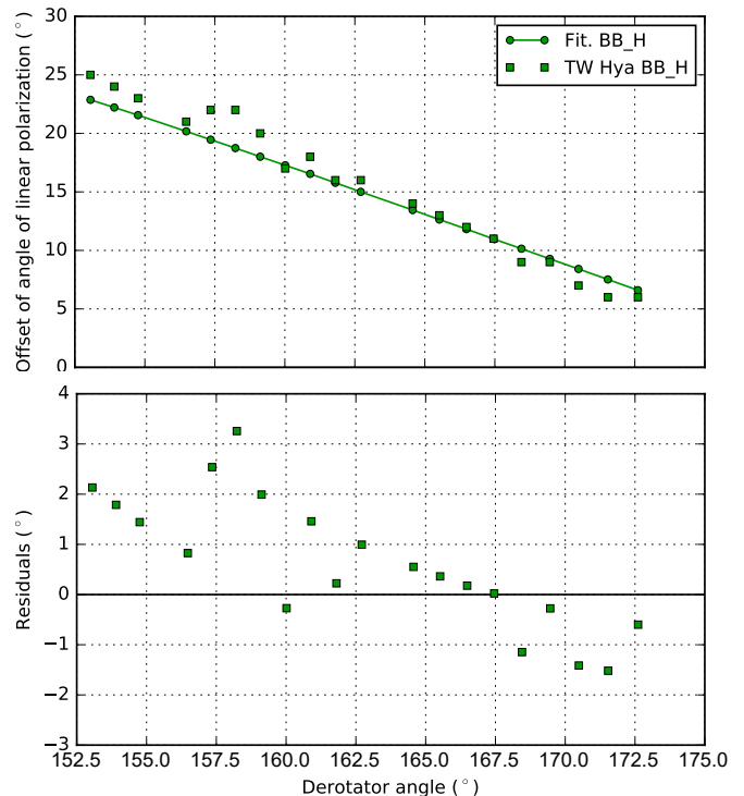
Fig. 6. Top: Expected polarization angle offsets of the same model (solid line) as used in Fig. 5; and the polarization angle offset angles ( \phi_0 of Eq. 17) of TW Hydrae (squares) with respect to azimuthal polarization. Bottom: Residuals between the model polarization angle offsets and \phi_0 retrieved for TW Hydrae.
