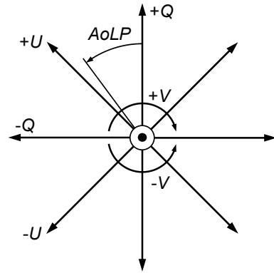
Fig. 1. Orientation of the Stokes vector components of Eq. 1, where the beam is propagating out of the paper towards the reader. After the vertical axis ( +Q ) is aligned with a preferred orientation (usually the meridian on-sky), the remaining Stokes vector components are oriented accordingly. The Angle of Linear Polarization ( AoLP , Eq. 4) is also measured with respect to the +Q direction in counter-clockwise direction.
