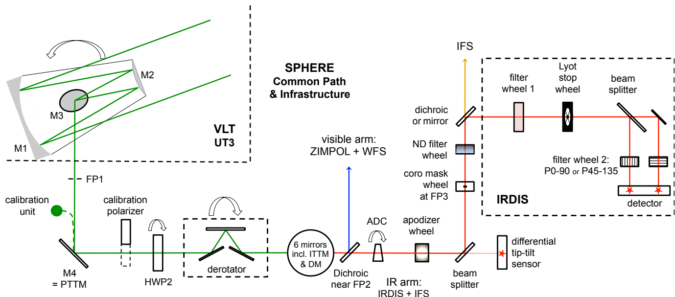
Fig. 2. Schematic overview of the telescope and SPHERE/IRDIS, showing the optical components that are relevant for the polarimetric imaging mode. The curved arrows indicate components that rotate during an observation block. Reflections at angles of incidence \geq 45^\circ in the instrument are represented with similarly large incidence reflections in the figure. The green beam shows the starlight before color filters are applied, blue represents visible light, red and orange represent NIR light (with the orange beam towards the IFS showing the shorter wavelengths).
