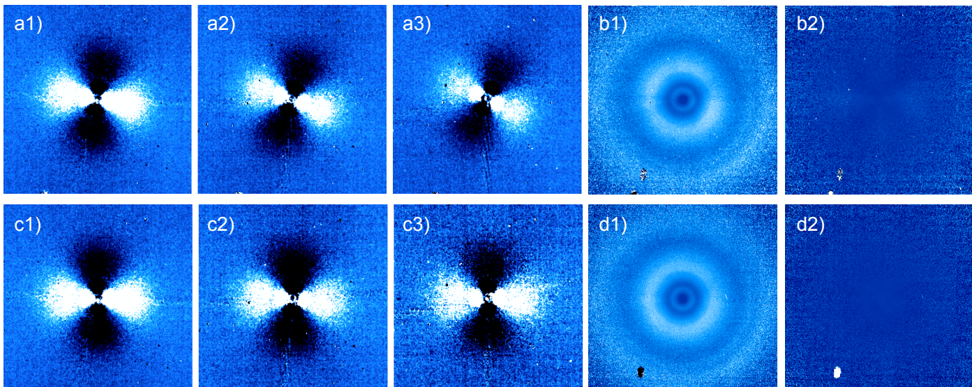
Fig. 8. a1, a2, & a3 ) Q_{\text{IPS}} images of three HWP cycles with \theta_{\text{der}} = 169.7^\circ, 162.0^\circ, and 154.1^\circ , respectively. These images are created with the U_\phi minimization method (Sect. 6.1). We can clearly see the butterfly patterns rotate in clockwise direction and the signal decrease from left to right. b) When we use the assumption of azimuthal polarization, we can find the correct \phi_0 for each HWP cycle and compute the final r^2 -scaled Q_\phi ( b1 ) and U_\phi ( b2 ) images (Sect. 6.1). Because we have used the assumption that we know the Angle of Linear Polarization at each point, we cannot claim to have determined the AoLP in this image. c) When we apply the correction method to the Q and U images, we retrieve the best approximation of the incident Q and U images (Sect. 6.2). The displayed Q images (for the same \theta_{\text{der}} as panel a) contain the ideal orientation of the butterflies and are corrected for the reduced polarimetric efficiency. However, the latter does not improve the signal to noise (illustrated by the increased noise in panel c3). d1 & d2) The IRDAP-corrected Q_\phi and U_\phi image. Because we no longer need the assumption that we know the AoLP a priori, we can use Q and U after the correction method to determine the AoLP in our final reduction.
