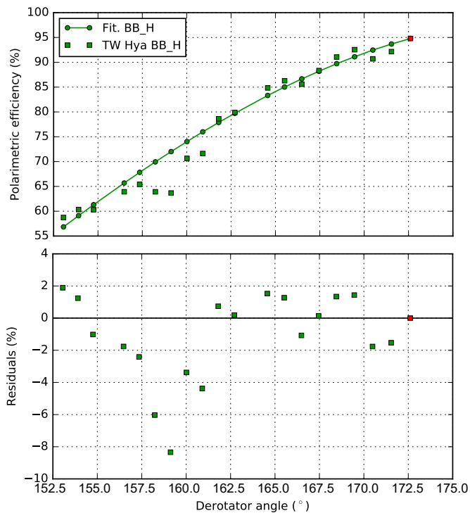
Fig. 5. Top: Polarimetric efficiency modeled (solid line) for the same derotator and HWP2 angles as used during the observation of TW Hydrae (squares). Note that the polarimetric efficiencies measured for the HWP cycles of TW Hydrae are only determined relative to the other HWP cycles. We therefore scaled all data points such that the first cycle (red square, with the highest polarimetric efficiency) matches the value of the model. Bottom: Residuals between the model and the polarimetric efficiencies obtained for TW Hydrae.
