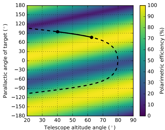
Fig. 9. The polarimetric efficiency in H band as a function of the parallactic angle and altitude angle, when the derotator is in field-tracking mode without an additional derotator offset. The dashed line shows the parallactic and altitude angle of TW Hydrae across the sky, with the solid line showing the angles during the SPHERE observation. We clearly see that using default derotator settings (North up on the detector) will give us mediocre polarimetric efficiencies.
