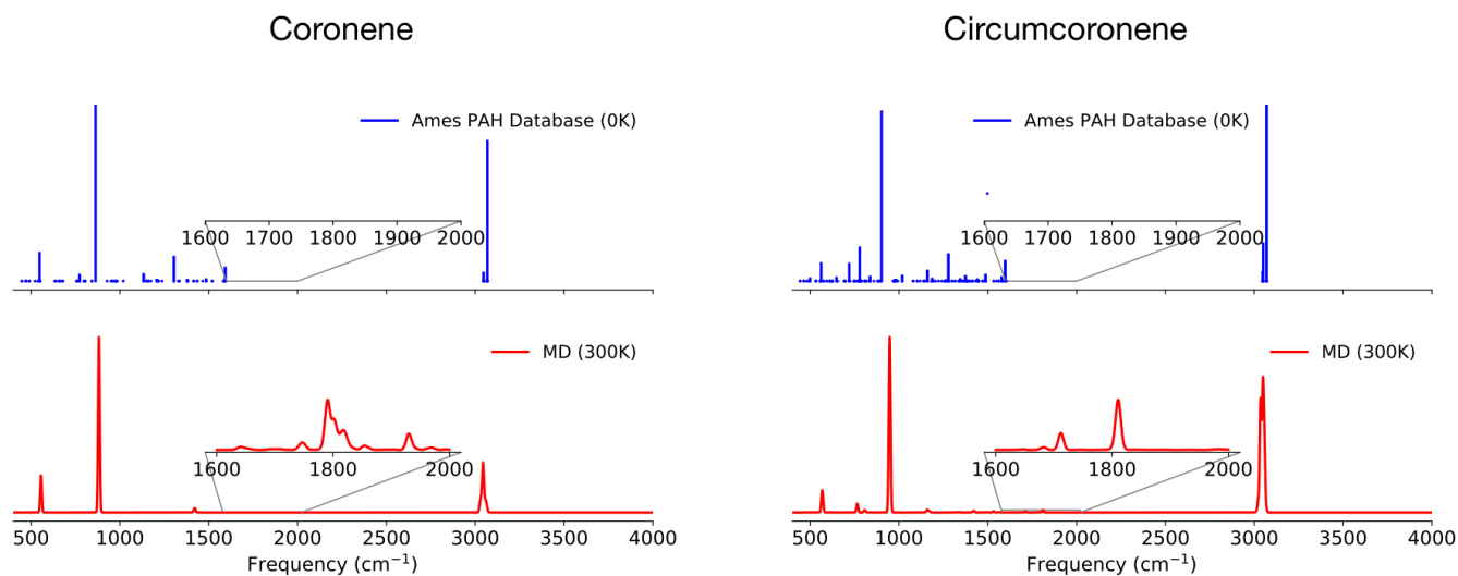
Fig. 3. Comparison between harmonic ( top panels ) and anharmonic ( bottom panels ) IR spectra of coronene ( left panels ) and circumcoronene ( right panels ). The harmonic spectra are downloaded from NASA Ames PAH Database, and multiple scaling factors are multiplied to correct the anharmonic effects (Bauschlicher et al. 2018). The anharmonic spectra are calculated at 300 K with semiempirical method of PM3. The insets show the region of combination bands, where anharmonicity and resonances dominate.
