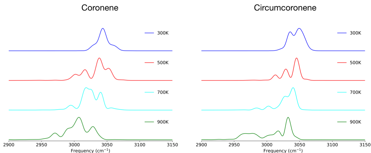
Fig. 4. C-H stretching region of the calculated anharmonic spectra of coronene and circumcoronene at 300 K, 500 K, 700 K, and 900 K.
