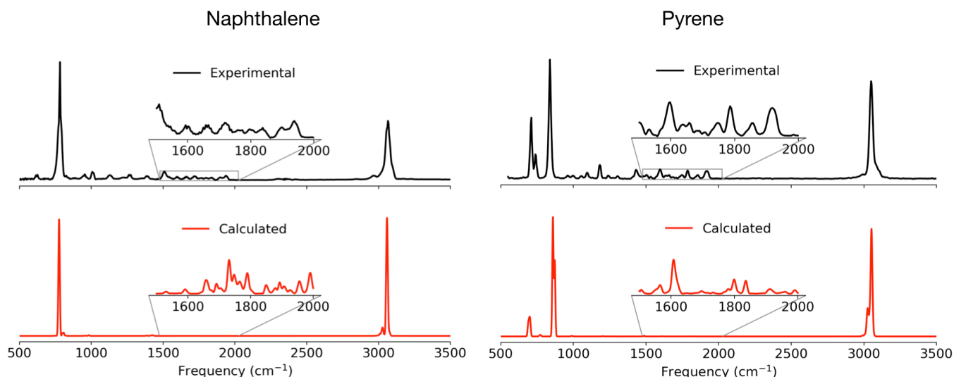
Fig. 2. Experimental and calculated gas-phase IR spectra of naphthalene and pyrene at 300 K. The top black curves represent the experimental spectra. The bottom red curves are calculated spectra using semiempirical method of PM3. The insets zoom in the region (1500–2000 \text{cm}^{-1} ) where combination bands dominate.
