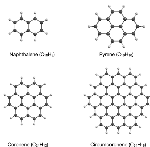
Fig. 1. Structures of molecules studied in this work. Naphthalene and pyrene belong to point group D 2h . Coronene and circumcoronene possess highly symmetric structure with point group D 6h .
