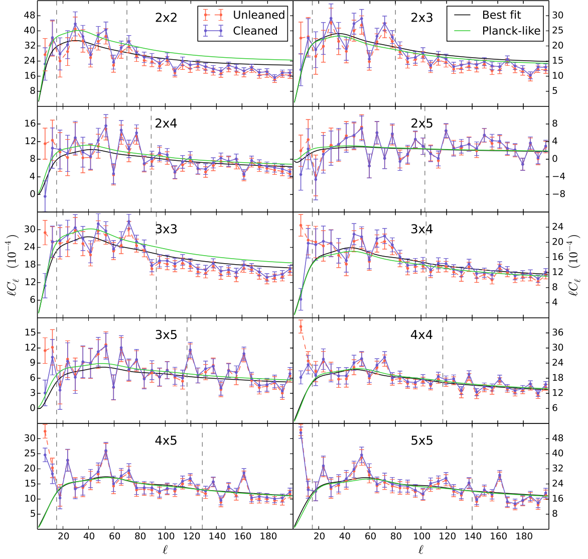
Figure 19. Similar as Fig. 16, but for data restricted to the northern Galactic hemisphere. The cleaning process reduces power at \ell < 9 and re-scales the C_\ell s. The best-fit C_\ell s to the northern data present slopes that are compatible with Planck.
