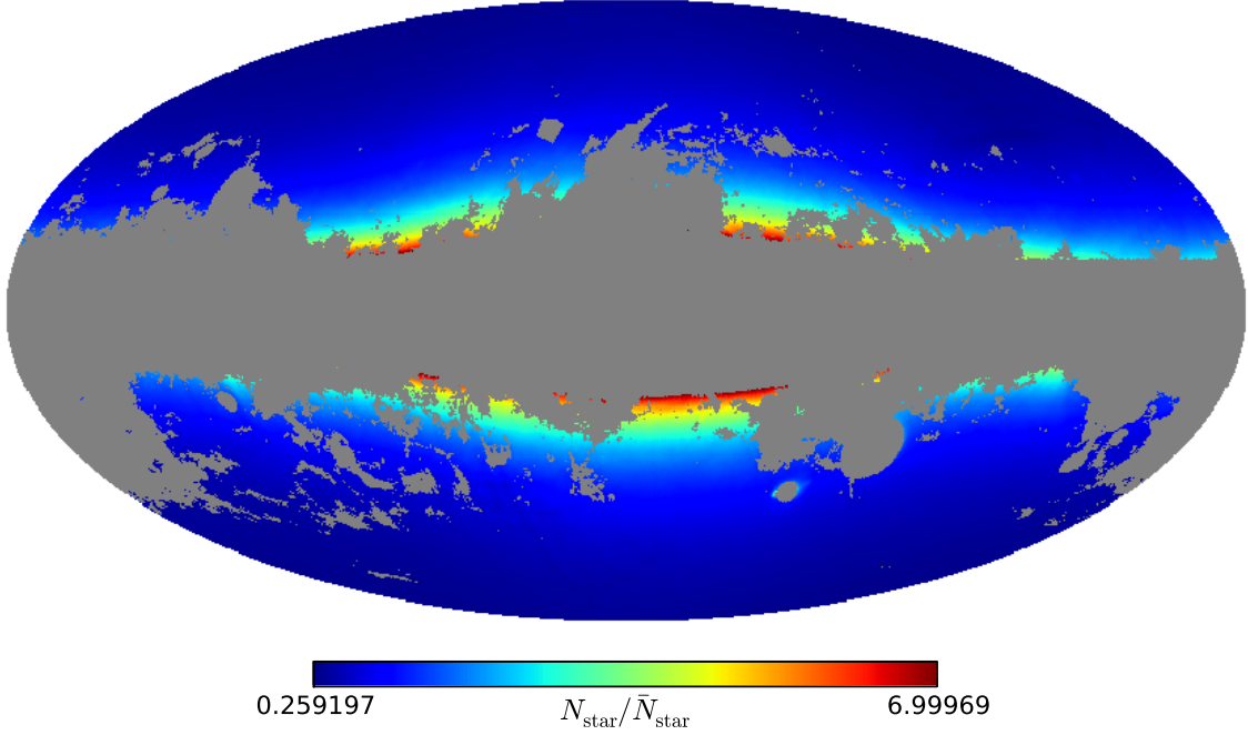
Figure 8. Stellar density template, derived from Gaia DR2 sources selected as described in Sec. 2.3, used to estimate contamination and obscuration in WSC projected galaxy distribution.
