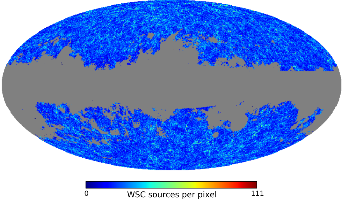
Figure 1. Sky map of number counts of WSC sources (mostly galaxies) in the photo- z range 0.10 < z < 0.35 in Galactic coordinates, after applying all the cuts described in Sec. 2, using Healpix [55] resolution parameter N_{\text{side}} = 256 . The gray regions were masked out.
