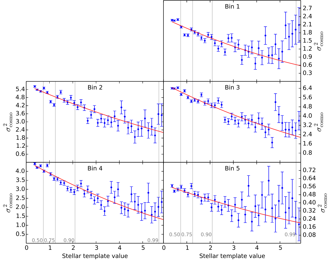
Figure 9. Variance attributed to cosmological fluctuations \sigma_{\text{cosmo}}^2 as a function of the stellar density template value S(s) (Fig. 8), for each redshift bin. The blue data points show the values measured from data, and the red curve is the obscuration model fit (Eq. 3.7). The vertical gray lines with labels show the survey area fraction with a smaller S(s) .
