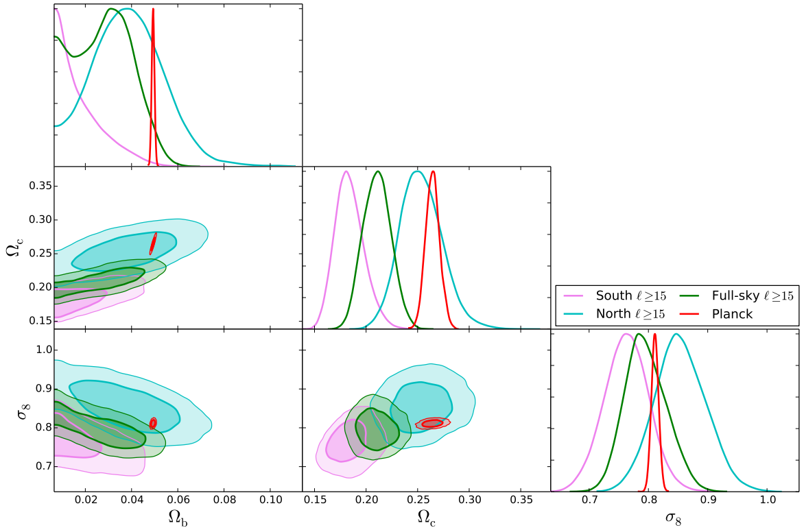
Figure 20. Similar as Fig. 17, but all WSC posteriors employ scales \ell \geq 15 and use cleaned data. The cyan and pink posteriors were obtained from the northern and southern hemispheres, respectively, while the green posteriors show the results for the full sky.
