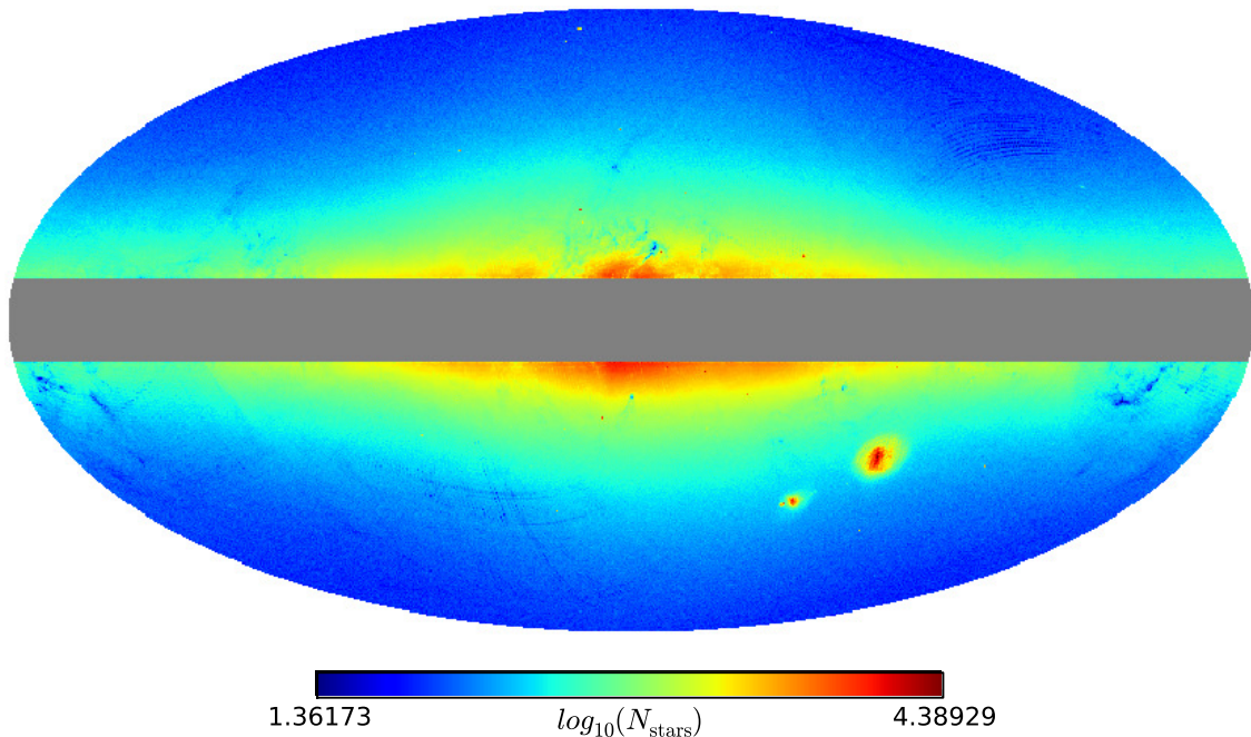
Figure 3. Sky map of number counts (sources per pixel, using N_{\text{side}} = 256 , in logarithmic scale) at Galactic latitudes |b| > 10^\circ of Gaia DR2 sources at G < 20 magnitude limit, after removing those with both parallax and proper motion measurements consistent with zero.
