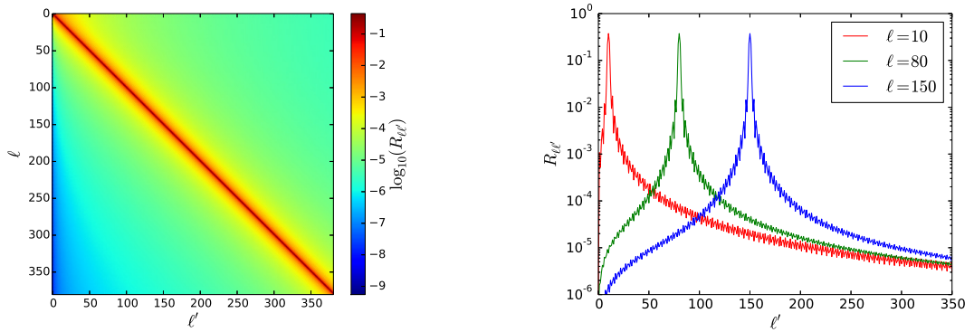
Figure 11. Left panel: a color plot of the logarithm of the mixing matrix R_{\ell\ell'} computed for our WSC mask, up to \ell = 380 . Right panel: plot of R_{\ell\ell'} for \ell fixed at 10 (red), 80 (green) and 150 (blue).
