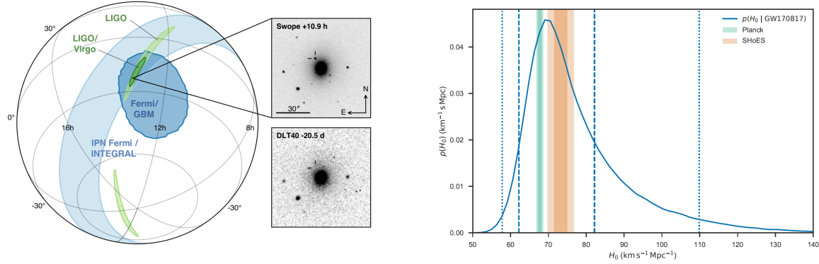
Figure 7. Left panel: The multi-messenger sky localization of GW170817 and the identification of the host galaxy. Right panel: The posterior distribution of H_0 compared to the recent CMB and SNIa constraints [653, 654]. Figures taken from Refs. [22, 24].
