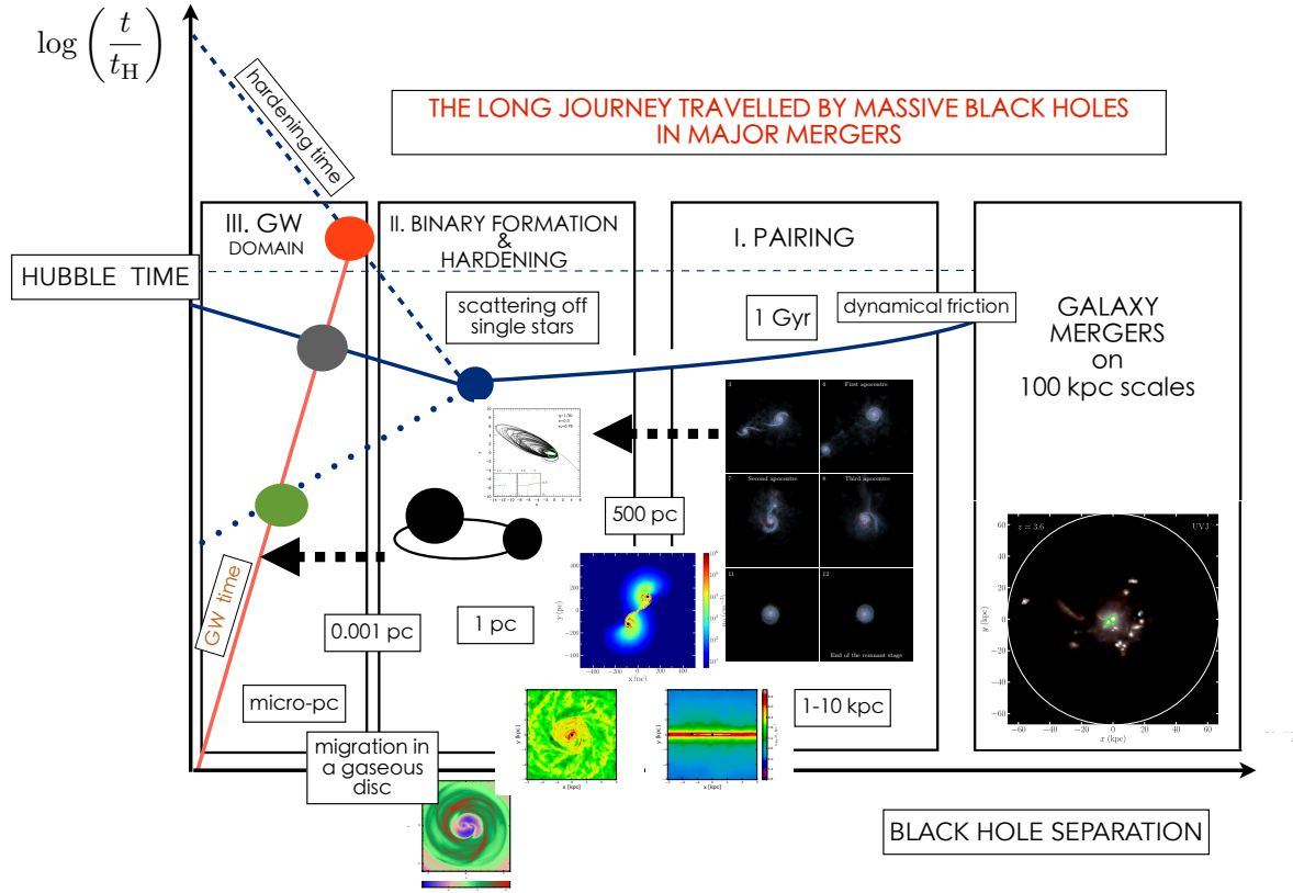
Figure 5. Cartoon illustrating the journey travelled by SMBHs of masses in the range 10^6\text{--}8\ M_\odot during major galaxy-galaxy collisions. The x -axis informs on the SMBH separation given in various panels, while the y -axis informs on the timescale. The journey starts when two galaxies (embedded in their DM halos) collide on kpc scales (right-most plot). The inset shows a selected group of galaxies from the cosmological simulation described in Ref. [340]. The inset in the second panel (from right to left), from Ref. [341], depicts the merger of two disc galaxies and their embedded SMBHs. Pairing occurs when the two SMBHs are in the midst of the new galaxy that has formed, at separations of a few kpc. The SMBHs sink under the action of star-gas-dynamical friction. In this phase, SMBHs may find themselves embedded in star-forming nuclear discs, so that their dynamics can be altered by the presence of massive gas-clouds. Scattering off the clouds makes the SMBH orbit stochastic, potentially broadening the distribution of sinking times during the pairing phase [342–345]. Furthermore, feedback from supernovae and AGN triggering by one or both the SMBHs affect the dynamics as these processes alter the thermodynamics of the gas and its density distribution, which in turn affect the process of gas-dynamical friction on the massive BHs. It is expected that eventually the SMBHs form a Keplerian binary, on pc scales. Then, individual scattering off stars hardens the binary down to the GW-driven domain. This is an efficient mechanism (and not a bottleneck) if the relic galaxy displays some degree of triaxiality and/or rotation. In this case, there exists a large enough number of stars on low-angular momentum orbits capable to interact with the binary and extract orbital energy [346]. The binary in this phase can also be surrounded by a (massive) circum-binary disc [347]. In a process reminiscent to type II planet migration, the two SMBHs can continue to decrease their separation and they eventually cross the GW boundary. Then, GW radiation controls the orbital decay down to coalescence.
