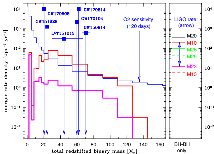
Figure 2. Left: Redshifted total merger mass distribution for two population synthesis models [124]: M10 (low BH natal kicks) and M23 (high BH natal kicks). The O2 LIGO sensitivity is marked; the most likely detections are expected when models are closest to the sensitivity curve. We also mark LIGO/Virgo BBH merger detections (vertical positions have no meaning), all of which fall within the most likely detection region between 20 – 100 M ⊙ . Right: Source frame BBH merger-rate density of several population synthesis models for the local Universe ( z = 0 ). The current LIGO O1/O2 BBH merger rate is 12–213 Gpc -3 yr -1 (blue double-headed arrow). Note that the models with fallback-attenuated BH natal kicks (M10, M20) are at the LIGO upper limit, while models with high BH natal kicks are at the LIGO lower limit (M13, M23). Models with small (M26) and intermediate (M25) BH kicks fall near the middle of the LIGO estimate.
