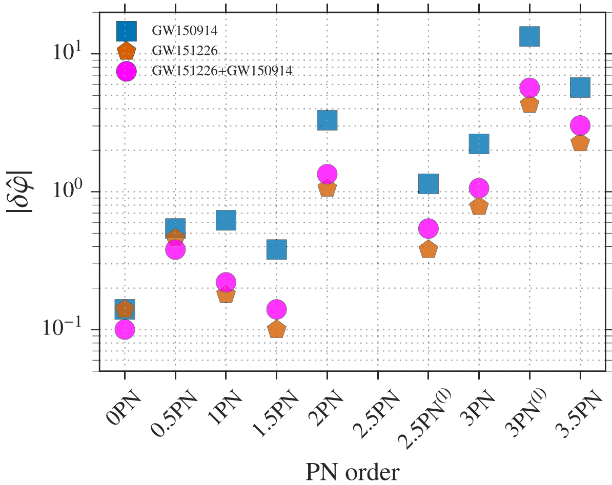
Figure 9. Two GW detections of inspiralling BH binaries were used to set bounds on possible deviations from their GR values of various PN coefficients that appear in the expression for the GW phase. Figure from Ref. [3].
