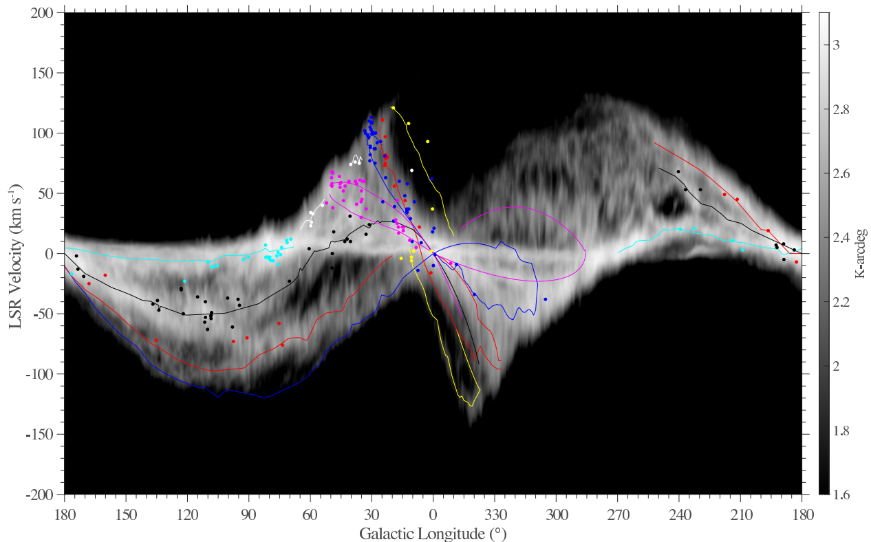
Fig. 3.— H I emission in grey scale as a function of v_{\text{LSR}} and Galactic longitude. Colored dots are sources with parallax measurements shown in Fig 1 and the colored lines trace the spiral arms updated from Reid et al. (2016) and discussed in Section 3.2. Note, we have connected the somewhat irregular (l, v) locations of giant molecular clouds seen in CO or H I emission, giving the slightly jagged spiral arm traces.
