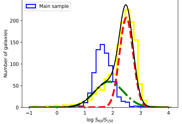
Fig. 3. The 60\text{-}\mu\text{m} - 150\text{-MHz} colour distribution of all matches within 3' between the RIFSCz sources (which only have IRAS observations) and LOFAR sources (yellow histogram). The dot-dashed Gaussian represents the inferred colour distribution of the true counterparts and the dashed Gaussian represents that of the random associations. The black solid line is the sum of the two. The colour distribution of the main sample is shown as the blue histogram.
