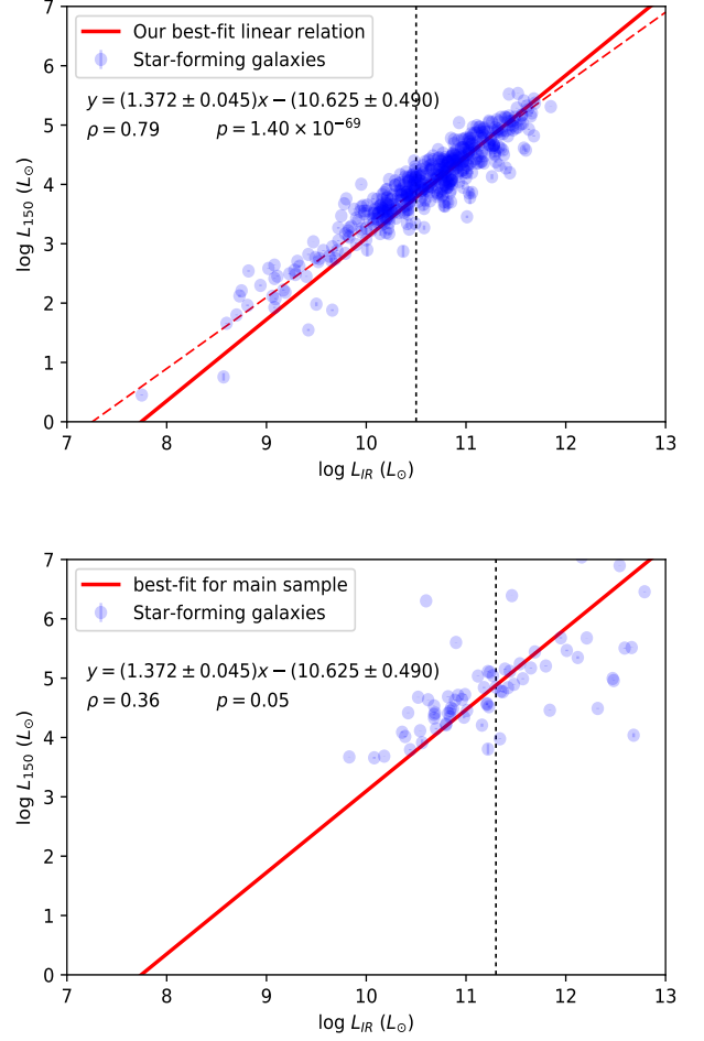
Fig. 10. Top: The correlation between the IR luminosity and the 150-MHz luminosity for the main sample, after excluding AGNs. The vertical dashed line indicates the 90% completeness limit at the median redshift ( z \sim 0.05 ) of the main sample. Bottom: Same as the top panel but for the second sample. The vertical dashed line indicates the 90% completeness limit at the median redshift ( z \sim 0.12 ) of the second sample.
