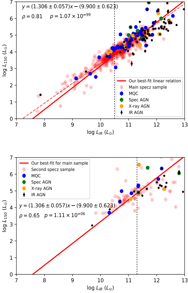
Fig. 9. Top: The correlation between the IR luminosity and the rest-frame 150-MHz luminosity for the main spec-z sample, including AGNs identified in the X-ray, IR, the Million Quasar Catalog and in optical spectroscopy. The vertical dashed line indicates the 90% completeness limit at the median redshift ( z \sim 0.05 ) of the main sample. Bottom: Same as the top panel but for the second sample. The vertical dashed line indicates the 90% completeness limit at the median redshift ( z \sim 0.12 ) of the second sample.
