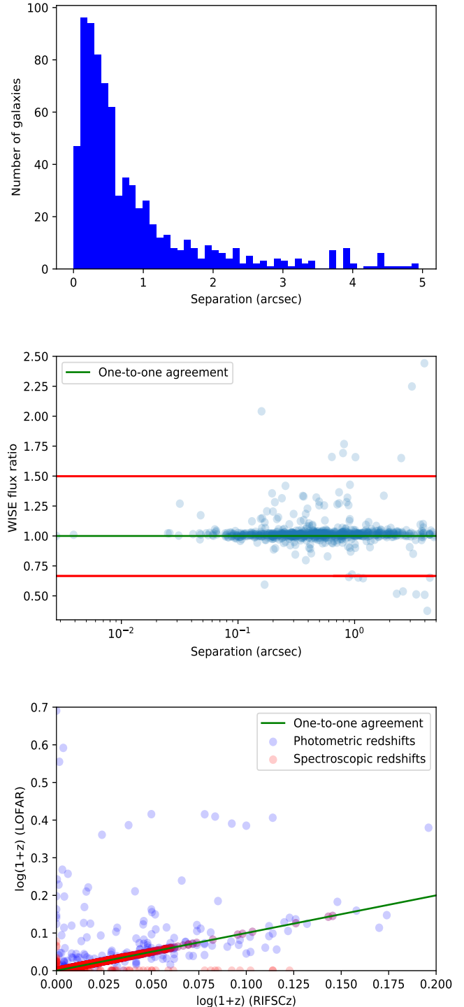
Fig. 1. Top: The distribution of positional separations of sources matched between RIFSCz and LOFAR. Middle: Comparison of WISE W1 flux for sources listed in RIFSCz and in LOFAR. Sources inside the two horizontal red lines have good WISE flux agreement (i.e., the difference is within a factor of 1.5). Bottom: Comparison of redshifts compiled in the RIFSCz and LOFAR VAC.
