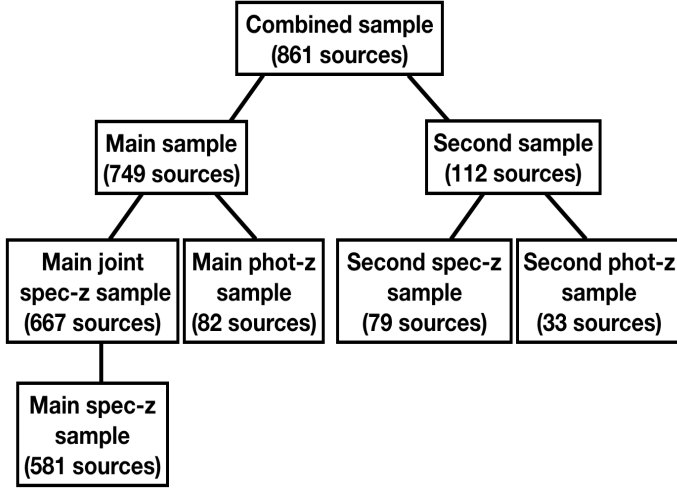
Fig. 4. A schematic view of our RIFSCz-LOFAR matched sample.
