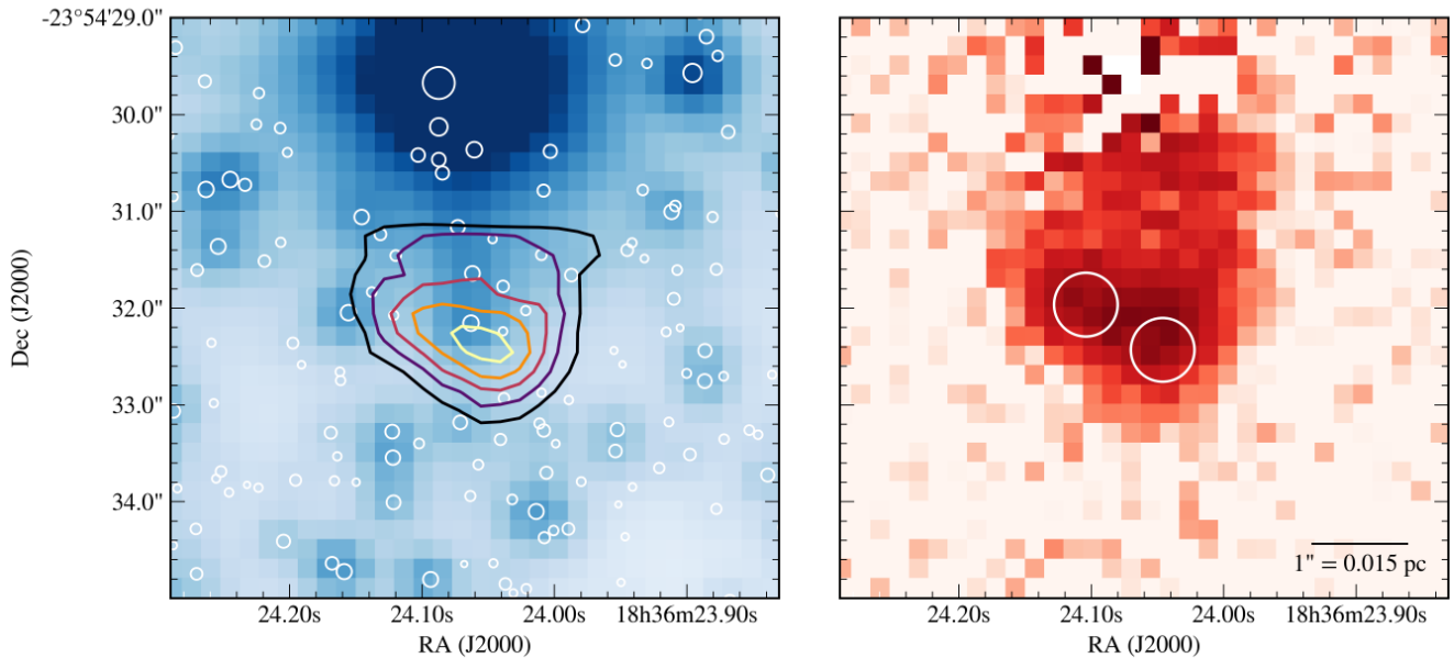
Fig. 1. MUSE whitelight detail image of the region in NGC 6656 containing the nebula created from a single observation (left). Contours give the combined [\text{N II}]\lambda 6583 emission flux after subtracting the stellar background (see Section 3.1). White circles represent HST sources from the catalogue of Nardiello et al. (2018), the diameter scales with F606W magnitude. The median flux in the four layers containing the [\text{N II}]\lambda 6583 emission line is shown after the median flux in three adjacent layers was subtracted (right). The two apertures used to extract the spectrum of the nebula are shown as white circles.
