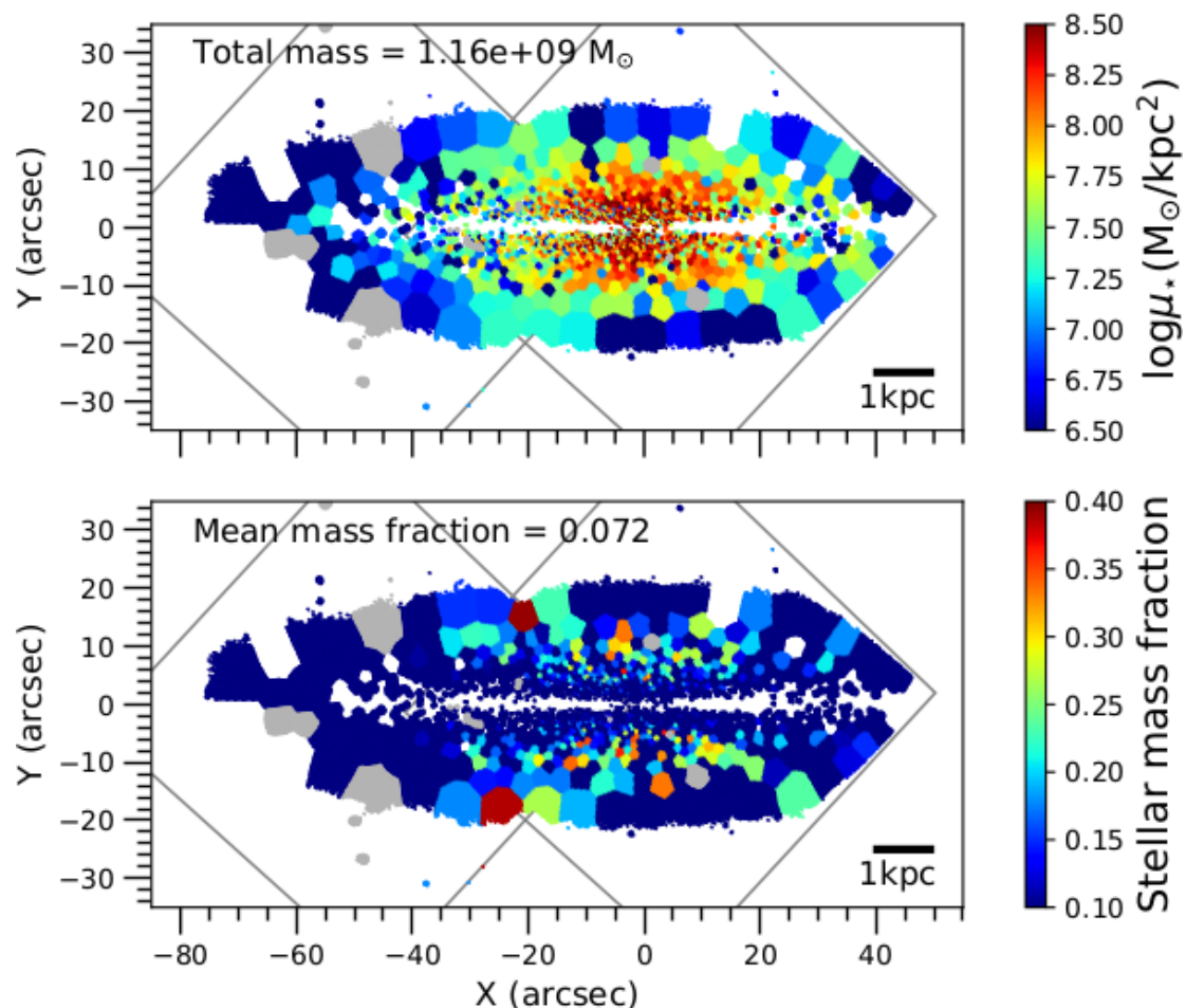
Fig. 13. Distribution in FCC 153 of the stellar population with ages between 6 and 11 Gyr, metallicities between -0.6 and -0.35 dex and [\text{Mg}/\text{Fe}] \sim 0.4 dex. The color scale shows the stellar mass density in the top panel and the stellar mass fraction in the bottom panel. The total mass or the mean mass fraction in this specific population are indicated on top-left of respectively the top and the bottom maps. In each panel, the coverage of the two MUSE pointings and the discarded bins are plotted in grey. A scale bar on bottom-right indicates the correspondence with physical units.
