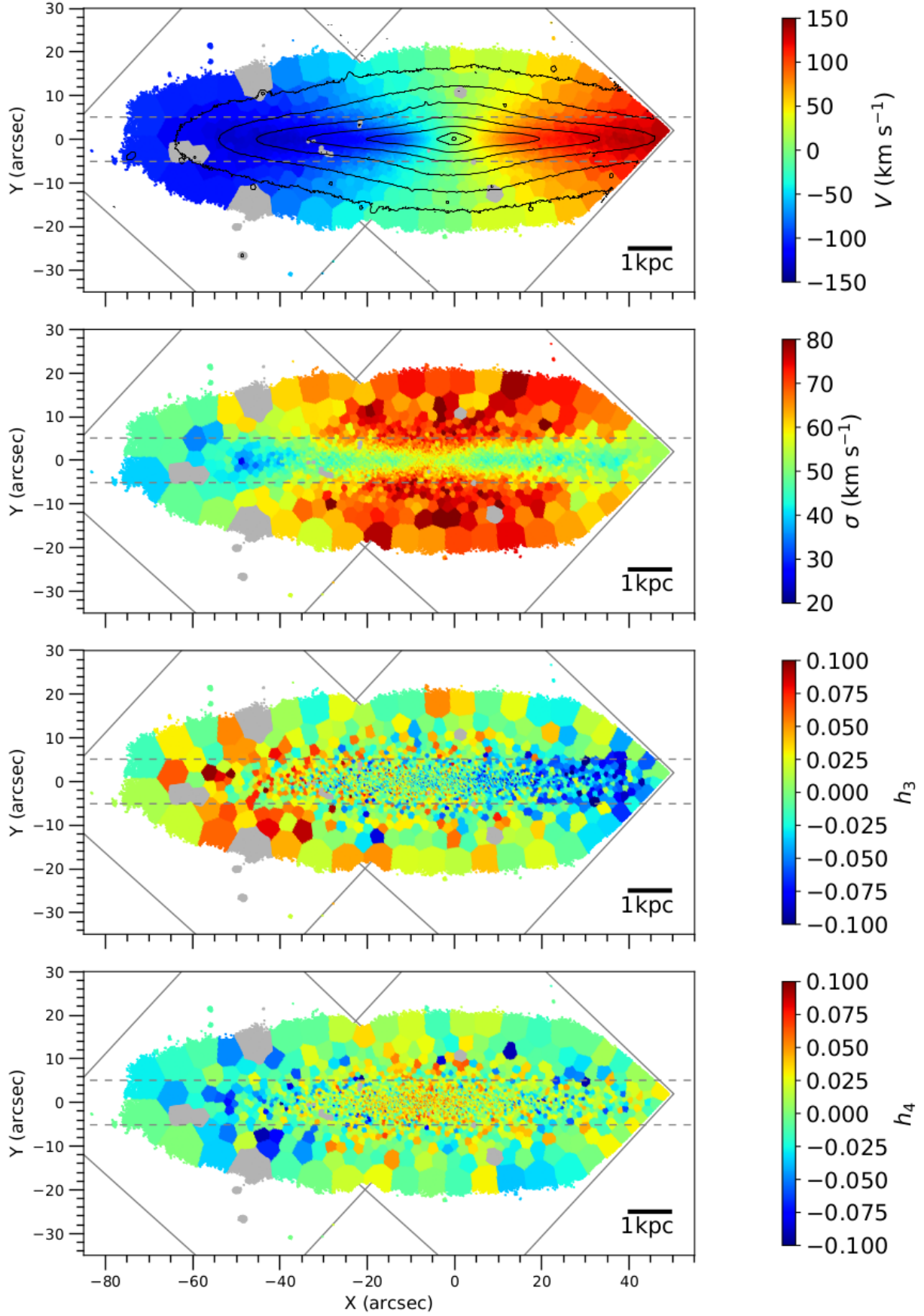
Fig. 2. Maps of the stellar kinematics of FCC 153. From top to bottom: mean velocity V , velocity dispersion \sigma , skewness h_3 and kurtosis h_4 . The discarded bins are plotted in grey, as well as the coverage of the two MUSE pointings. The physical units are indicated by the scale bar on bottom-right of each panel. The horizontal dashed lines indicate \pm z_{c1} . In the top panel, contours of surface brightness are plotted in black.
