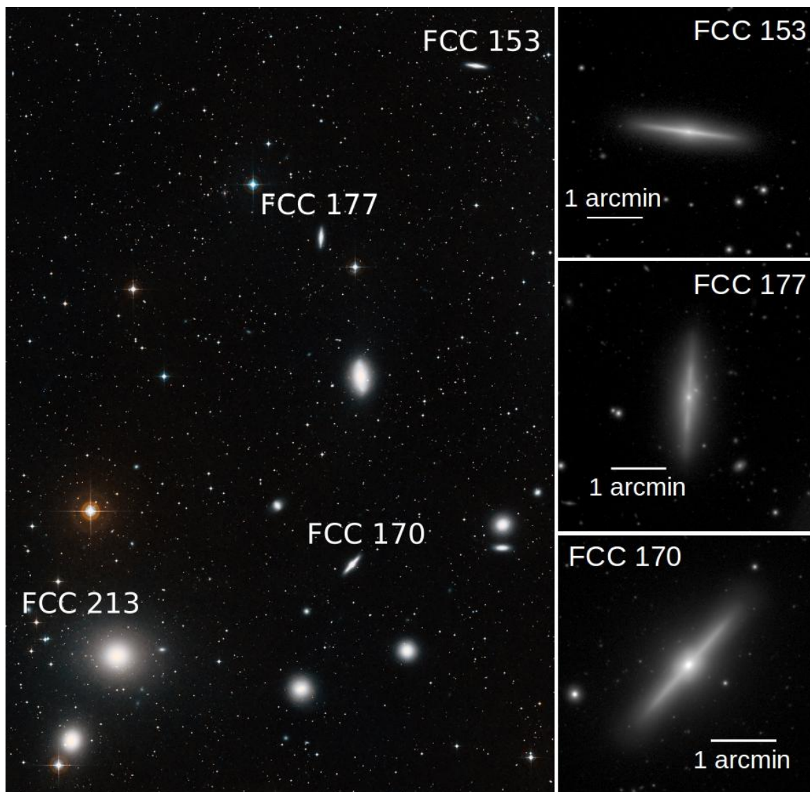
Fig. 1. Left: clipping of the wide-field view of the Fornax Galaxy Cluster (credit: ESO and Digitized Sky Survey 2, acknowledgment: Davide De Martin). The three galaxies analyzed in Paper I and this paper are indicated with their names. FCC 213 is the central galaxy of the cluster. Right: r -band images from the Fornax Deep Survey (Iodice et al. 2019). From top to bottom: FCC 153, FCC 177 and FCC 170. A scale bar is indicated in each image.
