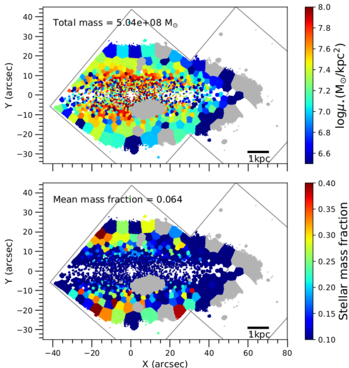
Fig. 14. As Fig. 13, now for FCC 177.
