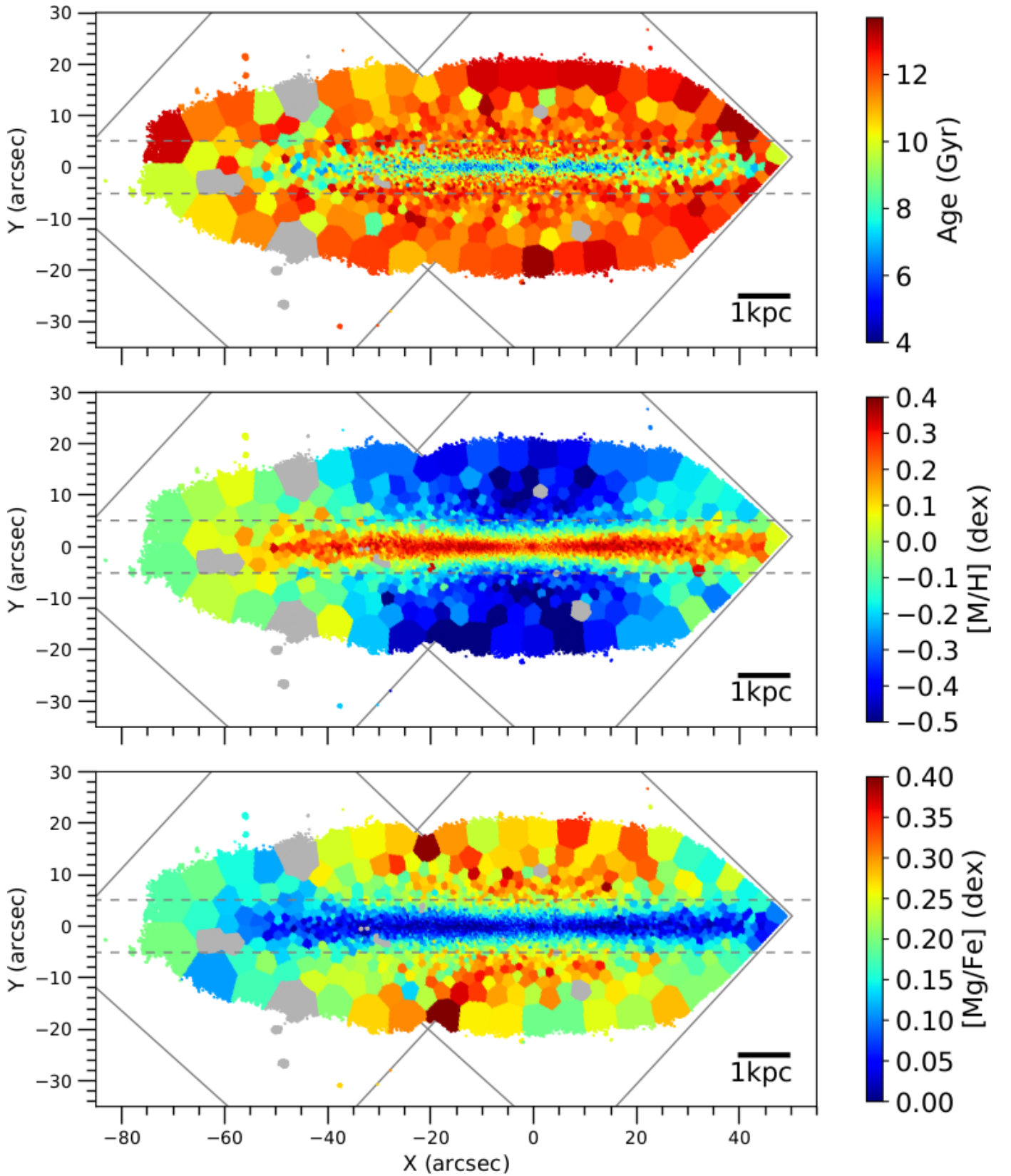
Fig. 4. Stellar-population maps for FCC 153. From top to bottom: mean age, total metallicity [M/H] , [Mg/Fe] abundance. The discarded bins are plotted in grey, as well as the coverage of the two MUSE pointings. The physical units are indicated by the scale bar on bottom-right of each panel. The horizontal dashed lines indicate \pm z_{c1} .
