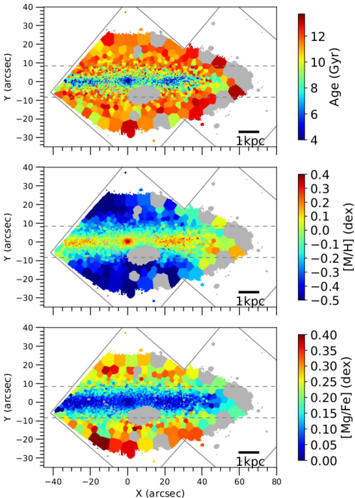
Fig. 5. As Fig. 4, now for FCC 177.
