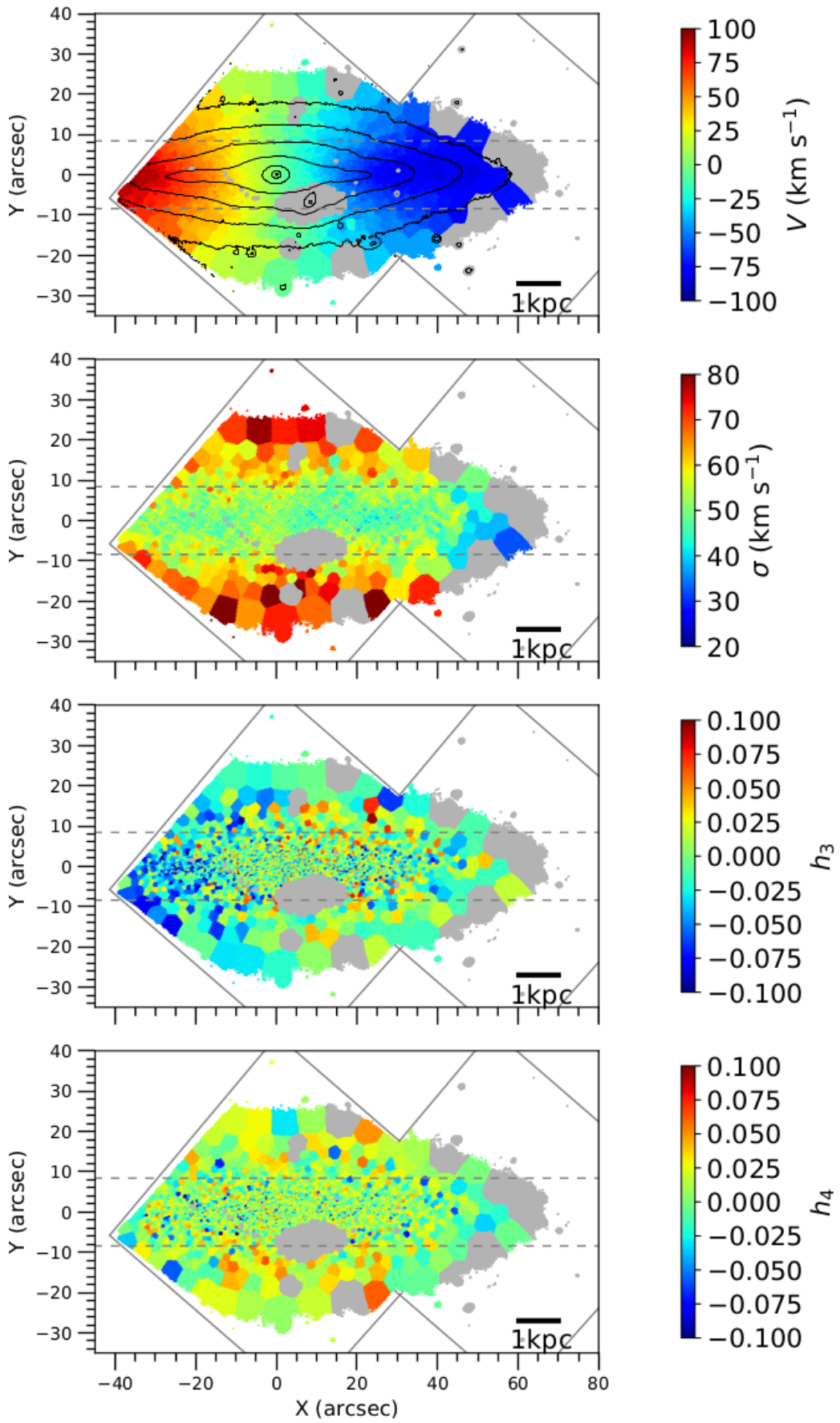
Fig. 3. As Fig. 2, now for FCC 177.
