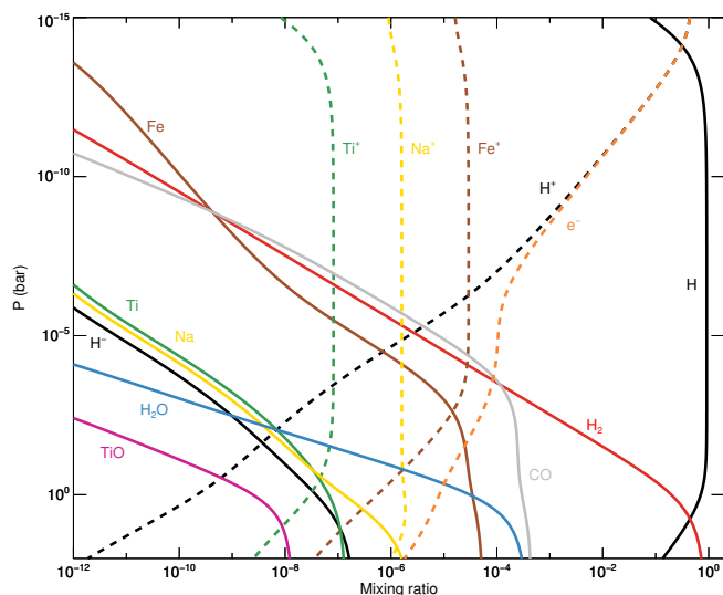
Fig. 3. Abundance profiles modeled with FastChem for a selection of neutral atoms (solid lines) and ions (dashed lines), as well as molecules, \text{H}^- and electrons. The model assumes an isothermal structure at 4,000 K and solar metallicity. Over most of the modeled pressure region, molecules tend to be dissociated and metals tend to be singly ionized. The decrease of ion abundances towards higher altitudes (pressures below \sim 10^{-12} bars) indicates the emergence of doubly ionized species at low pressures. The effects of photo-ionization are not included, as these are predicted to be small in the denser parts of the atmosphere (Kitzmann et al. 2018).
