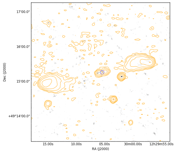
A.1. 17 ILTJ123005.72+491516.8 ROBUST: -0.5
