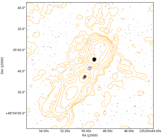
A.1. 27 ILTJ132049.67+480445.6 ROBUST: -\mathbf{0.5}
