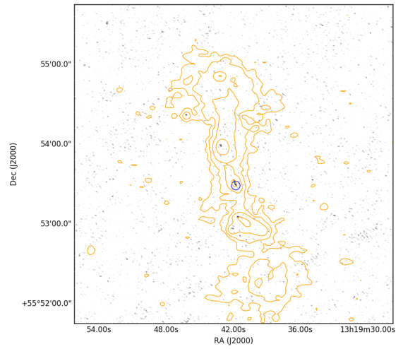
A.1. 26 ILTJ131941.97+555345.3 ROBUST: -\mathbf{0.5}
