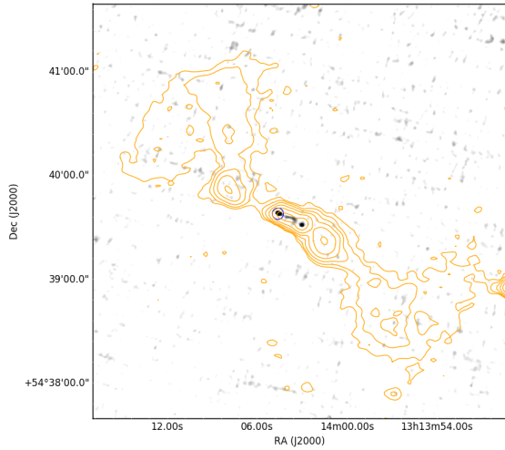
A.1. 25 ILTJ131403.17+543939.6 ROBUST: -\mathbf{0.5}
