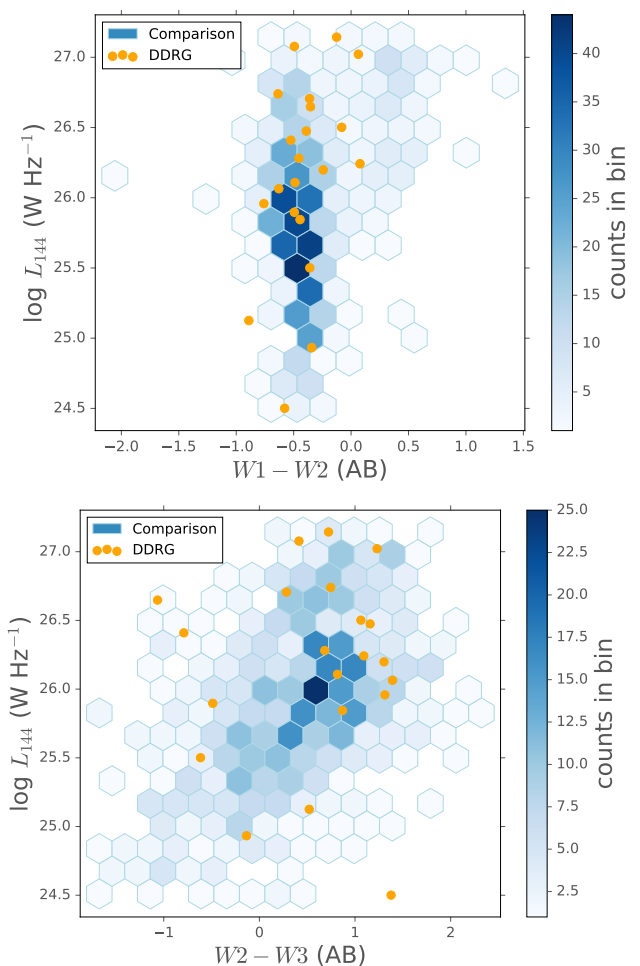
Fig. 7: Luminosity distribution of RLAGN (blue density hexagons) and DDRGs (orange points) with W1 - W2 (top) and W2 - W3 (bottom).
