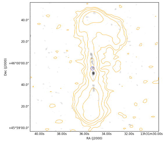
A.1. 28 ILTJ133135.09+455957.0 (removed from sample) ROBUST: \mathbf{0.5}
