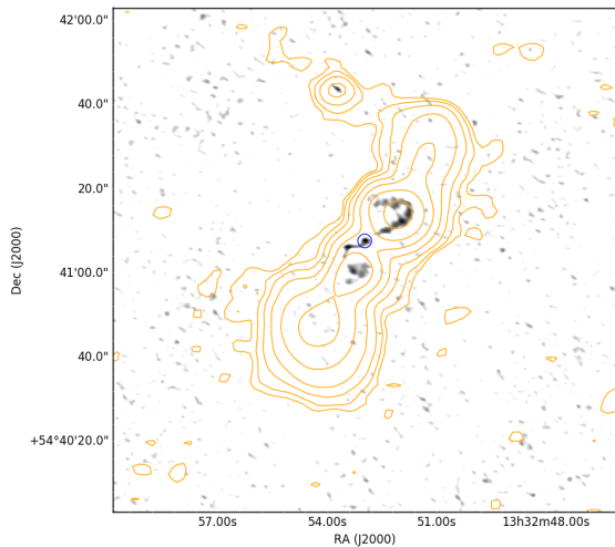
A.1. 29 ILTJ133252.97+544103.2 (removed from sample) ROBUST: -\mathbf{0.5}
