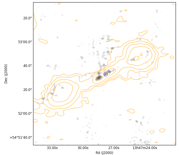
A.1. 30 ILTJ134727.92+545233.7 ROBUST: \mathbf{1.0}
