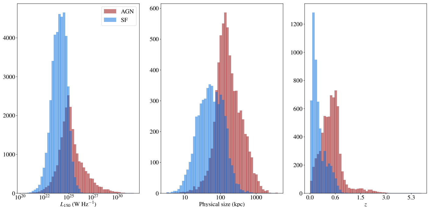
Fig. 6. Distributions of (left) radio luminosity, (middle) physical size, and (right) redshift for objects selected and not selected as RLAGN from the FCOZG sample using the criteria described in the text. All sources are shown in the left- and right-hand histograms, whereas in the middle only resolved sources (as defined in Section 2.1) are plotted.
