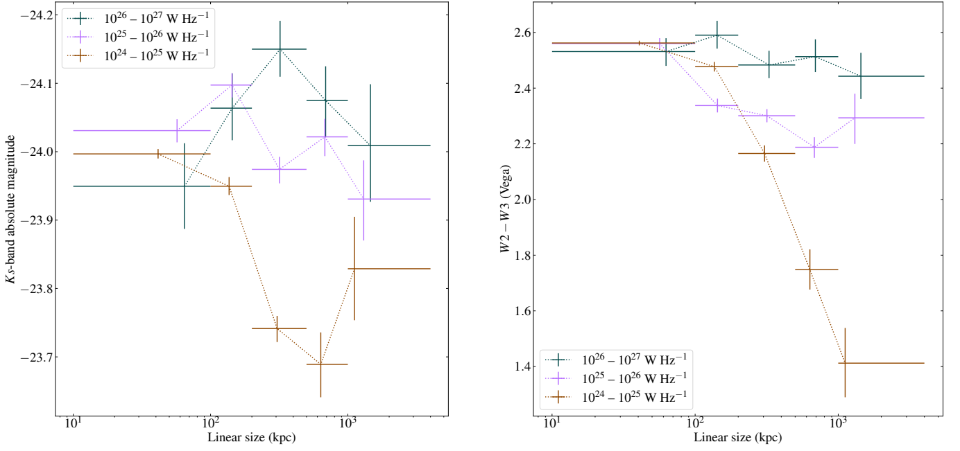
Fig. 10. Mean properties of the host galaxies of RLAGN as a function of projected linear size. Left: Ks -band rest-frame magnitude. Right: WISE band 2 minus band 3 colours (Vega magnitudes). In both plots the vertical error bars represent 1\sigma errors derived from bootstrap, the horizontal bars represent the bin range, and the position of the central point represents the mean projected linear size within the bin. Dotted lines joining points in a particular sample are to guide the eye only.
