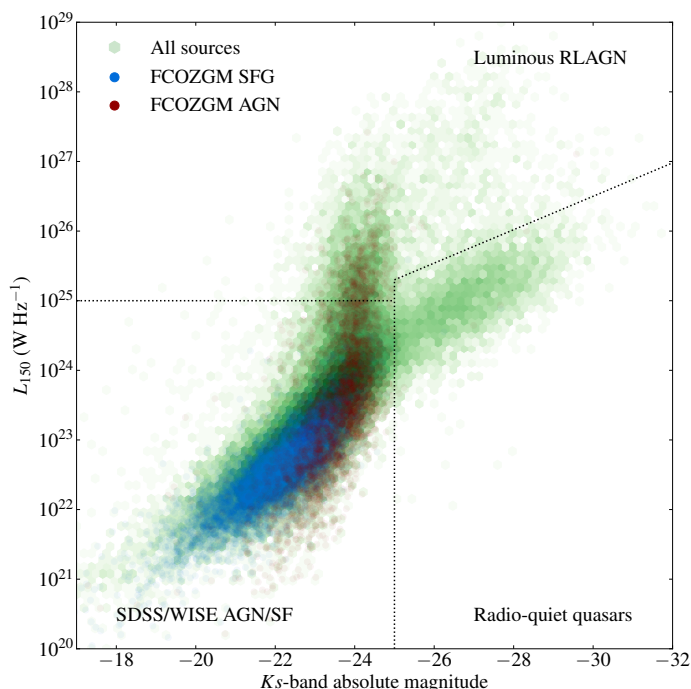
Fig. 5. Radio luminosity vs. Ks -band absolute magnitude for the FCOZGM sample. Overlaid on the density plot showing the full sample are the locations of FCOZGM RLAGN and FCOZGM SFG. Lines show the divisions on the plot used to select optically classified or radio-luminous AGN.
