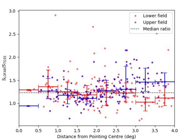
(a) Using the TGSS-ADR catalogue from Intema et al. (2017)
