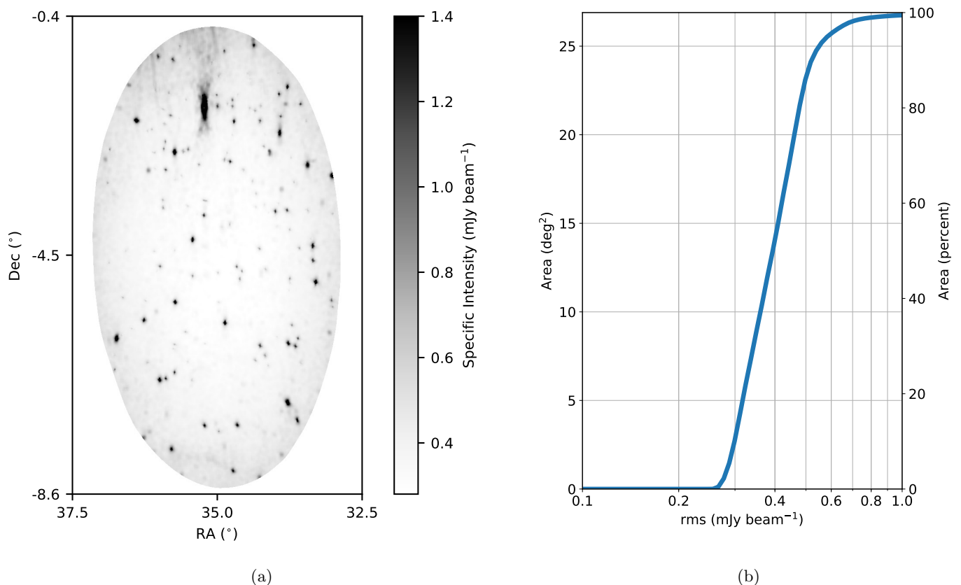
Fig. 5: rms coverage of the LOFAR XMM-LSS images. Panel (a) shows an image of the rms coverage across the field in which the flux scale varies between \sigma_{\text{cen}} and 5\sigma_{\text{cen}} , where \sigma_{\text{cen}} is the central rms of the image that was found to be 0.28 \text{ mJy beam}^{-1} . Panel (b) shows a plot of the area of the field that has an rms less than the given value. On the left-hand y-axis this is as a function of area in \text{deg}^2 and on the right-hand y-axis it is given as a percentage of the total area. The noise can be relatively high around bright sources in the field.
