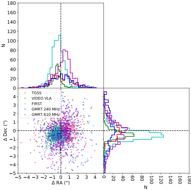
Fig. 9: Positional RA and Dec offsets of the LOFAR sources compared to TGSS-ADR (Intema et al. 2017, red), VIDEO VLA observations (Heywood et al. in prep, green), FIRST (Becker et al. 1995, Helfand et al. 2015, cyan), and GMRT observations (Tasse et al. 2007) at 240 MHz (blue) and 610 MHz (magenta). The histograms are both modelled as a Gaussian and the median values are used to quantify the average offsets. The values of these are given in Table 5. For the histogram, the errors are calculated by the 16th and 84th percentiles.
