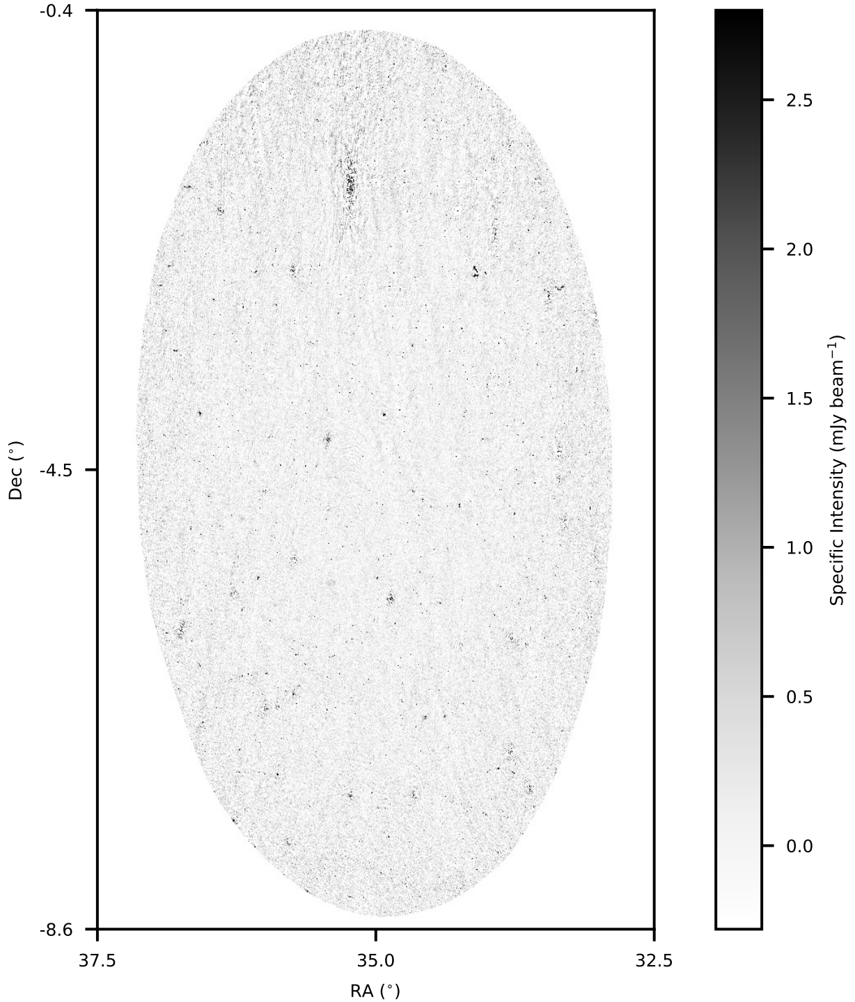
Fig. 3: Image of the XMM-LSS field observations imaged with LOFAR at \sim 150 MHz covering \sim 27 deg 2 . The associated flux scale is shown on the right-hand side in mJy beam -1 . The flux scale was chosen to range between -\sigma_{\text{cen}} and 10\sigma_{\text{cen}} , where \sigma_{\text{cen}} is the central rms of the image, which was determined to be 0.28 mJy beam -1 .
