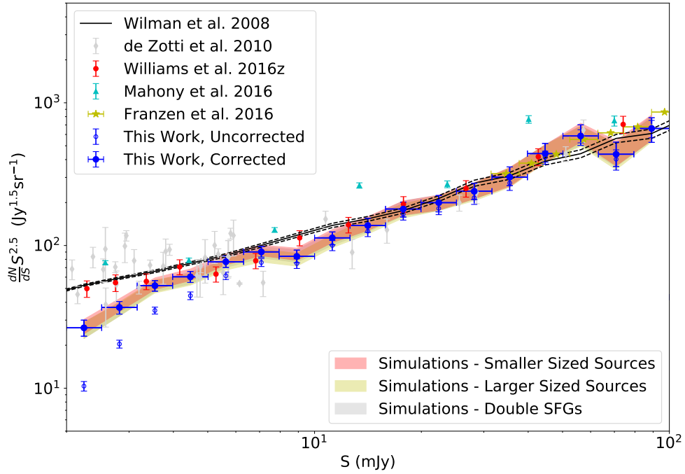
(b) Corrected using FDR correction and the completeness correction Method 2.
