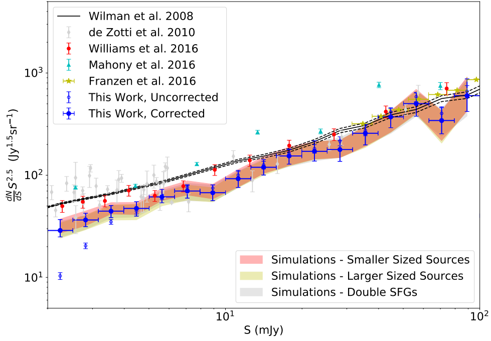
(a) Corrected using FDR correction and the completeness correction Method 1.
