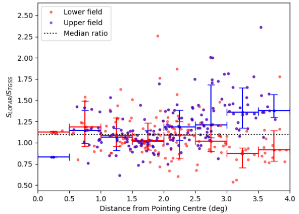
(b) Using the rescaled TGSS-ADR catalogue from Hurley-Walker (2017)
