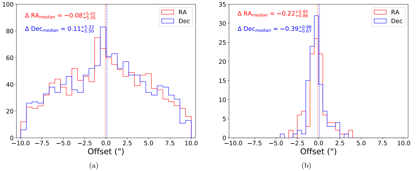
Fig. 10: Positional RA (red) and Dec (blue) offsets of the LOFAR sources compared to VIDEO sources (Jarvis et al. 2013). Shown in (a) is the histogram for all matches within 10" and in (b) is a histogram of offsets for the best-matched VIDEO source for each LOFAR source that had a VIDEO source within 10". The upper left shows the median offsets and the errors associated with these from the 16th and 84th percentiles. The dashed line indicates the median offset value for either the RA offsets (red) or Dec offsets (blue). Offsets are defined as RA_{\text{LOFAR}} - R_{\text{VIDEO}} and similar for Dec.
