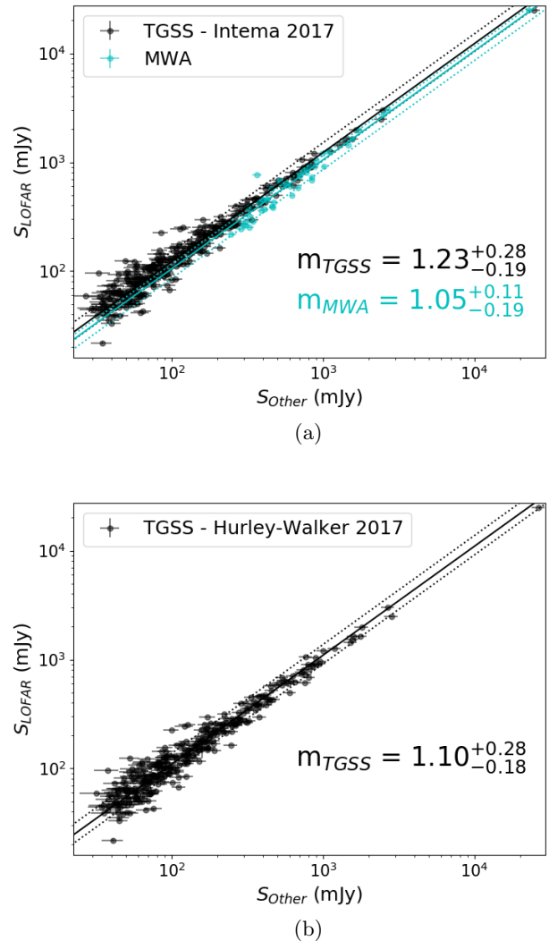
Fig. 7: Comparisons of the integrated flux recorded by LOFAR to that recorded by TGSS-ADR (black) and MWA (cyan) in Figure (a) and from the rescaled TGSS-ADR catalogue from Hurley-Walker (2017) in Figure(b). The black/cyan dotted lines show the fit to the data of the ratio between LOFAR to TGSS-ADR/MWA is used. The dotted lines indicate the errors associated with these fits (generated using the 16th and 84th percentiles). We quote the value of the median S_{LOFAR}/S_{TGSS} and S_{LOFAR}/S_{MWA} values and their errors in the lower right corner.
