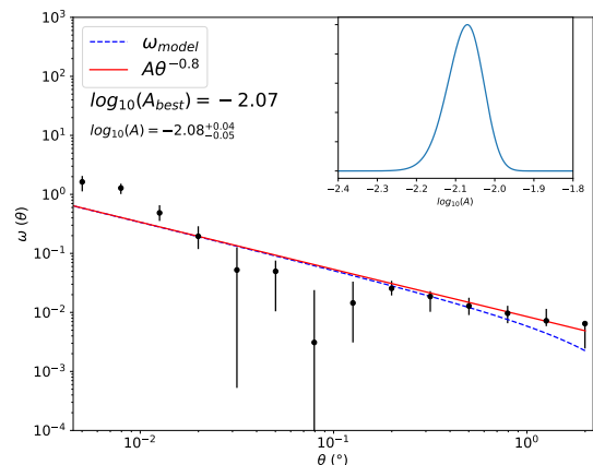
Fig. 14: Clustering in the XMM-LSS field for the merged source galaxy catalogue for a fixed slope of \gamma=0.8 . The insets in the upper right-hand corner quantifies the probability distribution derived from the \chi^2 values when fitting of the amplitude of the correlation function, A .
