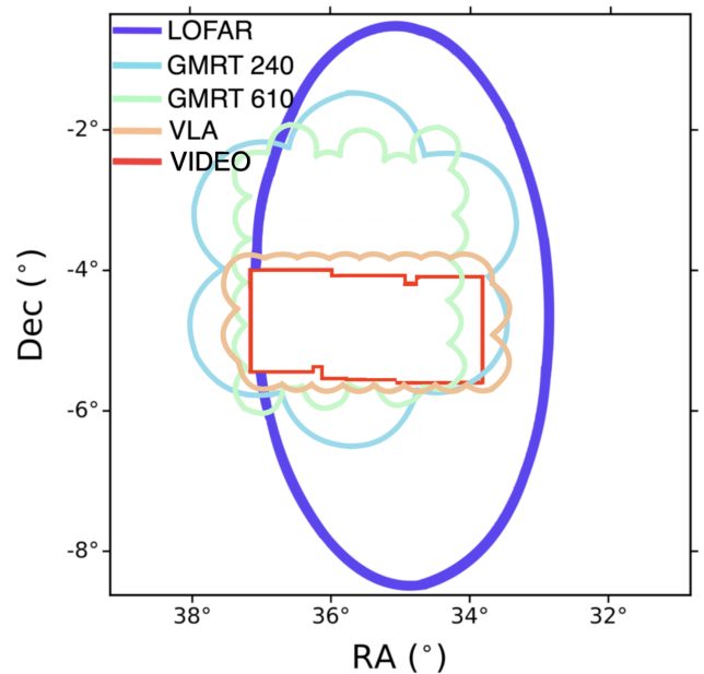
Fig. 6: Locations of targeted radio observations that have covered the XMM-LSS field at various radio frequencies. Shown are the observations presented in this paper (purple), observations from Tasse et al. (2007) at 240 MHz (blue) and 610 MHz (green), recent JVLA observations of the VIDEO field of Heywood et al. (in prep) (orange), and the near-IR VIDEO observations from Jarvis et al. (2013) (red).
