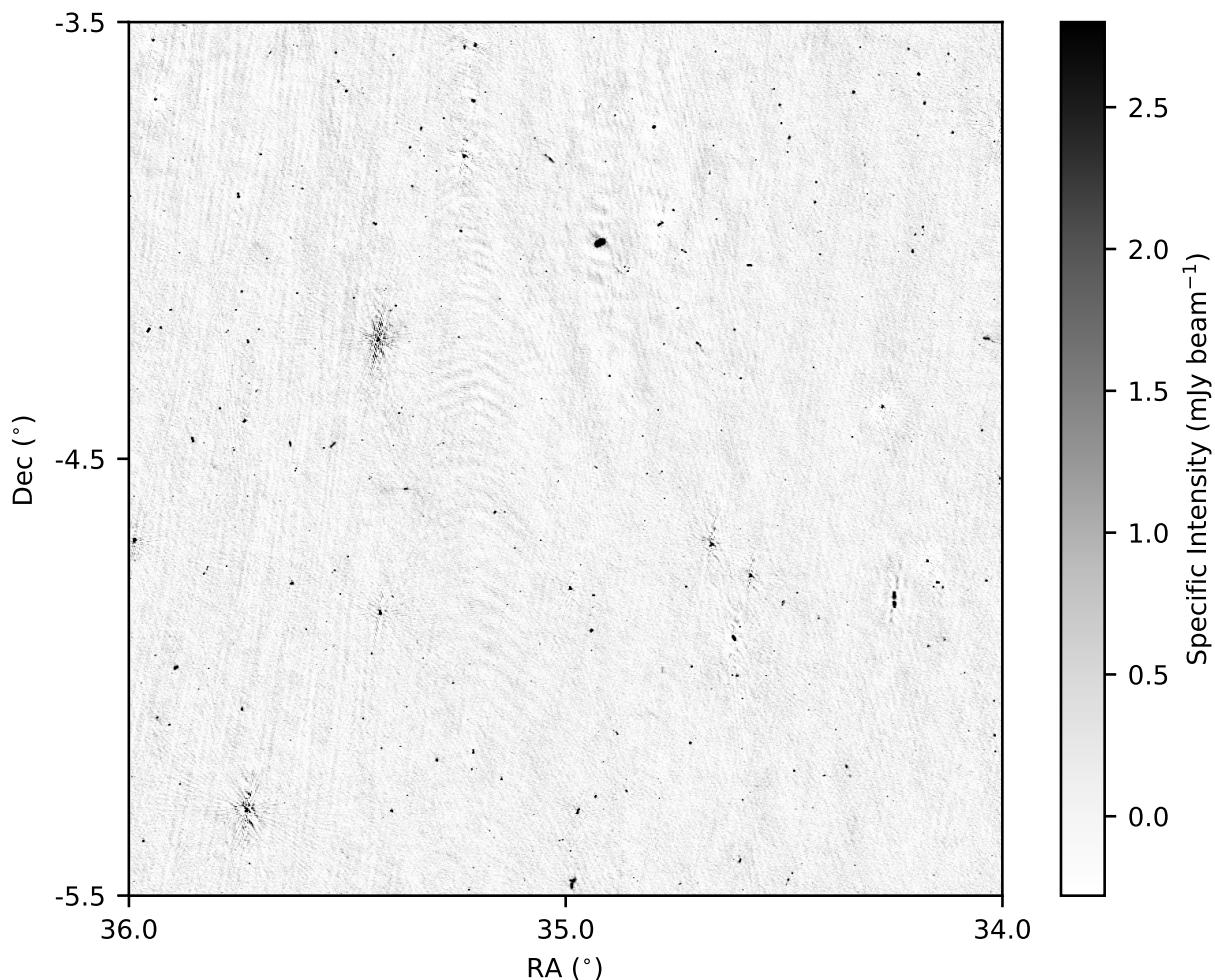
Fig. 4: Image of the central 4 \text{ deg}^2 of the field, containing \sim 600 sources. This has the same flux scale as Figure 3, ranging between -\sigma_{\text{cen}} and 10\sigma_{\text{cen}} , where \sigma_{\text{cen}} is the central rms of the image, which is 0.28 \text{ mJy beam}^{-1} . This zoomed-in image allows the presence of multi-component sources in this field to be seen.
