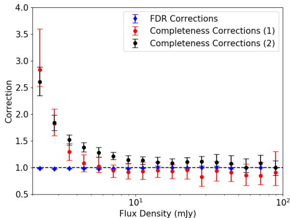
Fig. 12: Correction factors calculated and then applied to the source counts from the catalogue using the methods described in Sections 6.1 and 6.2: FDR corrections (blue) and completeness/resolution correction using Method 1 (red) and Method 2 (black).
