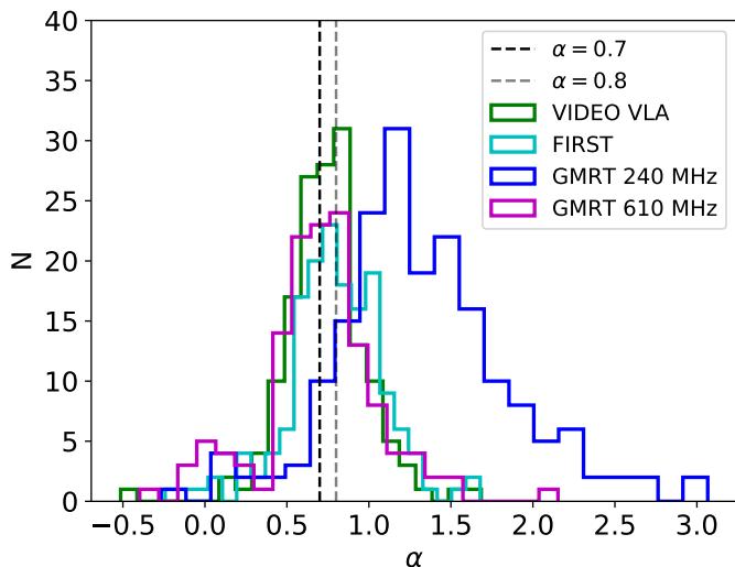
Fig. 11: Histograms showing the measured spectral index, \alpha , of sources in this field through matching to VIDEO VLA observations (Heywood et al. in prep, green), FIRST (Becker et al. 1995, Helfand et al. 2015, cyan), and GMRT observations (Tasse et al. 2007) at 240 MHz (blue) and 610 MHz (magenta) within a 5'' radius.
