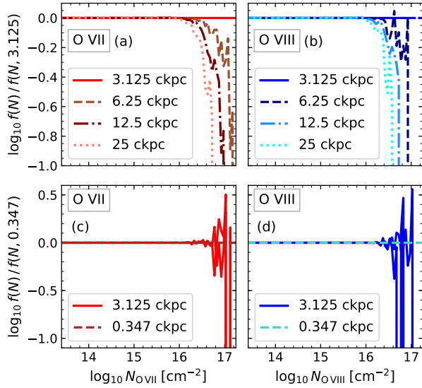
Figure A1. Convergence of the column density distribution function (CDDF, f(N) ) with pixel size. The left panels show O VII, the right panels show O VIII. In all panels, the solid line shows the CDDF as used throughout the paper: the column density is calculated on a grid of 32000^2 pixels, for each of 16 slices through the 100 cMpc box along the projection axis. These CDDFs are from the reference (Ref-L100N1504) simulation at z = 0.1 . In the top panels (a, b), this CDDF is compared to that obtained by degrading the resolution of the 3.125^2 ckpc ^2 pixel grid to get grids of 6.25^2 (dashed), 12.5^2 (dot-dashed) and 25^2 ckpc ^2 (dotted) pixels. The legends indicate the pixel sizes. In the bottom panels (c, d), the column density distributions extracted from two smaller regions ( 10 \times 10 cMpc ^2 ) at this standard resolution ( 3.125^2 ckpc ^2 per pixel) are compared with the CDDFs from the same region at nine times higher resolution. The CDDFs at different resolution are shown relative to the highest-resolution CDDF for the same region.
