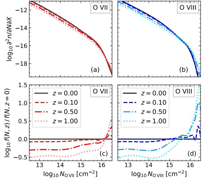
Figure 3. The evolution of the column density distribution function (CDDF) of O VII (a, c) and O VIII (b, d) in the 100 cMpc EAGLE reference simulation at from z = 1-0 . The top panels show the CDDFs themselves, while the bottom panels show the CDDFs relative to the z = 0 CDDF. This shows that the CDDF evolves only mildly between redshifts 0 and 1.
