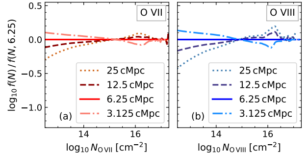
Figure A2. Convergence of the column density distribution function (CDDF, f(N) ) with slice thickness. The left panel shows O VII, the right panel shows O VIII. In both panels, the solid line shows the CDDF as used throughout the paper: the column density is calculated on a grid of 32000^2 pixels, for each of 16 slices through the 100 cMpc box along the projection axis. For the other lines, the thickness of the box slices for which the column density is calculated is varied as indicated. These CDDFs are from the reference (Ref-L100N1504) simulation at z = 0.1 . The differences between CDDFs for different slice thickness are mostly \lesssim 0.2 dex, which is small compared to the more than 8 orders of magnitude the CDDFs span in this column density range.
