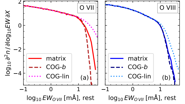
Figure B1. A comparison of methods to obtain the rest-frame equivalent width distribution from the CDDF. The rest frame EW distributions for O VII, \lambda = 21.60 \text{ \AA} (a) and the O VIII, \lambda = 18.97 \text{ \AA} doublet (b) in the Ref-L100N1504 simulation at redshift 0.1 are shown. The lines labelled ‘COG- b ’ are for EWs calculated from the CDDF using a single curve of growth with the best-fit b parameters to the relation between log EW and the column density obtained for a set of absorption spectra. The dotted line (‘COG-lin’) is for EWs calculated using the linear curve of growth for each ion. For the lines labelled ‘matrix’, the conversion from CDDF to EW distribution was done using a matrix generated from the column density-EW relation in Fig. 5, which accounts for scatter. We use the CDDF for 6.25 cMpc slices.
