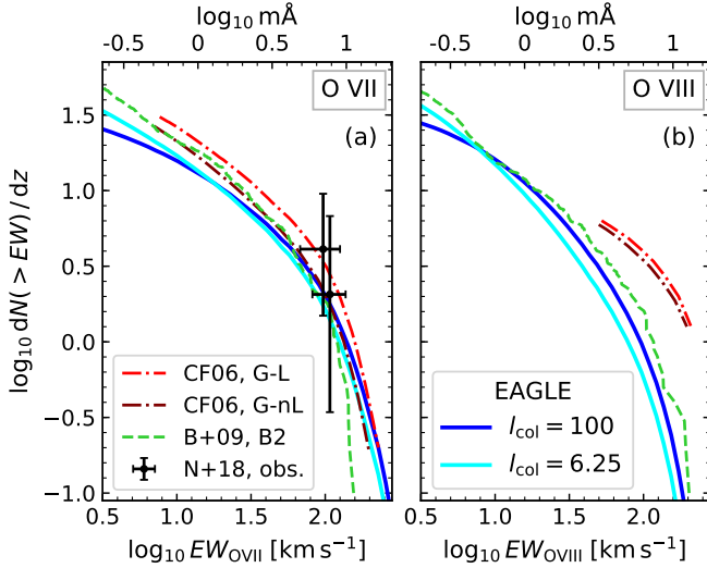
Figure 6. Comparison between the O VII (a) and O VIII (b) rest-frame equivalent width distributions in the EAGLE reference simulation (Ref-L100N1504) at z = 0.1 , the GSW model of Cen & Fang (2006) (CF06) at z \sim 0 with (G-L) and without (G-nL) assuming ionization equilibrium, the Branchini et al. (2009) (B+09) B2 model at z \leq 1 , and observations by Nicastro et al. (2018) with the update of Nicastro (2018) (N+18). Note that the units differ from those in Fig. 5: the equivalent widths are in km/s (still rest-frame), and the number of absorption systems per unit absorption length X . The EAGLE distributions were computed using the 100 cMpc and 6.25 cMpc CDDFs and the 100 cMpc column density equivalent width relation calibrated to all the sightlines in our sample. This shows the rough agreement between the equivalent width distribution we predict for O VII and that predicted in other work, and an agreement with the available observations. The O VIII distributions have larger differences, and there are no extant observational constraints we are aware of.
