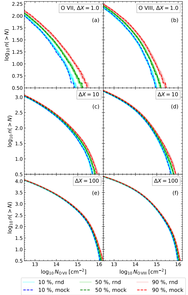
Figure C1. The cumulative column density distributions for mock surveys of sizes \Delta X = 1.01 ( \Delta z = 0.878 ; a, b), \Delta X = 10.0 ( \Delta z = 8.66 ; c, d), and \Delta X = 100 ( \Delta z = 86.7 ; e, f), of O VII (a, c, e) and O VIII (b, d, f) in the reference (Ref-L100N1504) simulation at redshift 0.1. The column densities are calculated for 16 6.25 cMpc slices, each with 3.125^2 ckpc 2 pixels. The dashed lines show mock surveys, where (x, y) positions were selected at random, and then each slice along the z -axis at that position was included, mimicking the measurement of different absorption systems along full 100 cMpc sightlines. This accounts for clustering along the line of sight on scales between 6.25 and 50 cMpc (i.e. half the size of the periodic box). We obtained a sample of 100 such mock surveys. At each column density, show the 10 th (blue), 50 th (green, median), and 90 th (red) percentiles of the distribution of absorber counts from the different mock surveys. To find the effect of large-scale structure on this distribution, we repeated this process for random surveys, show in lighter solid colors, where we select the same number of 6.25 cMpc columns, but choose them randomly. For these random surveys, we show the percentiles for ten different sets of 100 random surveys. The good agreement between the solid and dashed curves indicates that large-scale structure does not seem to affect the statistical variation in CDDFs that surveys may measure on scales of 6.25–50 cMpc.
