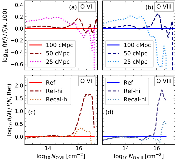
Figure A3. Convergence of the column density distribution function with simulation box size (top panels) and resolution (bottom panels). The left panels show O VII, the right panels show O VIII. The plots show the CDDF f(N, z = 0.1) , as described in equation 1, relative to a reference CDDF. In the top panels, the CDDFs from Ref-L025N0376 and Ref-L050N0752 are compared to the standard Ref-L100N1504 CDDF. In the right panels, Ref-L025N0376 (‘Ref’) is compared to the Ref-L025N0752 and Recal-L025N0752 (‘Ref-hi’, ‘Recal-hi’) CDDFs.
