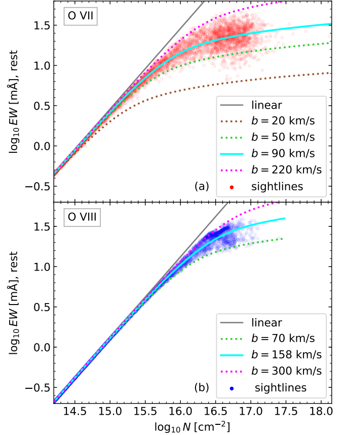
Figure 5. The curve of growth for the O VII resonant line (a) and the O VIII doublet (b) in the reference (Ref-L100N1504) simulation at redshift 0.1. We plot the rest frame equivalent width calculated over the full 100 cMpc sightlines against the column density along those same sightlines. The solid cyan lines are for the best-fit b parameters to the log equivalent width, using only the sightlines selected for the ion in question. The solid gray lines indicate the linear column density equivalent width relation, which applies to optically thin gas. The dashed lines roughly indicate the upper and lower range of b parameters. This demonstrates our sampling of the column density equivalent width relation, and the range of single-absorber-equivalent widths associated with it.
