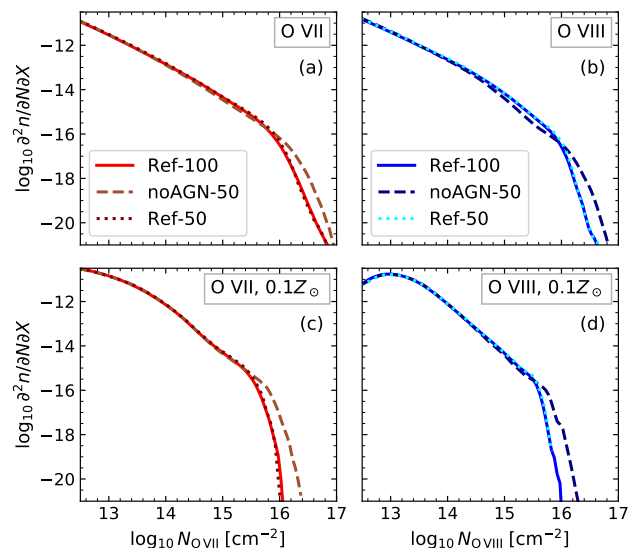
Figure 10. The top panels (a, b) compare the reference and no AGN models, to show the effect of AGN feedback on the z = 0.1 O VII (left panels) and O VIII (right panels) CDDFs. The column density distribution in the no AGN simulation (NoAGN-L050N0752, ‘noAGN-50’) is compared to the reference simulation (Ref-L100N1504, ‘Ref-100’). We also show the 50 cMpc reference simulation (Ref-L050N0752, ‘Ref-50’) results to demonstrate that differences between the reference and no AGN simulation distributions are not due to the size of the simulation domain. To gauge how much of the differences are due to differences in gas oxygen content, we show CDDFs made assuming all gas has a metallicity of 0.1 Z_{\odot} in the bottom panels. This shows that beyond the break in the CDDF, a boost in metal enrichment due to AGN feedback partly offsets its other effects.
