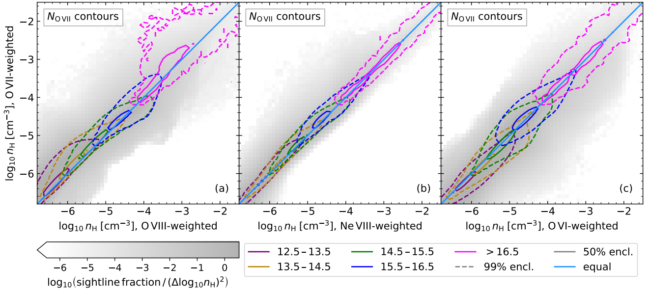
Figure 16. The O VII-weighted density (horizontal) of absorption systems plotted against the O VIII-weighted density (a), the Ne VIII-weighted density (b), and the O VI-weighted density (c) along the same sightline. These sightlines are our 6.25 cMpc long columns, and come from 32000 2 pixel projections of the reference (Ref-L100N1504) simulation at redshift 0. The greyscale shows the total sightline distribution, while the contours show the density distributions for different O VII column density bins, matching those in Fig. 11. These ranges are given in units of \log_{10} \text{cm}^{-2} . The light blue lines indicate where the densities are equal. This indicates that these ions tend to trace gas with similar densities along the same sightline, though there are small systematic differences at low column densities.
