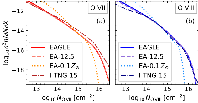
Figure 2. The column density distribution function (CDDF), as described in equation 1, of O VII (a) and O VIII (b) in the 100 cMpc EAGLE reference simulation at z = 0.0 . The solid lines (EAGLE) show our standard CDDF: it uses the simulation oxygen abundances, and column densities are measured in 6.25 cMpc long columns. The dotted lines (EA-0.1 Z_{\odot} ) use 0.1 times the solar abundance for all gas instead. All the EAGLE column densities are calculated from 32000^2 columns in each slice along the line of sight direction; each column has an area of 3.125^2 ckpc ^2 . We also compare to the IllustrisTNG 100-1 CDDF (Nelson et al. 2018, I-TNG-15), shown with dot-dashed lines. Since these column densities were measured in 15 cMpc columns, we also show the CDDF we obtain using 12.5 cMpc columns for comparison (dashed lines, EA-12.5). This shows that EAGLE and IllustrisTNG-100 predict similar column density distributions for these ions, and that using realistic metallicities is crucial in determining the column density distribution.
