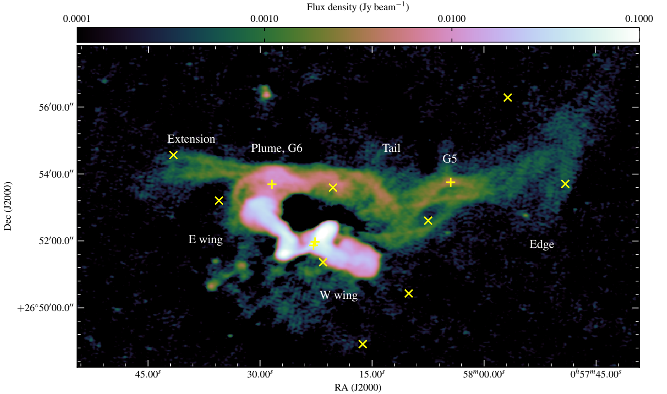
Figure 1. LOFAR colourscale of the radio emission from NGC 326. The colour scale is logarithmic over the range shown by the colour bar (in units of \text{Jy beam}^{-1} for the resolution of 8.2 \times 5.1 arcsec), yellow crosses mark the positions of potential cluster members; + signs are those in the spectroscopic study of Werner et al. (1999) and × signs show candidate galaxies selected from NED as described in the text. The double nuclei of NGC 326 are represented by the two adjacent crosses close to the centre of the image. Features referred to in the text are labelled.
