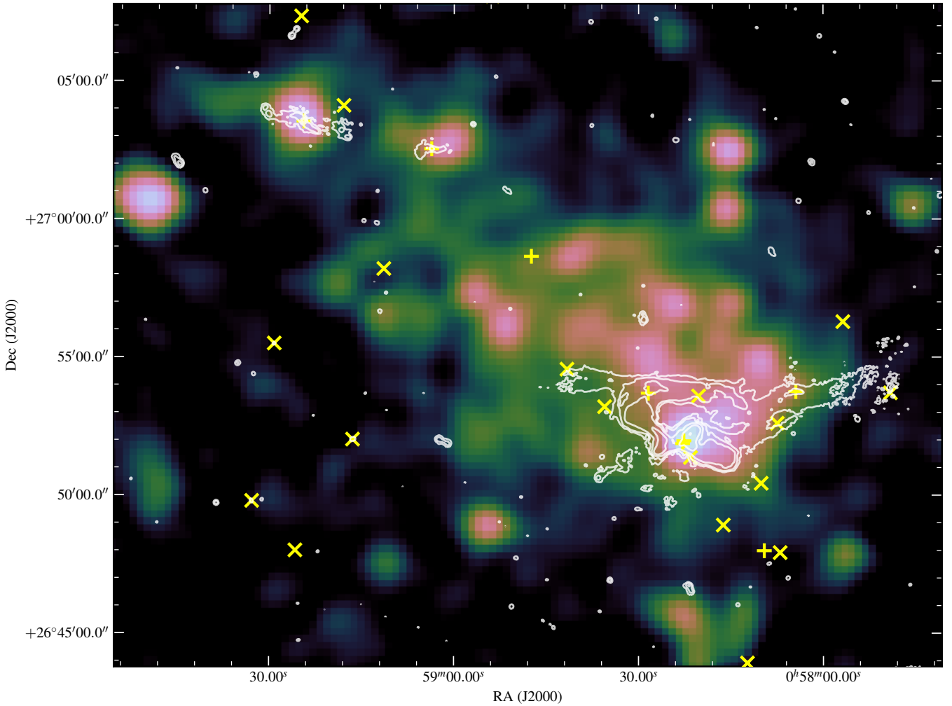
Figure 2. LOFAR contours of radio emission from the NGC 326 field (white, at 0.5 \times (1, 4, 16 \dots) mJy beam ^{-1} ) overlaid on a Gaussian-smoothed exposure-corrected ROSAT image with a logarithmic transfer function (colour). Crosses as in Fig. 1.
