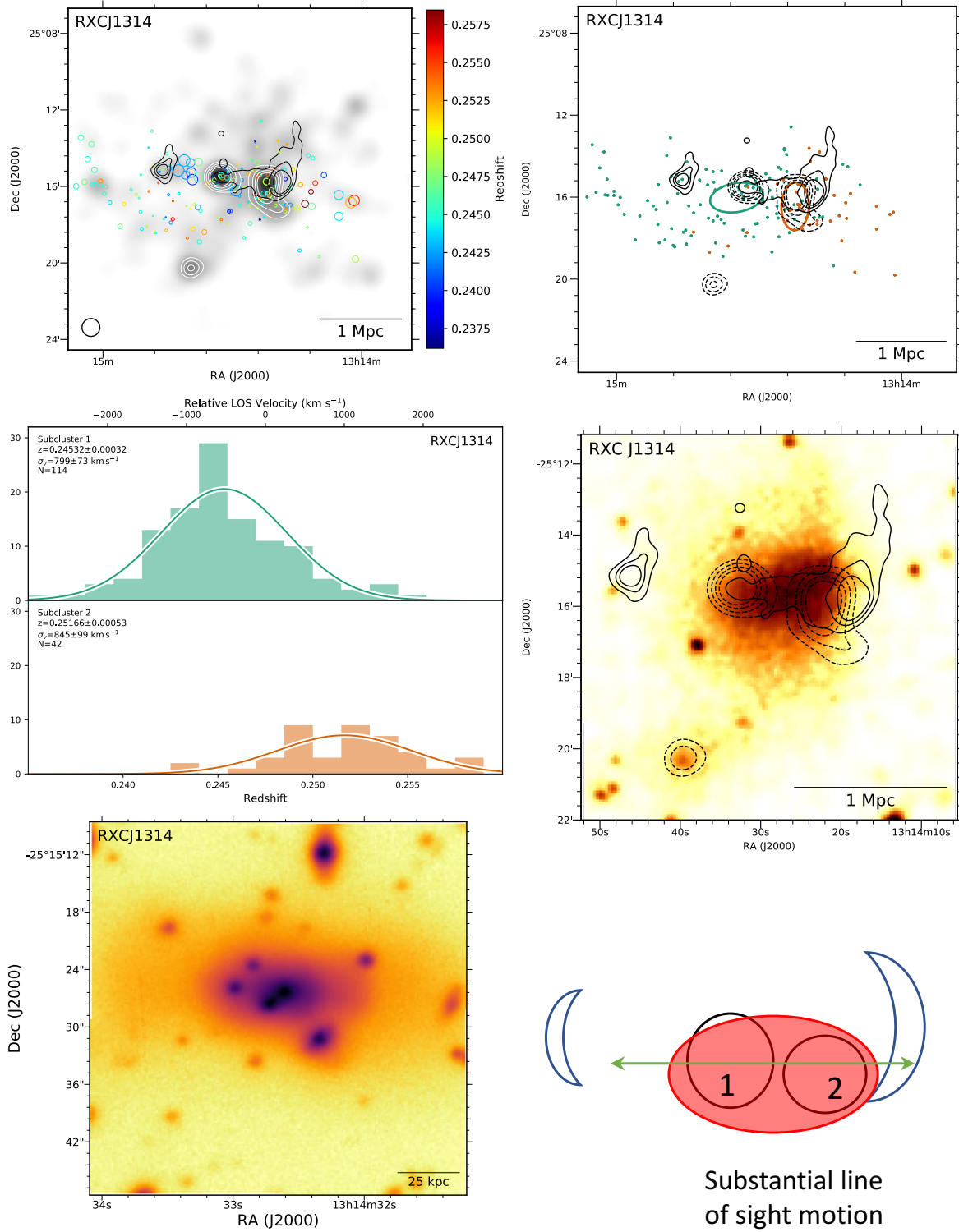
Figure 33. Top left: DS-test over red sequence Subaru/SuprimeCam r-band luminosity distribution with linearly spaced white contours. The black contours show VLA 2-4 GHz contours (P.I. Dawson). Top right: Subcluster membership of spectroscopic cluster members assigned with our GMM analysis. The same VLA contours (solid) and red sequence luminosity contours (dashed) are depicted. Middle left: Subcluster redshift histogram with colors matching the image at the top right. Middle right: 110 ks XMM image with the same VLA radio contours (solid) and red sequence luminosity contours (dashed). Bottom left: 150 kpc cutout of the Subaru r-band image centered on the cluster BCG in subcluster 1. Bottom right: Preferred merger scenario. The two subclusters and radio relics are aligned with the extended X-ray emission. A large line of sight velocity difference between the two subclusters is discovered suggesting a substantial component of the merger axis is along the line of sight, which is an outlier among other bimodal, double relic systems. A third subcluster is detected to the southeast, in the red sequence luminosity and X-ray surface brightness. It may have interacted in a glancing collision given the stream of X-ray emission connecting it to the cluster center.
