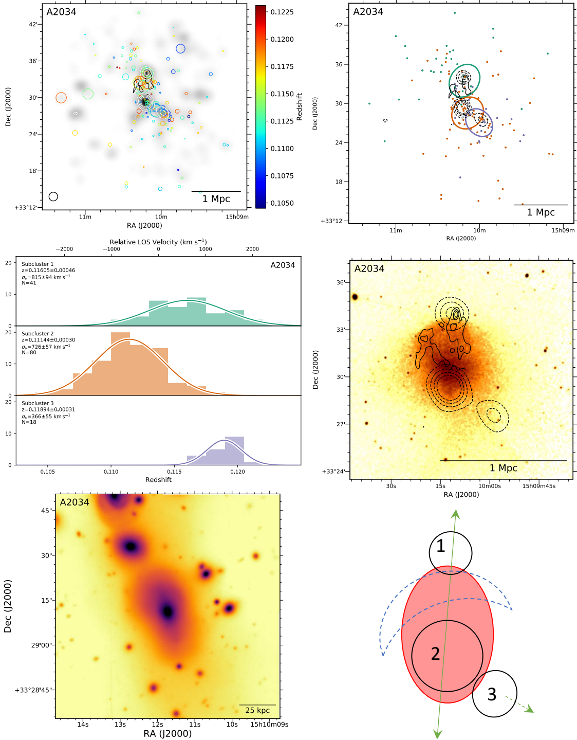
Figure 18. Top left: DS-test over red sequence R-band luminosity distribution with linearly space white contours. The black contours show the 1.4 GHz WSRT contours (van Weeren et al. 2011b). Top right: Subcluster membership of spectroscopic cluster members assigned with our GMM analysis. The same WSRT contours (solid) and red sequence luminosity contours (dashed) are depicted. Middle left: Subcluster redshift histograms with colors matching the image at the top right. Middle right: 261 ks Chandra image with the same WSRT radio contours (solid) and red sequence luminosity contours (dashed). The relics and disturbed ICM are suggestive of a merger between at least two subclusters; however, the lack of X-ray emission with subcluster 3 suggests it was also involved. Bottom left: 150 kpc cutout of the Subaru/SuprimeCam R-band image centered on the cluster BCG in subcluster 2. Bottom right: Proposed merger scenario. A2034 is primarily a north to south merger with two complications. First, the shock has been classified as a cold front in the literature, which would better explain subcluster 1’s location; however, the relic candidate is coincident with this edge in the ICM. Second, subcluster 3 appears to have exited toward the southwest having its ICM stripped.
