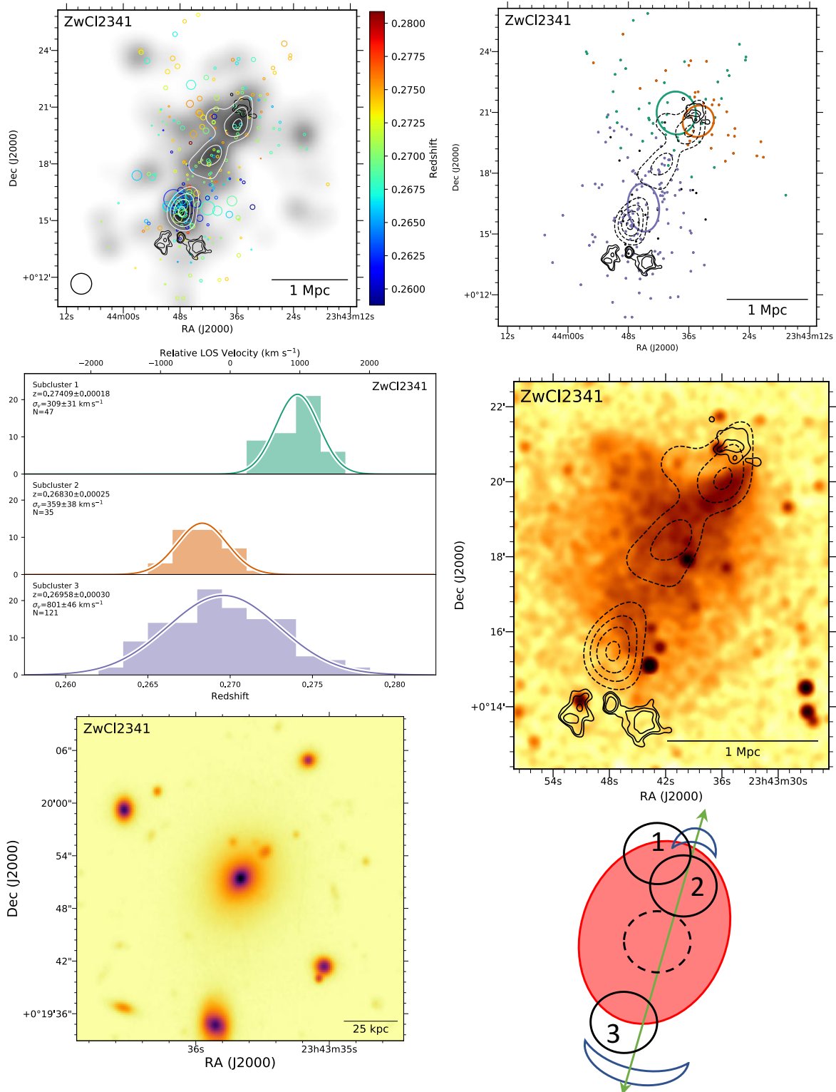
Figure 37. Top left: DS-test over red sequence Subaru/SuprimeCam r-band luminosity distribution with linearly spaced white contours. The black contours show GMRT 610 MHz contours (van Weeren et al. 2009b). Top right: Subcluster membership of spectroscopic cluster members assigned with our GMM analysis. The same WSRT contours (solid) and red sequence luminosity contours (dashed) are depicted. Middle left: Subcluster redshift histogram with colors matching the image at the top right. Middle right: 227 ks Chandra image with the same GMRT radio contours (solid) and red sequence luminosity contours (dashed). Bottom left: 150 kpc cutout of the Subaru r-band image centered on the cluster BCG in subcluster 1. Bottom right: Preferred merger scenario. We detect three subclusters with our GMM as well as a fourth that is evident in the red sequence luminosity distribution. Two subclusters (subclusters 2 and 3) and the candidate third situated in the middle of the cluster are aligned with the two radio relics. This suggests the dominant component of the merger is occurring along this axis with at least two subclusters partaking. Subcluster 1 is positioned to the east of subcluster 2, and is evident in both the X-ray surface brightness profile and red sequence luminosity. The disturbed gas suggests it has already merged, and the large line of sight velocity difference suggests line of sight motion.
