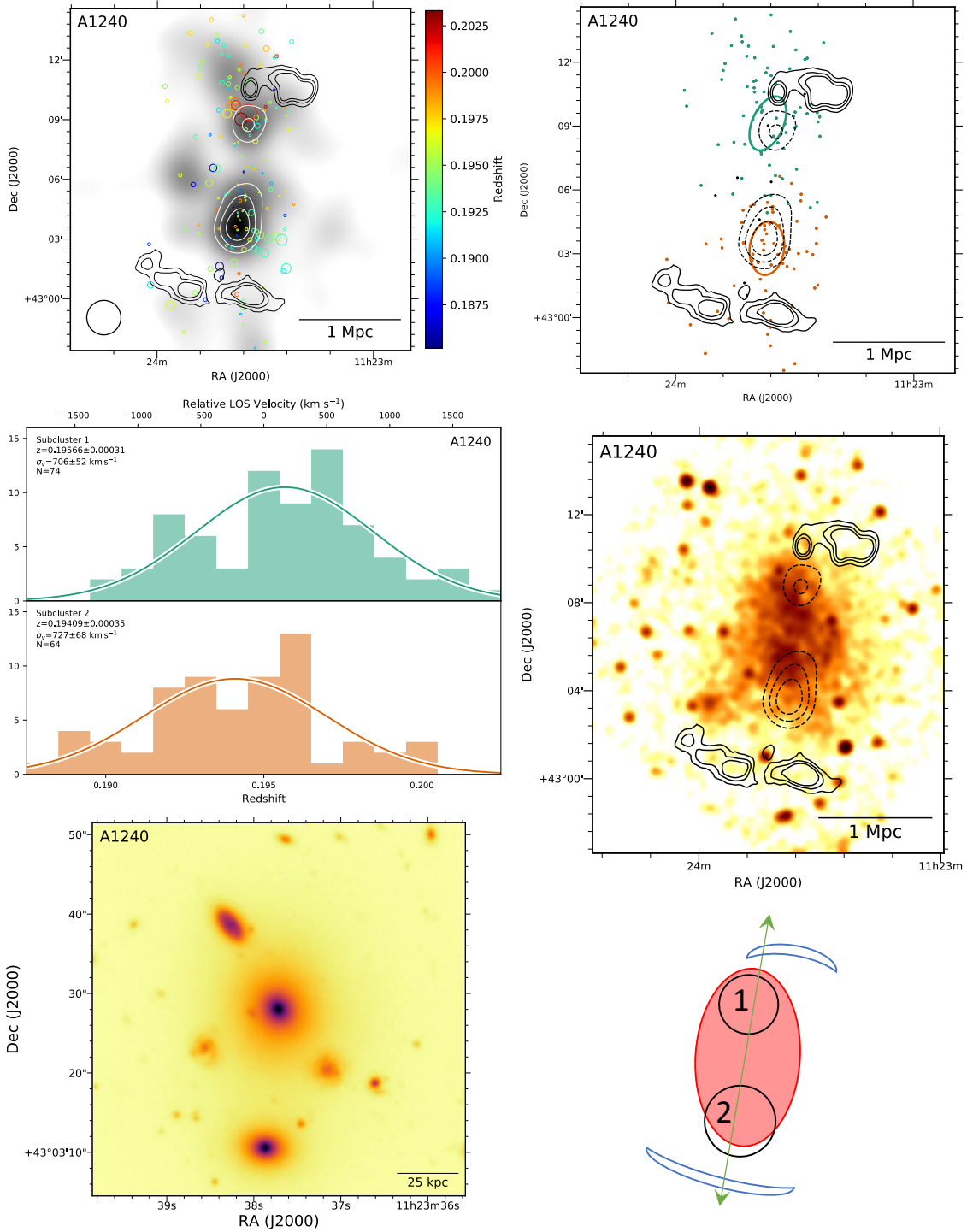
Figure 15. Top left: DS-test over red sequence r-band luminosity distribution with linearly spaced white contours. The black contours show the 1.4 GHz VLA contours (Bonafede et al. 2009). Top right: Subcluster membership of spectroscopic cluster members assigned with our GMM analysis. The same VLA contours (solid) and red sequence luminosity contours (dashed) are depicted. Middle left: Subcluster redshift histograms with colors matching the image at the top right. Middle right: 52 ks Chandra image with the same VLA radio contours (solid) and red sequence luminosity contours (dashed). The relics and disturbed ICM are suggestive of a merger between subclusters 1 and 2. Bottom left: 150 kpc cutout of the Subaru/SuprimeCam r-band image centered on the southern BCG, which is associated with subcluster 2. Bottom right: Proposed merger scenario. A1240 is a clean bimodal merger with two radio relics colinear with the two subclusters.
