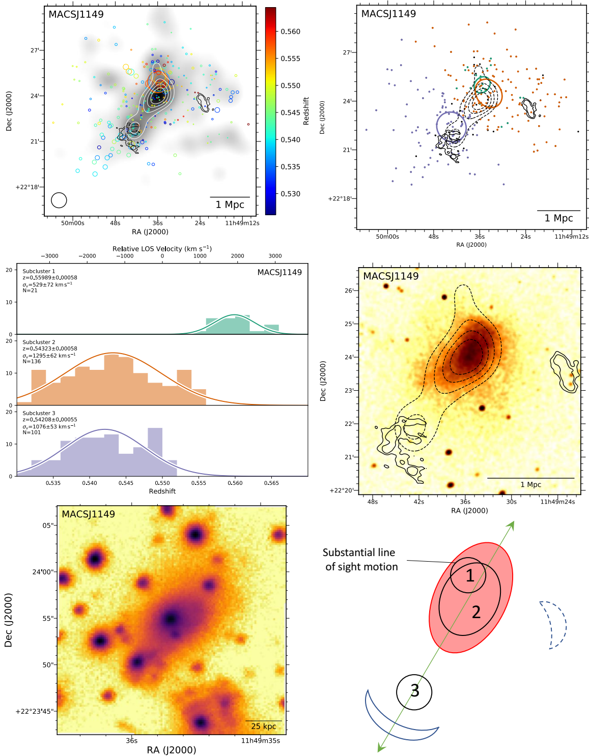
Figure 28. Top left: DS-test over red sequence Subaru/SuprimeCam R-band luminosity distribution with linearly spaced white contours. The black contours show GMRT 323 MHz contours (Bonafede et al. 2012). Top right: Subcluster membership of spectroscopic cluster members assigned with our GMM analysis. The same GMRT contours (solid) and red sequence luminosity contours (dashed) are depicted. Middle left: Subcluster redshift histogram with colors matching the image at the top right. Middle right: 372 ks Chandra image with the same GMRT radio contours (solid) and red sequence luminosity contours (dashed). Bottom left: 150 kpc cutout of the Subaru R-band image centered on the cluster BCG in subcluster 2. Bottom right: Preferred merger scenario. A detailed dynamical study of MACSJ1149 was presented in Golovich et al. (2016).
