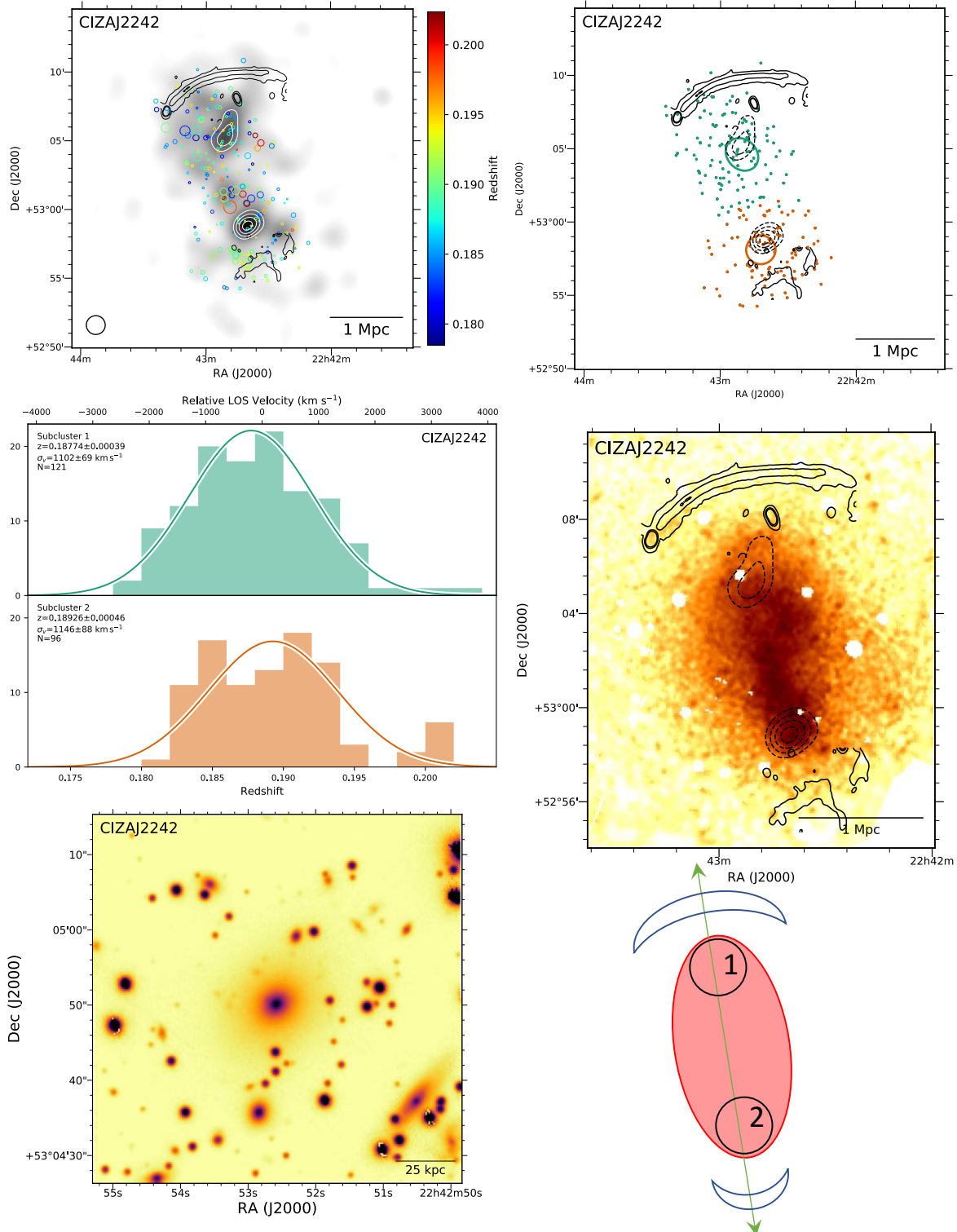
Figure 27. Top left: DS-test over red sequence Subaru/SuprimeCam i-band luminosity distribution with linearly spaced white contours. The black contours show WSRT 1382 MHz contours (van Weeren et al. 2010). Top right: Subcluster membership of spectroscopic cluster members assigned with our GMM analysis. The same WSRT contours (solid) and red sequence luminosity contours (dashed) are depicted. Middle left: Subcluster redshift histogram with colors matching the image at the top right. Middle right: 206 ks Chandra image with the same WSRT radio contours (solid) and red sequence luminosity contours (dashed). Bottom left: 150 kpc cutout of the Subaru i-band image centered on the cluster BCG in subcluster 1. Bottom right: Preferred merger scenario. CIZA J2242 is composed of at least two subclusters with similar velocity dispersions and redshifts suggesting a 1:1 merger in the plane of the sky. The ICM has been extremely disrupted and is situated between the two subclusters. The famous ‘Sausage’ radio relic in the north has been studied across a wide range of frequencies, and dark matter-galaxy offsets have been detected in this cluster (Jee et al. 2016). The high mass, simple geometry, and extreme shock features have motivated a number of simulation studies as well.
