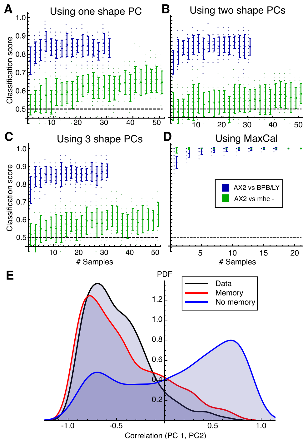
Figure 5. Discriminators trained on MaxCal behavioral descriptors perform better than shape alone. (A–C) Success rates for k -nearest neighbors based on the shapes of cells alone. Some number of samples are taken from the same condition and individually classified using the first 1 (A), 2 (B) or 3 (C) shape PCs, with the most commonly chosen classification used to identify the group. Classification is performed on both untreated vs BPB/LY treated (blue) and parental vs mhc - (green) data. (D) A similar k -nearest neighbor classification to (A–C), but with distances between neighbors based on the values of the two Lagrange multipliers that best separate the training data. (E) Degree of correlation between PC 1 and PC 2 across a number of simulated cell trajectories. Three lines are shown, corresponding to the data (black), a non-Markovian (red) master equation, in which transition probabilities depend on the last transition made, and a Markovian (blue) master equation, in which they simply depend on the current state. The Markovian model (without memory) lacks the skew toward negative correlations seen in the data. The non-Markovian model (with memory) recovers these.
