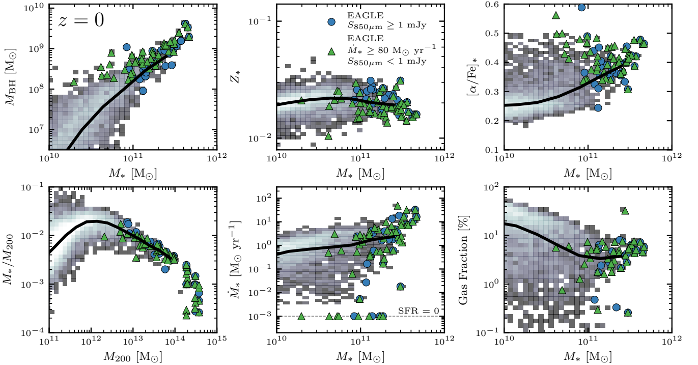
Figure 6. The properties at z = 0 of the descendants of the model galaxies in the S_{850\mu\text{m}} \geq 1 \text{ mJy} and highly star-forming Submm-Faint samples plotted as a function of either the stellar or halo mass. We plot the central supermassive black hole mass (top left), stellar metallicity (top centre), alpha-enhancement (top right), stellar mass to halo mass ratio (bottom left), SFR (bottom centre) and total gas fraction ( M_{\text{gas}}/M_{\text{gas}+\text{stars}} , bottom right). The total model galaxy population is represented as a two-dimensional histogram, coloured by the number of galaxies in each bin. The median trend for all galaxies is indicated via a solid line. We assign galaxies with a zero SFR to a value of \dot{M}_* = 10^{-3} M_\odot \text{ yr}^{-1} (indicated by a horizontal dashed line on the figure). In all panels, both central and satellite galaxies are shown (except in the lower left panel, where the general population only shows central galaxies for clarity). The once S_{850\mu\text{m}} \geq 1 \text{ mJy} galaxies are not obviously distinguishable from the general population at a given stellar mass in any of the integrated properties we have explored (i.e., they follow the median trends). However, the once highly star-forming Submm-Faint galaxies have, on average, overmassive black holes, lower metallicities and are more \alpha -enhanced for their stellar masses at z = 0 .
