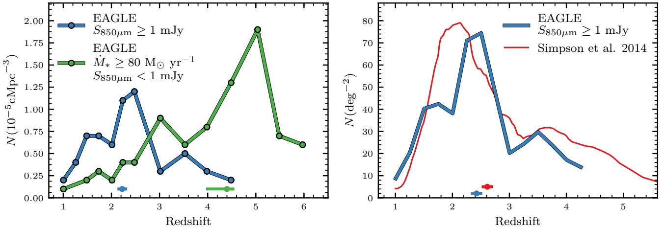
Figure 2. Left panel: the number density of the S_{850\mu\text{m}} \geq 1 \text{ mJy} and highly star-forming Submm-Faint model galaxies (in units of 10^{-5} \text{cMpc}^{-3} ) at each simulation snapshot. The median redshift of each sample is indicated by an error bar along the lower axis ( z = 2.2^{+0.1}_{-0.1} and z = 4.4^{+0.1}_{-0.4} for the S_{850\mu\text{m}} \geq 1 \text{ mJy} and highly star-forming Submm-Faint population, respectively). The galaxies in the S_{850\mu\text{m}} \geq 1 \text{ mJy} sample are most abundant at z \approx 2.5 and then become increasingly rare towards lower and higher redshift. The galaxies within the highly star-forming Submm-Faint sample are predominantly at higher redshift ( z > 4 ). Right panel: the number of S_{850\mu\text{m}} \geq 1 \text{ mJy} model galaxies per square degree (median value of z = 2.4^{+0.1}_{-0.1} ) compared to the statistically corrected observed sample of SMGs from Simpson et al. (2014) (median value of z = 2.6^{+0.1}_{-0.1} ). The shape and the median value are similar for the two distributions. The position of the peak is slightly higher for the sample of S_{850\mu\text{m}} \geq 1 \text{ mJy} model galaxies ( z \approx 2.5 ) compared to the observations ( z \approx 2 ).
