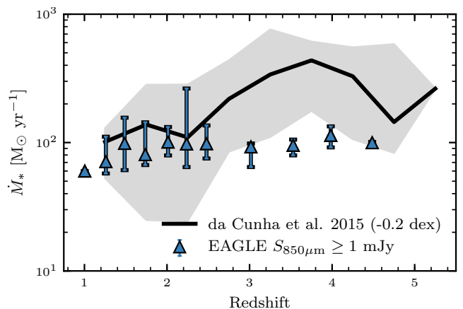
Figure 1. The median SFR as a function of redshift for both the EAGLE S_{850\mu\text{m}} \geq 1 mJy galaxies at each simulation snapshot and the observed SMGs from da Cunha et al. (2015) . A -0.2 dex SFR recalibration has been applied to the observational data at all redshifts (see Section 2.1.3). The error bars and the height of the shaded region outline the 10 th – 90 th percentile range. The SFRs of the model galaxies in the S_{850\mu\text{m}} \geq 1 mJy sample are high ( \dot{M}_* > 50 M_\odot \text{ yr}^{-1} , with a median SFR of 94 M_\odot \text{ yr}^{-1} ), and are in reasonable agreement with the SFRs inferred from the observations below z \approx 3 where the bulk of the population lie. However, the SFRs of the model galaxies in the high-redshift tail ( z \gtrsim 3 ) are a factor of \approx 3 lower than the observations.
