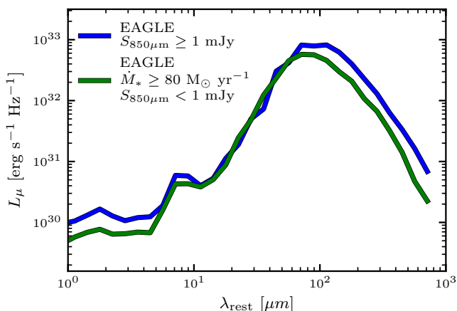
Figure 9. Composite broadband spectral energy distributions (SEDs) for the S_{850\mu\text{m}} \geq 1 mJy and highly star-forming Submm-Faint galaxies. The leftward shifting of the peak in the dust emission for the highly star-forming Submm-Faint sample signifies hotter dust temperatures than the S_{850\mu\text{m}} \geq 1 mJy galaxies.
