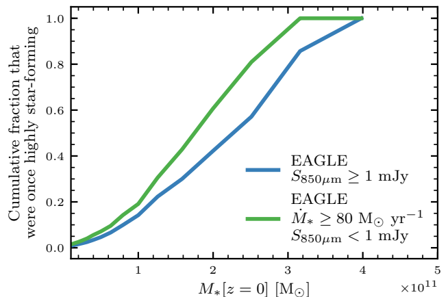
Figure 7. The cumulative fraction of galaxies at z = 0 that were ever once S_{850\mu\text{m}} \geq 1 mJy or highly star-forming and Submm-Faint, as a function of the present day stellar mass. The descendants of these galaxies are rare; only \approx 20\% of the galaxies at z = 0 with stellar masses greater than M_*[z = 0] \geq 10^{11} M_\odot were once highly star forming. However, this fraction rapidly increases to 100% for stellar masses M_*[z = 0] \geq 3 \times 10^{11} M_\odot .
