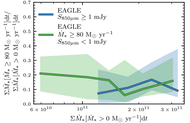
Figure 8. For the descendants of the model galaxies in the S_{850\mu\text{m}} \geq 1 mJy and highly star-forming Submm-Faint samples at z = 0 , the fraction of the total initial stellar mass formed in situ within the galaxy at a rate above \dot{M}_* \geq 80 M_\odot \text{ yr}^{-1} as a function of the total initial mass that formed in situ within the galaxy. On average, the fractions in both samples are low (10–20%, implying a typical starbursting duration of \approx 100 –400 Myr), indicating that high-SFR events are not the main contributor to the in situ production of stars for the galaxies in both samples. Instead, the majority of stars produced in situ within these galaxies are formed at lower SFRs, over longer periods of time.
