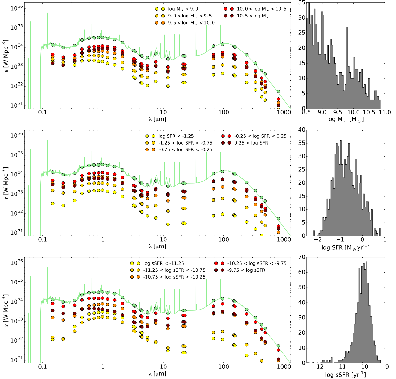
Figure 2. The contributions of galaxies with different properties to the EAGLE-SKIRT CSED: stellar mass (top row), star formation rate (middle row), and specific star formation rate (bottom row). The right-hand panel on each row shows the histogram of the relevant quantity for the EAGLE-SKIRT sample. The left-hand panel shows the contributions of five different bins to the total EAGLE-SKIRT CSED.
