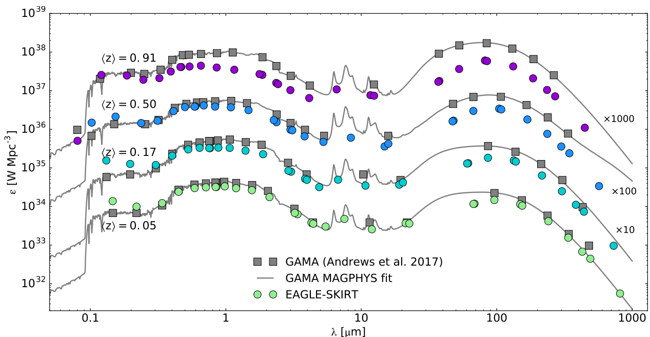
Figure 5. The evolution of the CSED between z = 0 and z = 1 . As in Figure 1, the grey squares and solid grey lines are the GAMA broadband observations and best fitting MAGPHYS SED models from Andrews et al. (2017b). The four different lines correspond to four different redshifts bins (as indicated on the left), and they have been shifted vertically for the sake of clarity. The coloured dots are the EAGLE-SKIRT CSED at the same mean redshifts.
