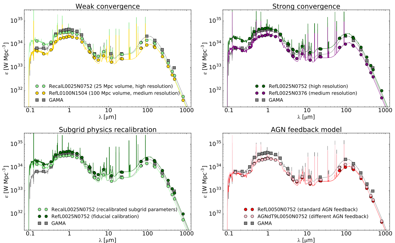
Figure 3. A comparison of the CSED corresponding to different EAGLE runs. The models used are indicated in each panel. As in Figure 1, the coloured dots are the broadband EAGLE-SKIRT CSED measurements, the solid grey squares are the broadband GAMA measurements from Andrews et al. (2017b), and the solid lines represent CIGALE fits through the simulated/observed data. For details on the different simulations, see Table 1.
