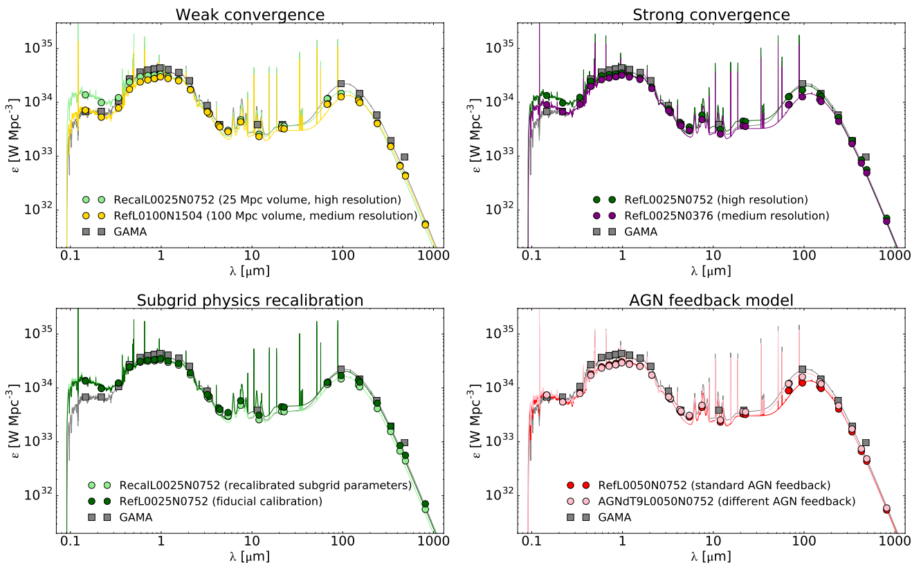
Figure 4. A comparison of the normalised CSED corresponding to different EAGLE runs. This figure is identical to Figure 3, except that the CSED in each panel is normalised to the stellar mass density of the RecalL0025N0752 simulation.
