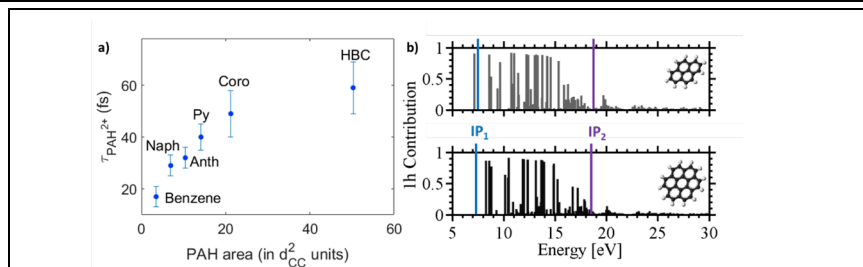
Fig. 2. a) Dication decay constant as a function of the PAH area (given in units of the distance between two adjacent carbon atoms, d_{\text{CC}} ); Benzene ( \text{C}_6\text{H}_6 ) is taken from [8]; b) Computed ADC spectra for Pyrene and Coronene, from Supplementary Material of [6].
