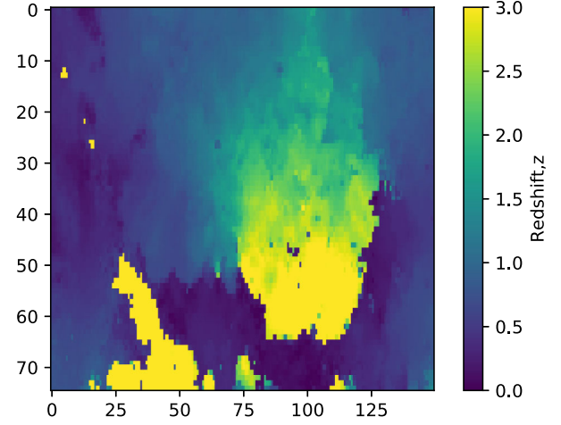
FIG. 1. The [8] self-organizing map. The color scale shows the mean photometric redshift per pixel. The axes are pixel labels that are arbitrarily defined.
