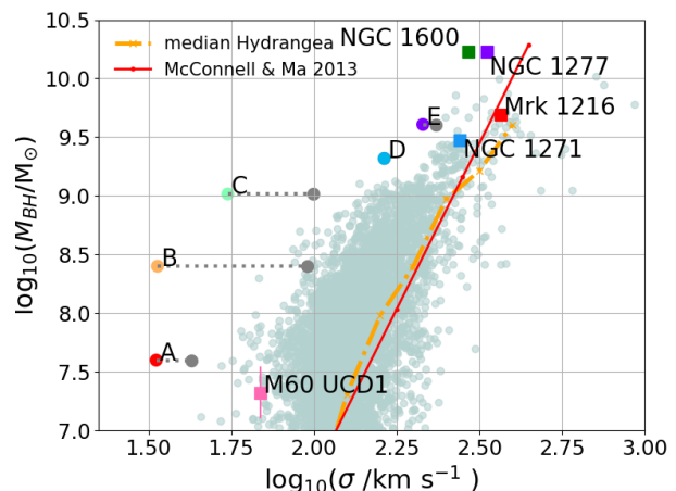
Figure 5. M_{\text{BH}} as a function of stellar velocity dispersion. The distribution for galaxies with \log_{10}(M_{\text{BH}}/M_{\odot}) > 7 at z = 0 is shown in gray-blue. The solid red line shows the empirical relation for early type galaxies from McConnell & Ma (2013), while the dash-dotted orange line displays the median of the Hydrangea sample. The Hydrangea BMGs are plotted at their z = 0 values (coloured circles). The re-computed stellar velocity dispersions are shown as gray circles connected to the original values by dotted gray horizontal lines.
