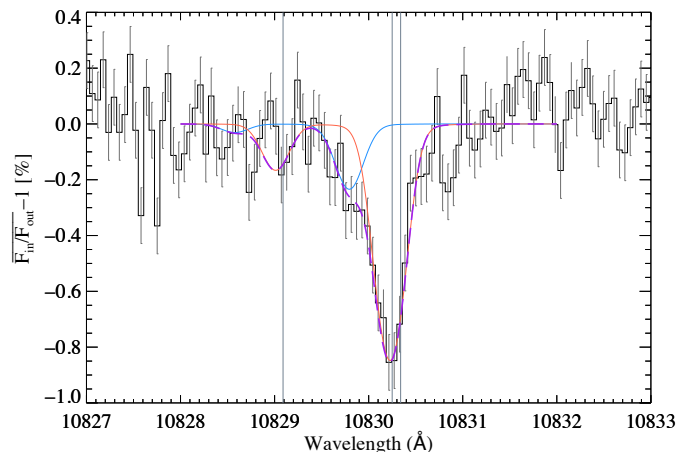
Fig. 4. Average transmission spectrum around the He I triplet in the planet rest-frame. The positions of the three helium lines are marked by vertical lines. The red curve is the best-fit Parker wind model obtained for a temperature of 6000 K and a mass-loss rate of 4.2 \times 10^9 \text{g s}^{-1} . The blue line indicates a model for a tentative blueward component centred at around -13 \text{km s}^{-1} . The magenta dashed curve is the combination of the red and blue lines.
