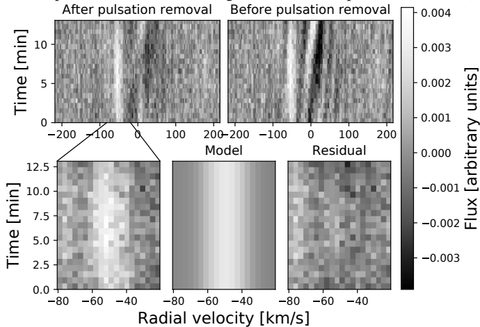
(b) Exoplanet candidate for the night of UT 2017 Dec 11 (JD = 2458098).
