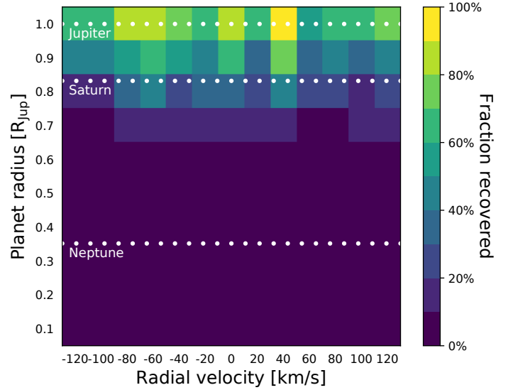
Fig. 5: Recovery fraction of 152 transit injections into the \beta Pictoris dataset. Exoplanet signals with a SNR > 3.0 above other nights are considered recovered. We assume an impact parameter b = 0 . The radii of Jupiter, Saturn and Neptune are indicated by the white dashed lines. As v_{\text{eq}} = 130 km/s, radial velocities outside of our range are (close-to) zero. Companions with radii R = R_{\text{Jup}} are almost fully recovered and a large fraction with radii R = R_{\text{Sat}} are recovered. The effects of stellar pulsation are seen by the fluctuations of the recovery fraction as a function of radial velocity.
