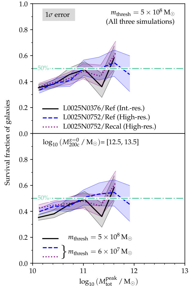
Figure B1. Survival fraction of satellites in low-mass groups in three (25 \text{ cMpc})^3 simulations from the EAGLE project. L0025N0376/Ref (black solid line) uses the same resolution as the Hydrangea simulations analysed in the main part of this paper, while the other two (blue dashed and purple dotted lines, corresponding to different choices of subgrid parameters) have eight times better mass resolution. In the top panel, the same survival threshold ( 5 \times 10^8 M_{\odot} ) is applied to all three, while the bottom panel uses an eight times lower threshold for the higher-resolution simulations. In the first case, the higher resolution has no impact, but with a lower mass threshold the fraction of surviving galaxies increases slightly at the low-mass end.
