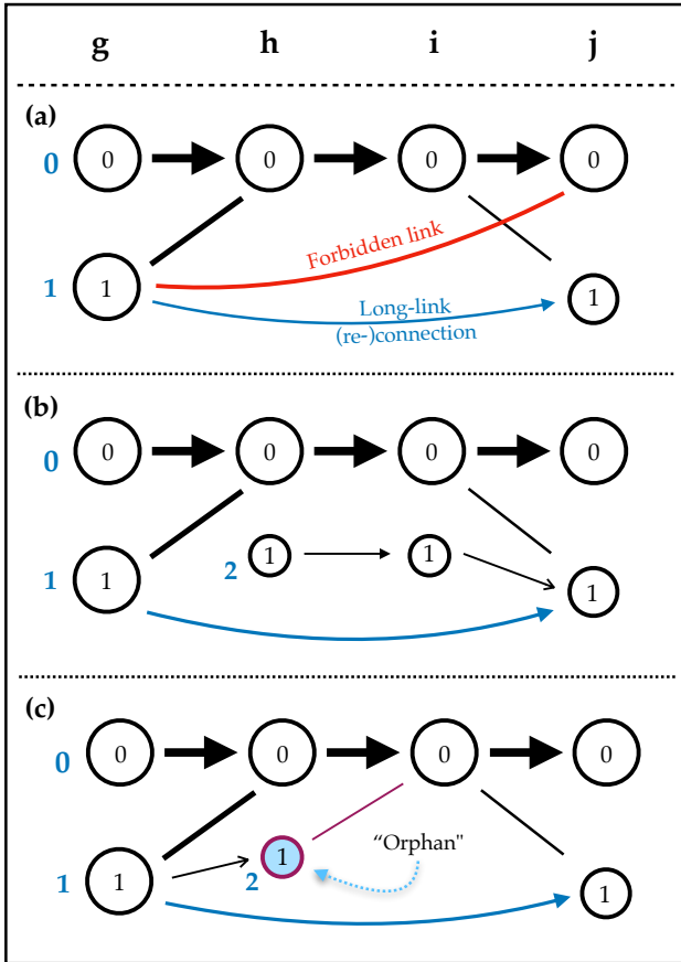
Figure A7. Three example situations involving the re-connection of subhaloes via long-links. Panel a ( top ) depicts the simplest case in which a subhalo without descendant ( g_1 ) is re-connected to a subhalo without progenitor ( j_1 ). As described in the text, link g_1-j_0 is forbidden because it would invert the survival order established in snapshot h . Panel b ( middle ) illustrates a long-link connection that ‘overrides’ a (weaker) direct link from galaxy 2 (subhalo i_1 ). Panel c ( bottom ) shows a case in which an originally identified descendant ( h_1 ) is disconnected and turned into an ‘orphan’ that is only alive in one snapshot, because the long-link g_1-j_1 allows the continued tracing of galaxy 1 to snapshot j .
