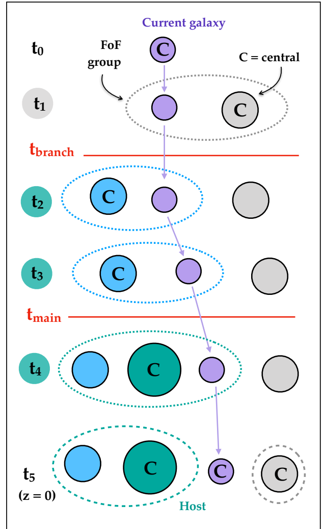
Figure 1. An illustration of our host assignment scheme. Shown are six consecutive snapshots at times t_0 to t_5 (the latter corresponding to z = 0 ). Coloured circles represent four individual galaxies, of which the purple one is currently under consideration. Although it is a central at redshift z = 0 , it was a satellite in four previous snapshots ( t_1 – t_4 ), with the respective groups outlined by dotted ellipses. Their centrals lie in two FoF groups at z = 0 , indicated by the grey and green dashed ellipses in the bottom row. These are the two candidate hosts of the galaxy, and the shading behind each snapshot label (on the far left) indicates to which one it was associated at this point. Because it is associated most often to the green candidate, this is selected as the galaxy’s host. The two horizontal red lines indicate the two accretion times used in this paper, corresponding to first infall into the host itself ( t_{\text{main}} ) and one of its progenitor branches ( t_{\text{branch}} ).
