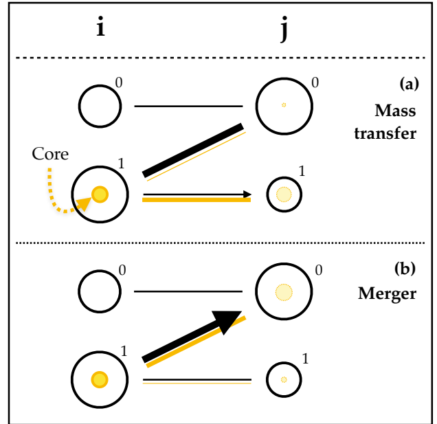
Figure A2. Identification of mass transfer by considering subhalo cores. Black circles represent two subhaloes each in two successive snapshots i and j . The total particle overlap between them, as indicated by the width of the connecting black lines, is identical in the top and bottom configurations and could be interpreted as either mass transfer or a merger. The small yellow circle in subhalo i_1 represents its most bound ‘core’ particles. As indicated by the yellow lines, these transfer differently in the two scenarios: under mass transfer (top), they remain mostly within their own galaxy and end up in j_1 (as indicated by the faint yellow circles in the j subhaloes), but in a merger they end up (mostly) in subhalo j_0 .
