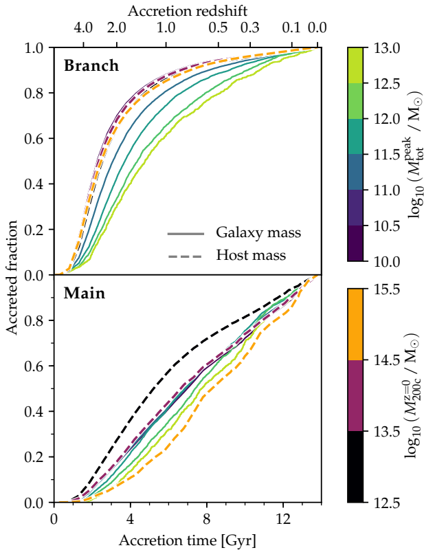
Figure 2. Cumulative distribution of accretion times for different peak total galaxy masses (solid lines) and different host halo masses (dashed lines) in the hydrodynamical simulations. Top: accretion onto any branch of the host group ( t_{\text{branch}} ). Bottom: accretion onto its main progenitor branch ( t_{\text{main}} ), for galaxies with t_{\text{main}} < \infty . Values of t_{\text{branch}} are predominantly early (around z \approx 2 ), while t_{\text{main}} is more evenly spread out. The former depend mostly on galaxy mass, the latter on host mass.
