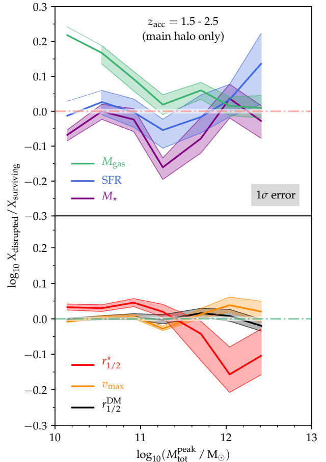
Figure 14. Top panel: bias of disrupted galaxies in baryonic properties prior to accretion, compared to surviving galaxies (at a mass threshold of 5 \times 10^8 M_{\odot} for survival). Stellar mass is shown in purple, star formation rate in blue, and gas mass in green. Only galaxies directly falling into their final host between z = 2.5 and 1.5 are shown to avoid indirect biases due to different accretion times. Only bins with at least ten surviving and disrupted galaxies are shown. At fixed M_{\text{tot}}^{\text{peak}} , disrupted galaxies had slightly higher gas mass, and slightly lower stellar mass, than surviving galaxies. Bottom panel: the same for DM half-mass radius (black), stellar half-mass radius (red), and maximum circular velocity (orange). Out of these, only the stellar half-mass radius shows a significant (but relatively small) difference between disrupted and surviving galaxies.
