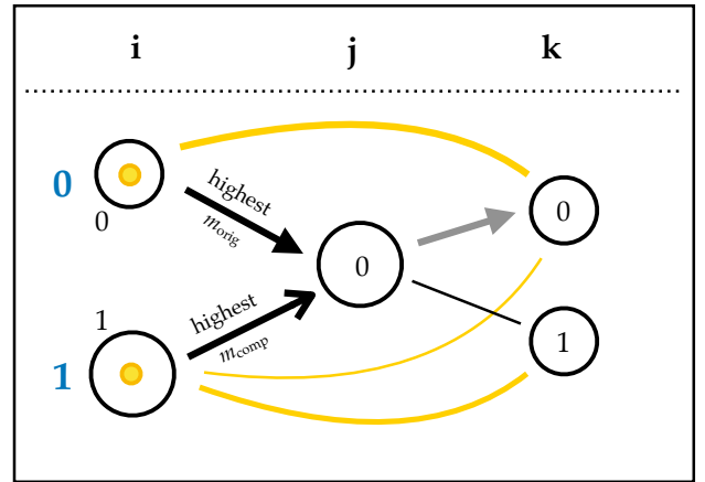
Figure A6. Decision between ambiguous progenitors. Subhalo j_0 could be the descendant of i_0 (which contributes the largest amount of mass, m_{\text{orig}} ) or i_1 (whose mass contribution adjusted for prior exchanges, m_{\text{comp}} , is greatest). In the following snapshot ( k ), k_0 is the likely descendant of j_0 , but only i_0 sends most of its core particles to this subhalo. The progenitor of j_0 is therefore chosen to be i_0 (continuing galaxy 0), while galaxy 1 is merged (and will likely be re-connected to k_1 in the next snapshot, as described in Section A5). Under all other circumstances, i_1 would be selected as the progenitor of j_0 .
