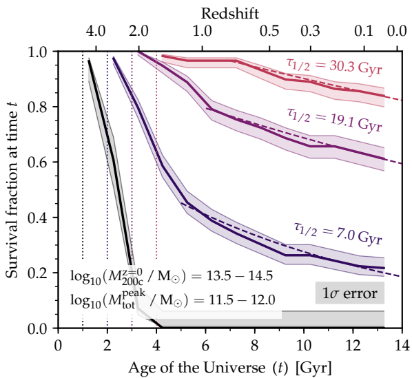
Figure 12. Connection between accretion and disruption time for one bin in galaxy and host mass (see bottom-left corner) in the hydrodynamical simulations. We select galaxies that were accreted within 4 intervals of \Delta t = 500 Myr, centered on the times indicated by vertical dotted lines, and show their survival fraction (above a total mass threshold of 5 \times 10^8 M_{\odot} ) as a function of time. Thin dashed lines represent the best-fit late-time exponential decay model, with corresponding half-life time \tau_{1/2} as indicated on the right. The earliest-accreted galaxies have all disrupted rapidly after accretion. Later generations show a progressively shallower decline in survival fraction, with \tau_{1/2} \gg t_{\text{Hubble}} at z_{\text{acc}} < 2 .
