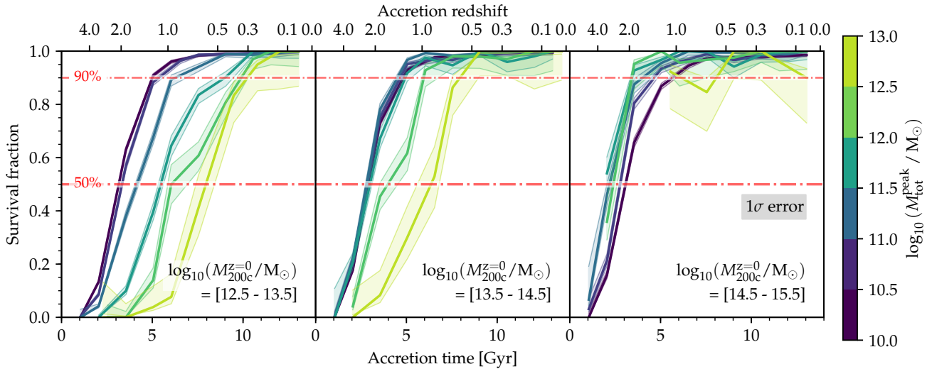
Figure 11. The fraction of non-pre-processed galaxies accreted at a given redshift ( z_{\text{acc}} ) that survive to z=0 (with M_{\text{tot}}^{z=0} > 5 \times 10^8 M_{\odot} ), in the hydrodynamical simulations. Only bins with at least ten galaxies are shown, which is why not all lines extend to the earliest accretion times. Different panels show different host mass ranges, as indicated in the bottom-right corners. In all three panels, the survival fraction of low-mass galaxies approaches unity for galaxies accreted at z_{\text{acc}} \lesssim 1 , and then drops rapidly towards earlier accretion times. More massive galaxies, and those in less massive groups, are still disrupted at lower z_{\text{acc}} .
