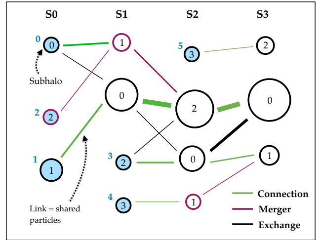
Figure A1. Example tracing situation with 14 subhaloes (circles with inscribed number representing their arbitrary ID and size indicating their mass) in 4 snapshots S0–S3 (different columns). Lines represent links, i.e., particle overlaps between subhaloes, whose width scales with link particle number (for simplicity assuming that all particles have equal mass). Green lines represent links that connect successive subhaloes of the same galaxy. The first subhalo of each galaxy is shaded blue, with a number to the left indicating the (arbitrary) galaxy ID. Purple circles indicate the last subhalo of a galaxy about to disrupt/merge, with the corresponding purple link pointing to the galaxy's carrier in the next snapshot. Black lines represent exchange links between galaxies.
