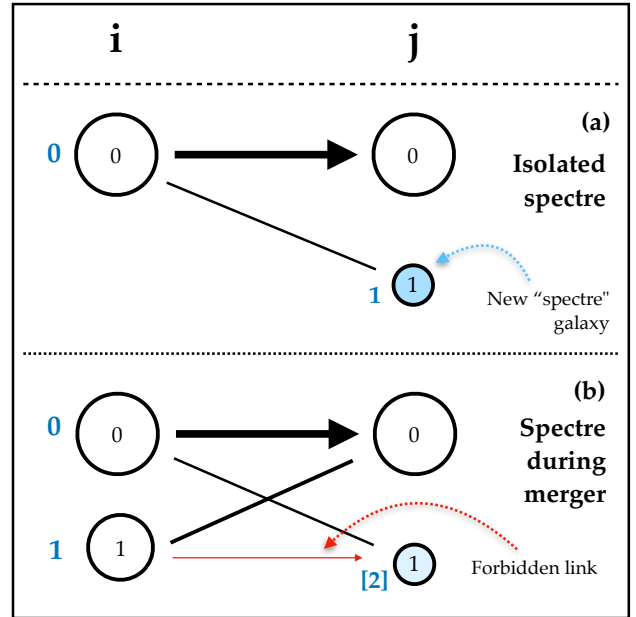
Figure A5. Exclusion of links to prevent connections to spurious ‘spectre’ galaxies. Top: formation of a spectre in isolation, which is easily identified as a new galaxy. Bottom: when a spectre forms at the same time as a merger, it may be mis-identified as the descendant of the merging galaxy (1). The link i_1-j_1 is therefore marked as forbidden.
