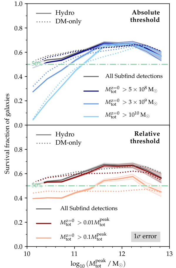
Figure 5. Dependence of satellite survival fractions on the imposed detection threshold in the hydrodynamical (solid lines) and DM-only simulations (dotted lines) of massive clusters. Grey lines show the total survival fraction, i.e., all galaxies detected by SUBFIND at z = 0 . In the top panel , the dark, medium, and light blue lines show, respectively, the fraction of galaxies retaining a total mass of at least 5 \times 10^8 , 3 \times 10^9 , and 10^{10} M_{\odot} , respectively, at z = 0 . The bottom panel gives the fraction of galaxies that retain at least 1 (dark red) and 10 per cent (light red) of their total peak mass at z = 0 . All thresholds apart from this last one converge in the hydrodynamic simulations at M_{\text{tot}}^{\text{peak}} > 3 \times 10^{11} M_{\odot} . In contrast, many lower-mass galaxies – and in the DM-only simulations even some Milky Way analogues – only survive as low-mass remnants below 10^{10} M_{\odot} .
