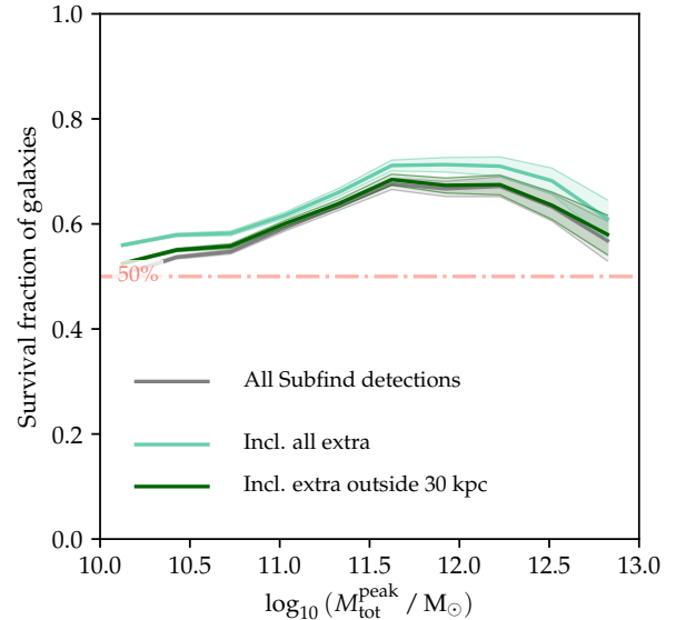
Figure B2. Fraction of galaxies in massive clusters ( M_{200c}^{z=0} > 10^{14.5} M_\odot ) that survive to z = 0 . The grey line includes all galaxies present in the SUBFIND catalogue. The light green line adds galaxies which retain a self-bound remnant with at least ten particles when starting from all particles that are part of the galaxy in its last snapshot. The dark green line limits those recovered detections to only those that lie away from subhaloes in the SUBFIND catalogue (see text for details). There is no significant population of surviving galaxies that is missed by SUBFIND, particularly with the more restrictive definition (dark green).
