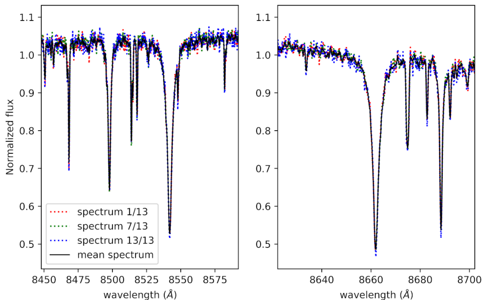
Fig. 4. Same as Fig. 3 except for the region around the Ca + infrared triplet lines used in this analysis.
