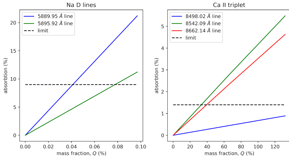
Fig. 9. Absorption by the Na D lines (left) and the Ca + triplet (right) as a function of fraction of available lost mass that becomes absorbing gas, assuming a dust-mass loss rate of 2 \times 10^{11} \text{ g s}^{-1} , Earth crust abundances and absorption lifetimes equal to the photoionization lifetimes of 1.8 \times 10^3 \text{ s} and 1.1 \times 10^3 \text{ s} , respectively.
