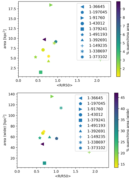
Figure 17. The total size of the likely quenching regions as a function of their average distance ( R/R_{50} ) from the galactic centre of the QG galaxies. In the top panel we consider only the regions that satisfied our quenching criteria, while in the bottom panel we consider the area comprising the plausible quenching regions and the less extreme adjacent areas. The symbols represent different galaxies, while the colour represents the percentage of spaxels in the area with respect to the whole spaxels of the galaxy.
