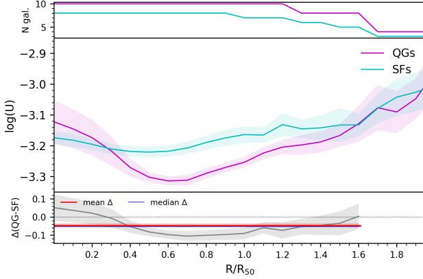
Figure 13. The average radial profiles of \log U for QG and SF samples. The layout of the figure is the same as in Figure 10.
