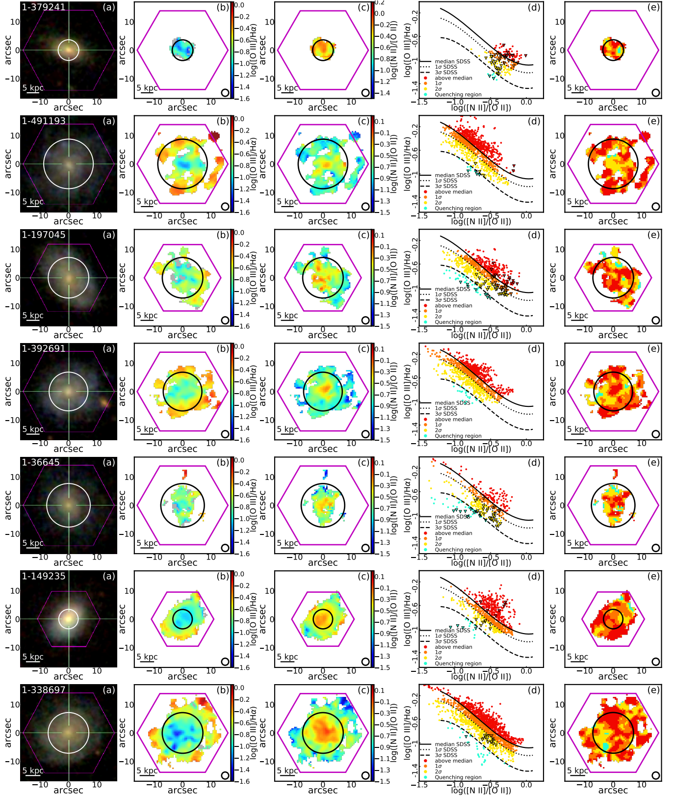
Figure 2. A summary of the 10 QG galaxies in our sample. (a) The g-r-i images composite from SDSS. Each image covers a region of 17 \times 17 \text{ arcsec}^2 and in the bottom-left corner of each image is reported the scale of 5 kpc. (b) The dust-corrected [\text{O III}]/\text{H}\alpha maps. The grey areas show regions with \text{S/N}([\text{O III}]) < 2 . (c) The dust-corrected [\text{N II}]/[\text{O II}] maps. (d) The [\text{O III}]/\text{H}\alpha vs [\text{N II}]/[\text{O II}] diagnostic diagram for the quenching. The spaxels are colour-coded according to their position on the plane: red dots for those lying above the median curve, orange dots for them between the median and 1\sigma , yellow dots for spaxels which lie between 1\sigma and 3 \times 1\sigma and, finally, cyan dots for spaxels below the 3 \times 1\sigma curve that, according with our classification criteria described in the text, represent likely quenching regions. The triangles represent spaxels with an upper limit in [\text{O III}]/\text{H}\alpha (i.e. spaxels with \text{S/N}([\text{O III}]) < 2 ). (e) The map of the galaxies colour-coded according to the position of spaxels as in (d). In (a), (b), (c) and (e) the overlapped-magenta hexagonal shapes the MaNGA IFU bundles, while the circle represents the R_{50} . Finally, the 2.5'' circle in the bottom-right corner of the maps in (b), (c) and (e) represent the typical PSF (FWHM) of MaNGA data.
