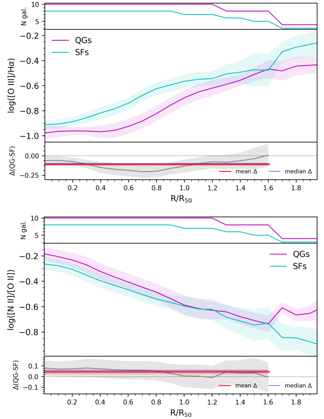
Figure 12. The average radial profiles of dust-corrected [\text{O III}]/\text{H}\alpha ( top ) and [\text{N II}]/[\text{O II}] ( bottom ) for QG and SF samples. The layout of the figure is the same as in Figure 10.
