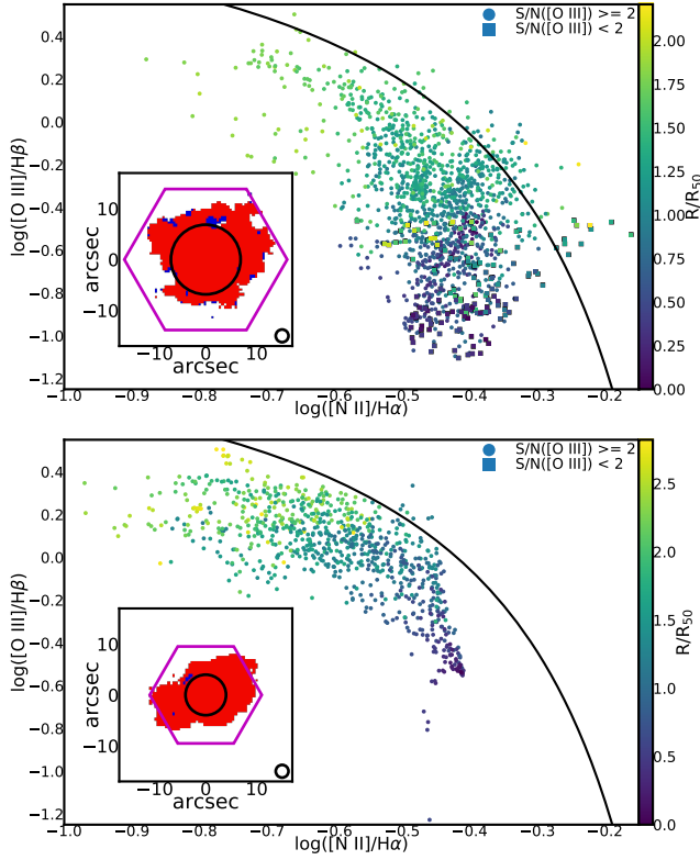
Figure 8. The resolved BPT diagram of QG 1-43012 ( top ) and of SF 1-178443 ( bottom ). Each round dot represents a spaxel in which the S/N([O\ III]) \geq 2 , while the square dots represent spaxels in which the S/N([O\ III]) < 2 and their [O\ III]/H\alpha values are upper-limits. The colours of the dots change according to the distance R/R_{50} of the spaxels from the centre of the galaxy. The black curve is from Kauffmann et al. (2003). The coloured maps represent the resolved BPT maps of the two galaxies. Spaxels with ionisation dominated by star formation (below the Kauffmann et al. (2003) curve) are represented in red, while those whose the ionisation is dominated by AGN/LINERs radiation are represented in blue. Overlapped is the hexagonal shape of the MaNGA IFU bundle, while the circle represents the R_{50} . The 2.5'' circle in the bottom-right corner of the maps represent the PSF (FWHM) of MaNGA datacubes.
