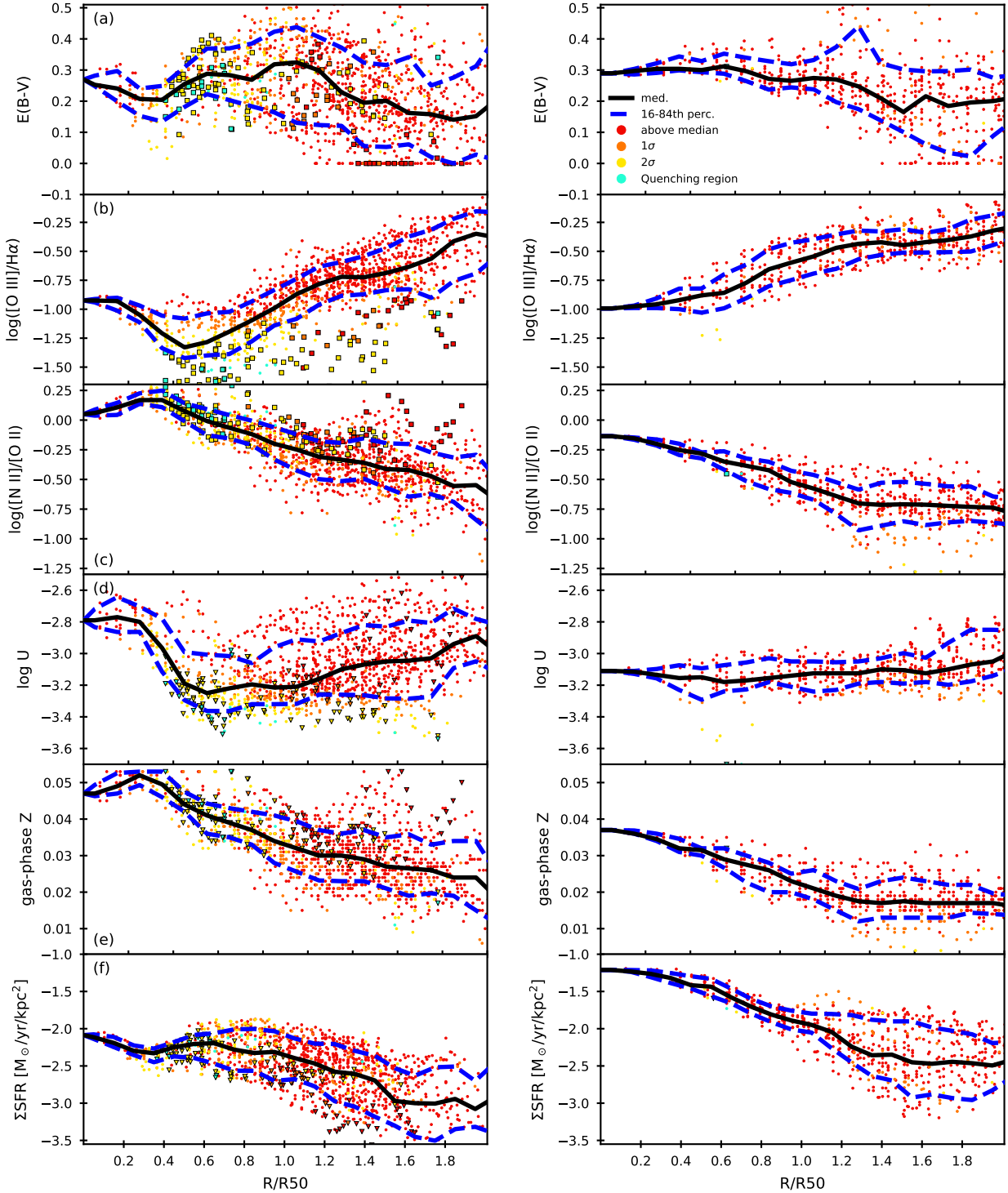
Figure 9. Radial profiles of QG 1-43012 ( left ) and of SF 1-178443 ( right ): (a) E(B-V) , (b) dust-corrected [\text{O III}]/\text{H}\alpha , (c) dust-corrected [\text{N II}]/[\text{O II}] , (d) \log U , (e) gas-phase Z , (f) \Sigma\text{SFR} . The black curves represent the median of the relations in bins of width 0.1R/R_{50} , while the blue ones represent the 16-84 th percentile of the relations. Each round dot represents a spaxel in which the S/N([\text{O III}]) \geq 2 , while the square dots represent spaxels in which the S/N([\text{O III}]) < 2 and their [\text{O III}]/\text{H}\alpha values are upper-limits. The dots colour code is the same as in Figure 7, and it is based on the position of each spaxel on the [\text{O III}]/\text{H}\alpha vs [\text{N II}]/[\text{O II}] diagram (Figure 1 and Figure 6). The cyan is representing quenching regions, followed by the yellow for the galactic regions that lie between 3 \times 1\sigma and 1\sigma of the diagram, orange for those between 1\sigma and the median and red for regions of pure star-formation that are above the median of the diagram.
