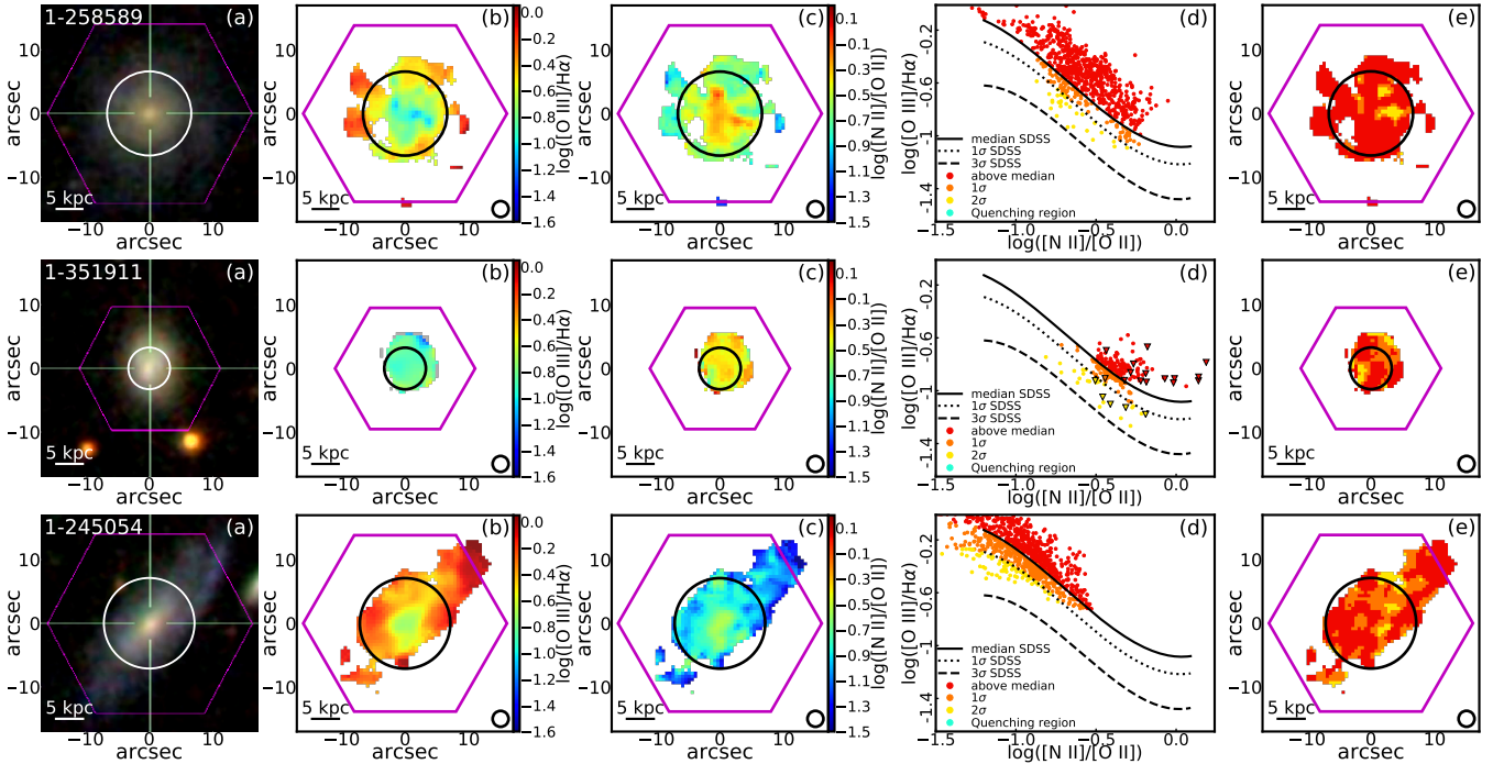
Figure 3. A summary of the 8 SF galaxies in our sample. (a) The g-r-i images composite from SDSS. Each image covers a region of 17 \times 17 arcsec 2 and in the bottom-left corner of each image is reported the scale of 5 kpc. (b) The dust-corrected [\text{O III}]/\text{H}\alpha maps. The grey areas show regions with \text{S/N}([\text{O III}]) < 2 . (c) The dust-corrected [\text{N II}]/[\text{O II}] maps. (d) The [\text{O III}]/\text{H}\alpha vs [\text{N II}]/[\text{O II}] diagnostic diagram for the quenching. The spaxels are colour-coded according to their position on the plane: red dots for those lying above the median curve, orange dots for those between the median and 1\sigma , yellow dots for spaxels which lie between 1\sigma and 3 \times 1\sigma and, finally, cyan dots for spaxels below the 3 \times 1\sigma curve. The triangles represent spaxels with an upper limit in [\text{O III}]/\text{H}\alpha (i.e. spaxels with \text{S/N}([\text{O III}]) < 2 ). (e) The map of the galaxies colour-coded according to the position of spaxels as in (d). In (a), (b), (c) and (e) the overlapped-magenta hexagonal shapes the MaNGA IFU bundles, while the circle represents the R_{50} . Finally, the 2.5'' circle in the bottom-right corner of the maps in (b), (c) and (e) represent the typical PSF (FWHM) of MaNGA data.
