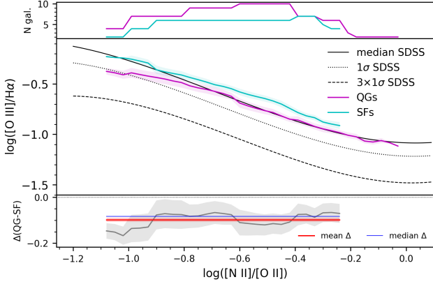
Figure 10. The average dust-corrected [\text{O III}]/\text{H}\alpha vs [\text{N II}]/[\text{O II}] diagram for the QG and SF samples. Top : the number N of galaxies that contribute to the average. Centre : The magenta curve represents the mean curve of the QG galaxies, that we obtain by averaging their means; the magenta shaded area shows the error of the average (i.e. \sigma_{\text{mean}}/\sqrt{N} ). The cyan curve shows the mean curve of the SF sample. The black curves represent median, 1\sigma and 3\times 1\sigma limit of the SDSS star-forming galaxies sample (see Q18). Bottom : the grey curve represents the differences in [\text{O III}]/\text{H}\alpha , as a function of [\text{N II}]/[\text{O II}] , between QGs and SF galaxies and the grey shaded area shows the propagated errors. The red line and pink shaded area represent the weighted mean and error of these differences averaged over the [\text{N II}]/[\text{O II}] range (see Table 2).
