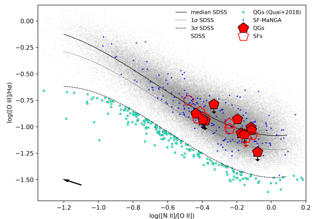
Figure 1. The diagnostic [\text{O III}]/H\alpha vs [\text{N II}]/[\text{O II}] diagram. The black curves represent median, 1\sigma and 3 \times 1\sigma limits of the SDSS star-forming galaxies sample (see Q18), which are represented by grey dots. The black arrow in the bottom-left corner represents the direction of the dust vectors for the Calzetti et al. (2000) extinction law, for an E(B-V) = 0.3 . The cyan squared dots below the 3 \times 1\sigma limits represent the SDSS quenching candidates selected in Q18. The blue dots represent the SDSS galaxies that have a match in MaNGA-DR14. The red pentagons represent the SDSS position of the MaNGA galaxies analysed in this paper: full symbols for the galaxies with quenching regions (QRG) and empty symbols for the star forming (SF) galaxies, as defined in subsection 2.5. The arrows indicate galaxies with the upper limits in [\text{O III}]/H\alpha .
