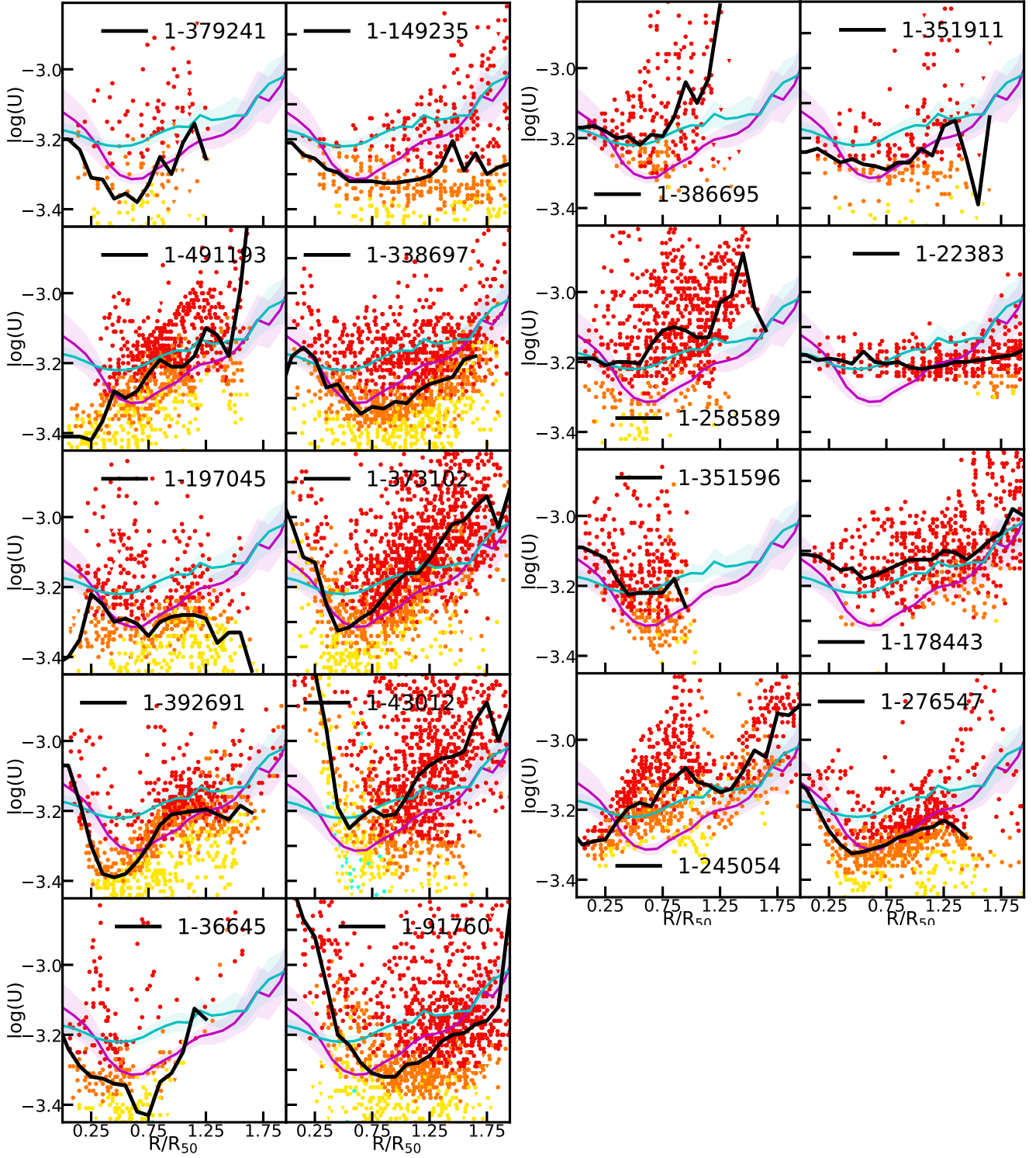
Figure A3. Radial profiles of ionisation parameter \log(U) of each galaxy belonging to QG sample (left) and to SF sample (right). See Figure A1 for panels description.
