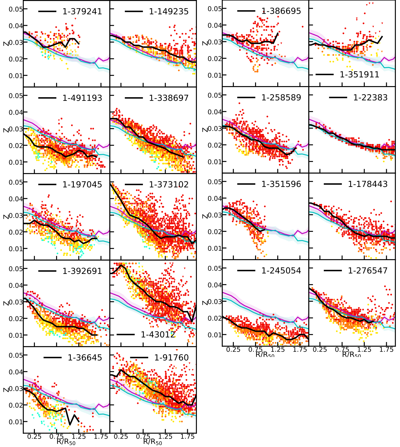
Figure A4. Radial profiles of gas phase metallicity Z of each galaxy belonging to QG sample (left) and to SF sample (right). See Figure A1 for panels description.
