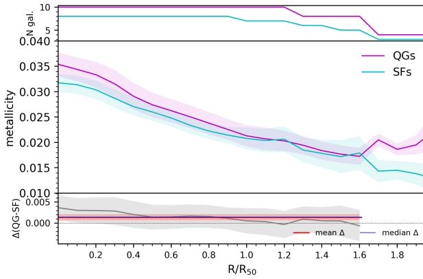
Figure 14. The average radial profiles of the gas-phase metallicity Z for QG and SF samples. The layout of the figure is the same as in Figure 10.
