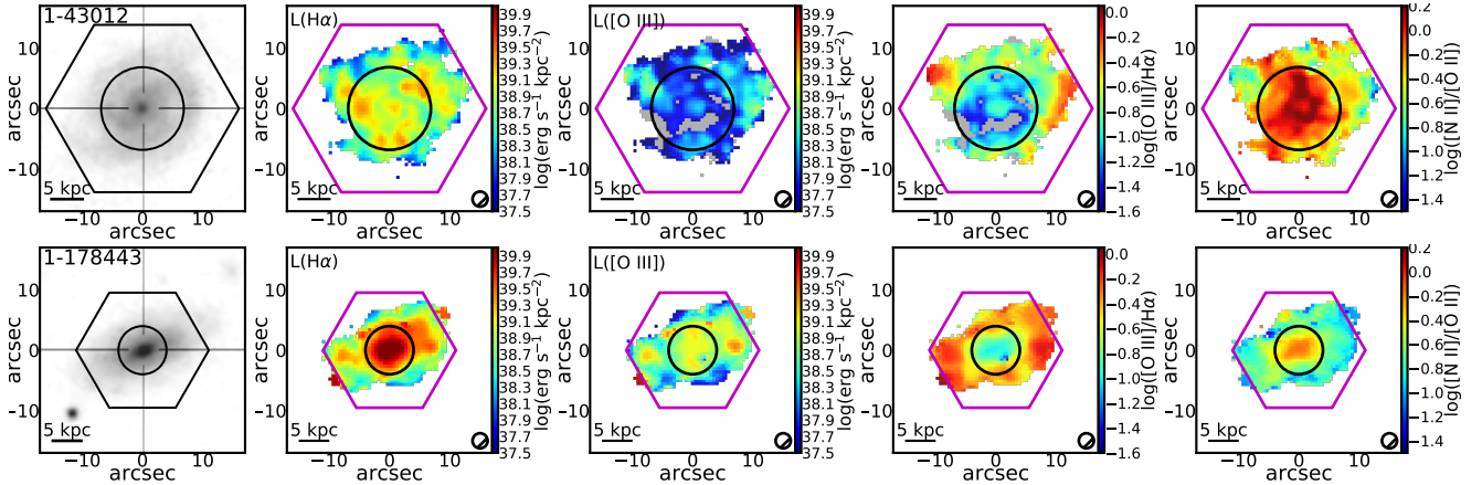
Figure 5. Spatially resolved maps of the two case galaxies. Each row shows maps of QG 1-43012 (top) and maps of SF 1-178443 (bottom). Each column shows, from left to right (1) r-band images (2) luminosity surface density maps of dust-corrected H\alpha , (3) luminosity surface density maps of dust-corrected [O\ III] , (4) dust corrected [O\ III]/H\alpha maps and (5) dust corrected [N\ II]/[O\ II] maps. Spaxels coloured in grey represent regions with S/N([O\ III]) < 2 . Overlapped in magenta are the hexagonal shapes of the MaNGA IFU bundles, while the black circles represent the R_{50} . The 2.5'' circle in the bottom-right corner of the maps represent the PSF (FWHM) of MaNGA datacubes. The galaxies go over the edge of the IFU shape because of the effect of the dithering, resulting in a coverage of a larger area of the sky.
