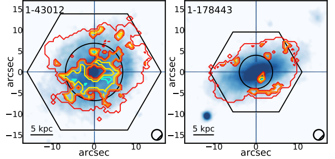
Figure 7. The contours of the resolved [\text{O III}]/\text{H}\alpha vs [\text{N II}]/[\text{O II}] diagram are superimposed to the G images (in false colours) of QG 1-43012 (left) and SF 1-178443 (right). The contours colour code is based on the position of each spaxel on the diagram, and it is the same as in Figure 1. The cyan is representing quenching regions, followed by the yellow for the galactic regions that lie between 3 \times 1\sigma and 1\sigma of the diagram, orange for those between 1\sigma and the median and red for regions of pure star-formation that are above the median of the diagram. In the bottom-left corner is reported the scale of 5 kpc. Overlapped are the hexagonal shapes of the MaNGA IFU bundles, while the circles represent the R_{50} . The 2.5'' circle in the bottom-right corner of the maps represent the PSF (FWHM) of MaNGA datacubes.
