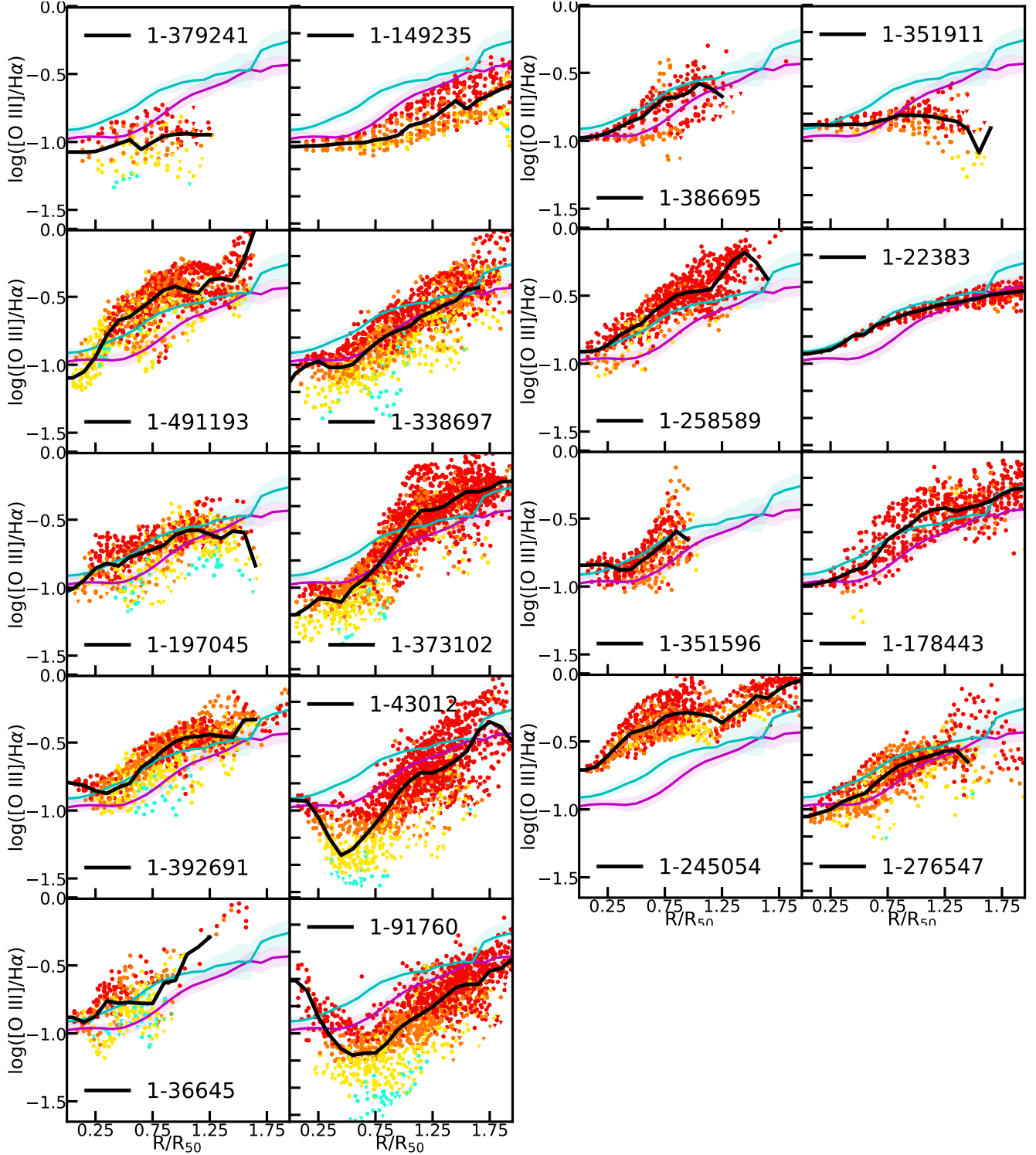
Figure A1. Radial profiles of [\text{O III}]/\text{H}\alpha ratio of each galaxy belonging to QG sample (left) and to SF sample (right). The black curves represent the median of the relations in bins of width 0.1R/R_{50} , while the blue ones represent the 16-84 th percentile of the relations. Each round dot represents a spaxel in which the \text{S/N}([\text{O III}]) \geq 2 , while the square dots represent spaxels in which the \text{S/N}([\text{O III}]) < 2 and their [\text{O III}]/\text{H}\alpha values are upper-limits. The dots colour code is the same as in Figure 7, and it is based on the position of each spaxel on the [\text{O III}]/\text{H}\alpha vs [\text{N II}]/[\text{O II}] diagram (Figure 1 and Figure 6). The cyan is representing quenching regions, followed by the yellow for the galactic regions that lie between 3 \times 1\sigma and 1\sigma of the diagram, orange for those between 1\sigma and the median and red for regions of pure star-formation that are above the median of the diagram. The magenta and cyan curves represent the average radial profiles of QG and SFs populations (as in Figure 11).
