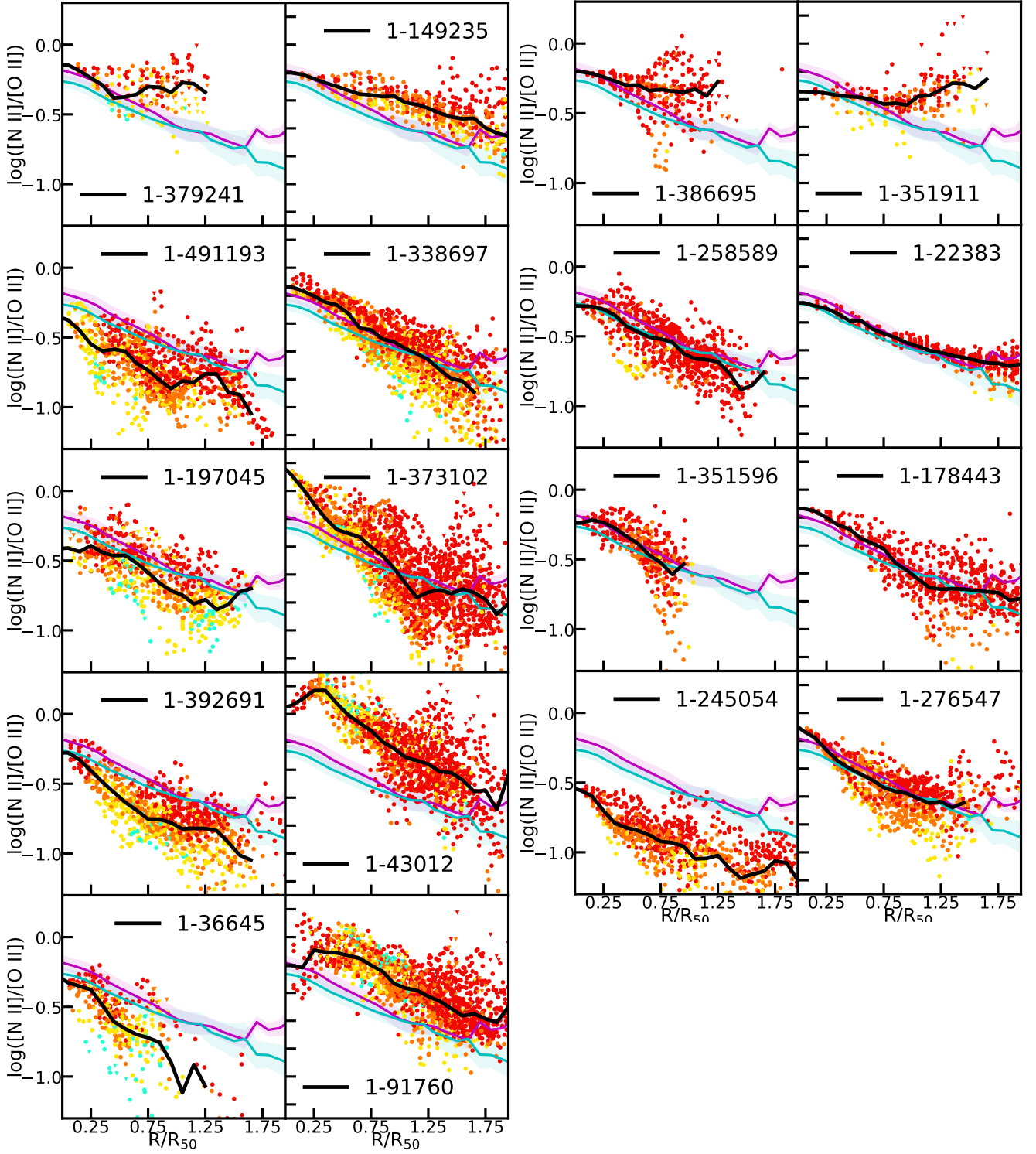
Figure A2. Radial profiles of [\text{N II}]/[\text{O II}] of each galaxy belonging to QG sample (left) and to SF sample (right). See Figure A1 for panels description.
