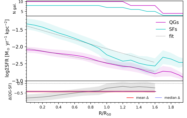
Figure 15. The SFR surface density ( \log \Sigma \text{SFR} ) radial profile for QG and SF samples. The dotted black lines represent the linear fit to the radial profiles. The layout of the figure is the same as in Figure 10.
