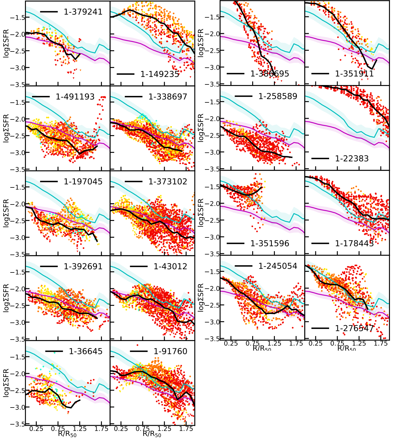
Figure A5. Radial profiles of the star formation rate surface density \Sigma\text{SFR} of each galaxy belonging to QG sample (left) and to SF sample (right). See Figure A1 for panels description.
