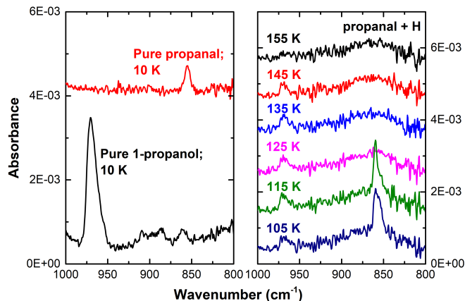
Fig. 5: (Left) Infrared features of pure propanal (exp. 2.3) and 1-propanol (exp. 2.0). (Right) RAIRS annealing series of propanal + H (exp. 2.1), taken after deposition at 10 K. Note that the features at 860\text{ cm}^{-1} and 969\text{ cm}^{-1} are signatures of propanal and newly formed 1-propanol (tentative), as the signatures disappear by 125 K (propanal peak desorption temperature) and 155 K (1-propanol peak desorption temperature), respectively. RAIR spectra are offset for clarity.
