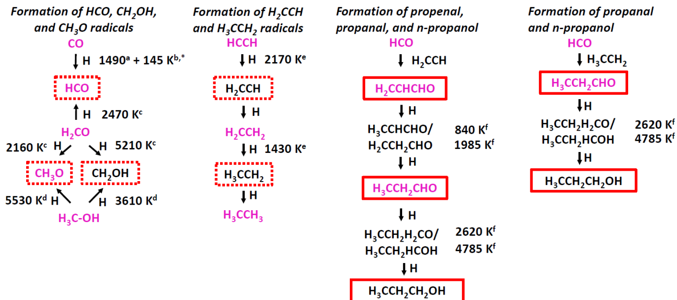
Fig. 6: Proposed mechanisms for exp. 1.0. Note that all radical-radical reactions shown here are barrierless. Relevant species within each mechanism are boxed; solid-line boxes indicate stable species and dotted-line boxes indicate radicals. Species labeled with purple font are those that have been detected in space. Activation energies are by a) Andersson et al. (2011) and b) Álvarez-Barcia et al. (2018) c) Song & Kästner (2017) d) Goumans & Kästner (2011) e) Kobayashi et al. (2017) and f) Zaverkin et al. (2018). * indicates the zero-point energy (ZPE) contribution.
