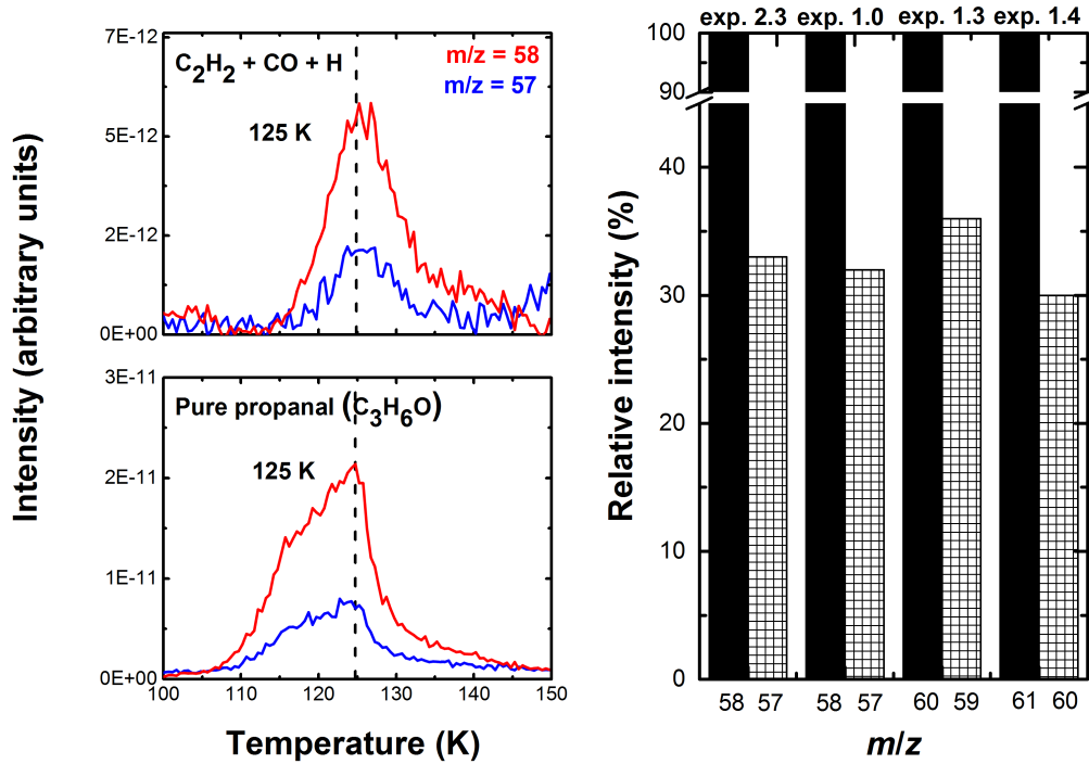
Fig. 2: (Left) TPD spectra of \text{C}_2\text{H}_2 + \text{CO} + \text{H} (top; exp. 1.0) and propanal (bottom; exp. 2.3) taken after deposition at 10 K. (Right) QMS fragmentation pattern of two m/z values that are normalized to the QMS signal of the \text{C}_3\text{H}_6\text{O}^+ ion (or the corresponding isotopologue) found in the propanal (exp. 2.3), \text{C}_2\text{H}_2 + \text{CO} + \text{H} (exp. 1.0), \text{C}_2\text{H}_2 + \text{C}^{18}\text{O} + \text{H} (exp. 1.3), and \text{C}_2\text{H}_2 + {}^{13}\text{C}^{18}\text{O} + \text{H} (exp. 1.4) experiments.
