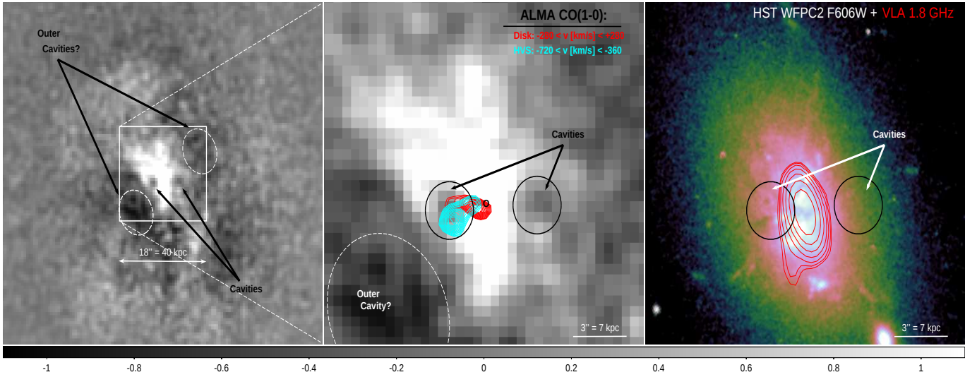
FIG. 5.— Left : Chandra residual flux image of A1664 after subtracting the sum of four freely-varying \beta -model fits, normalized by the flux image in the broad (0.5–7.0 keV) band, and binned such that one pixel is approximately 0.5'' on a side. The image is smoothed with a 2-pixel radius Gaussian kernel. The image highlights a cavity system in the X-ray emission with a set of arrows toward the center of the cluster, and another set of possible outer cavities. Middle : a zoomed-in view of the region of interest, smoothed with a 2-pixel radius Gaussian kernel. The ‘o’ marks the location of the BCG. The contours from the molecular CO emission measured by ALMA are overlaid, and are found just behind or inside the putative Eastern cavity. The systemic possible “disk” component and the high-velocity system (HVS) are described in detail in Russell et al. (2014). Right : HST WFPC2 F606W image of A1664 for comparison, from O’Dea et al. (2010), with JVLA 1.8 GHz contours overlaid (courtesy of A. C. Edge).
