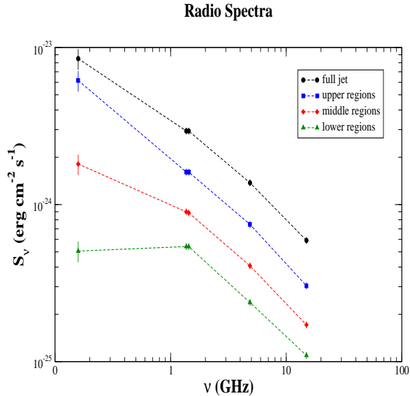
Figure 4. The radio spectrum measured over larger regions created merging those selected in previous multi-frequency analyses (Massaro et al. 2011) as described in § 3.2.
