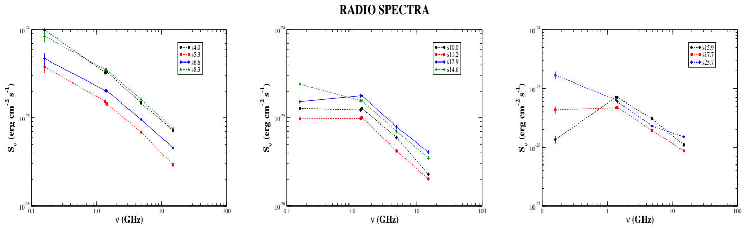
Figure 3. The radio spectra for 10 knots along the jet labeled following the nomenclature of Fig. 2 and that of the southern hotspot s25.7. We excluded from this figure the knot s2.1 but its radio flux density at low radio frequency is reported in Appendix together with all other radio extended components.
