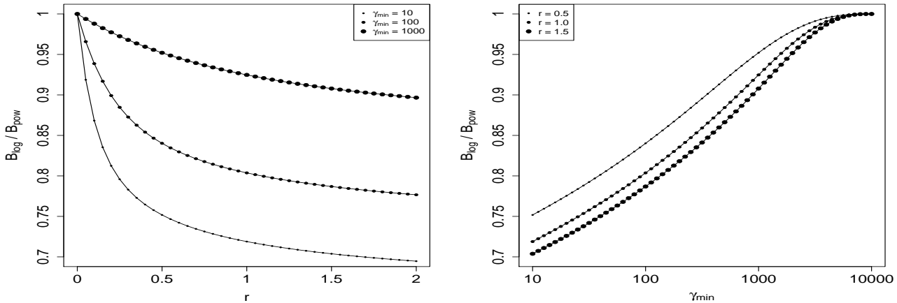
Figure 5. The ratio between the magnetic field strength estimated using a simple power-law vs a log-parabolic distribution as function of both the PED curvature r (left panel) and the minimum value of the Lorentz factor for the PED: \gamma_{\min} (right panel).
