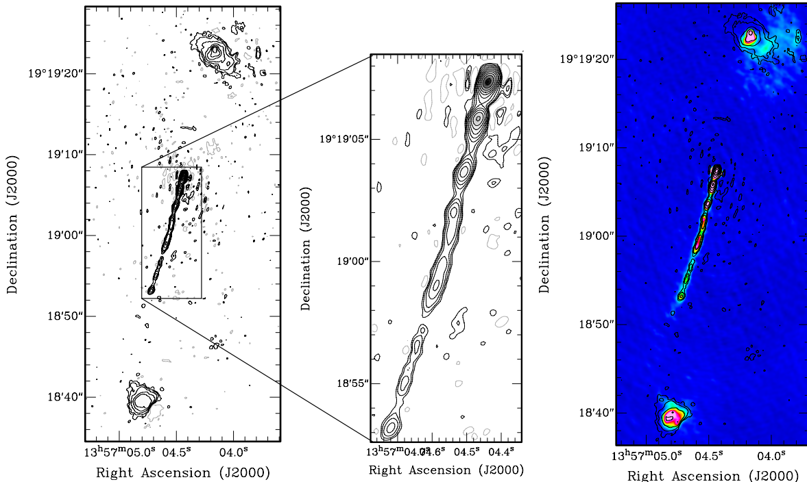
Figure 1. Left and center: LOFAR image of 4C+19.44 with zoom-in (center) of the jet. The contour levels are -0.0012 , 0.0012 to 1.5 in multiple of 2 . Right: The JVLA radio image of 4C+19.44 in C band with LOFAR radio contours overlaid. The image clearly shows how the radio structure observed at 159 MHz matches the morphology at GHz frequencies. Extended structures in the northern lobe are detected at larger significance in the JVLA image, but jet knots are detected in both images as we expected when selecting the target to carry out our experiment.
