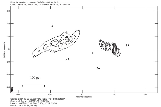
Fig. 2. VLBI continuum image at 2.3 GHz. The contour levels are 0.011 \times -0.864, 0.864, 1.729, 3.458, 6.916, 13.83, 27.66, 55.33 Jy beam -1 .
