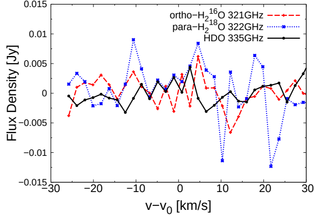
Figure 1. The observed flux densities around the line centers of the ortho- \text{H}_2^{16}\text{O} line at 321 GHz (red dashed line with cross symbols), the para- \text{H}_2^{18}\text{O} line (blue dotted line with filled square and cross symbols) at 322 GHz, and the HDO line at 335 GHz (black solid line with circle symbols) of the disk around HD 163296, with a velocity resolution dv = 1.9 \text{ km s}^{-1} . In obtaining the observed line flux densities, we adopted a circular aperture with radius 20 au.
