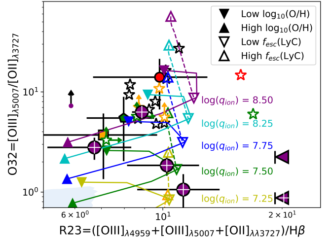
Figure 8. R23 vs O32 diagram, similar to Figure 6, however now we have zoomed into the upper-right region where highly ionized galaxies are found. With the exception of LCEs (white stars), individual galaxies in comparison samples have been removed for simplicity. Symbols common to both figures are the same as in Figure 6. The major addition in this Figure are photoionization modeling tracks output by the MAPPINGS V code. Solid lines show tracks for ionization bounded models of constant ionization parameter, q_{ion} (values shown in the annotated text with corresponding colours), with increasing 12 + \log_{10}(O/H) as indicated by the filled triangles. Dashed lines show tracks with increasing f_{esc}(\text{LyC}) , as indicated by the open triangles, at fixed q_{ion} and 12 + \log_{10}(O/H) . These models clearly show the three-fold degeneracy between q_{ion} , 12 + \log_{10}(O/H) , and f_{esc}(\text{LyC}) in the observed R23-O32 space.
