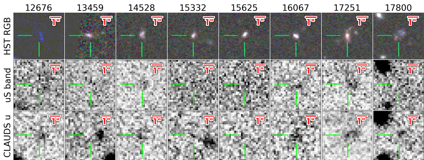
Figure 2. Top: RGB images for our selected galaxies produced using HST F160W, F125W and F814W filters (galaxy 12676 only has coverage in F814W). HST imaging shows galaxies in our sample to be elongated, nonsymmetric, and/or exhibiting multiple continuum peaks. These features may be indicative of ongoing mergers; however, we cannot fully rule out the possibility of low redshift, line-of-sight companions. Although there is no evidence from our MOSFIRE spectra of such companions, this possibility will affect our selection, and we discuss the implications of this in Section 6.2 Middle: CFHTLS uS images of our galaxy sample. Bottom: CLAUDS u band images of our galaxy sample that are used in estimating f_{esc}(LyC) in Section 4.4.
