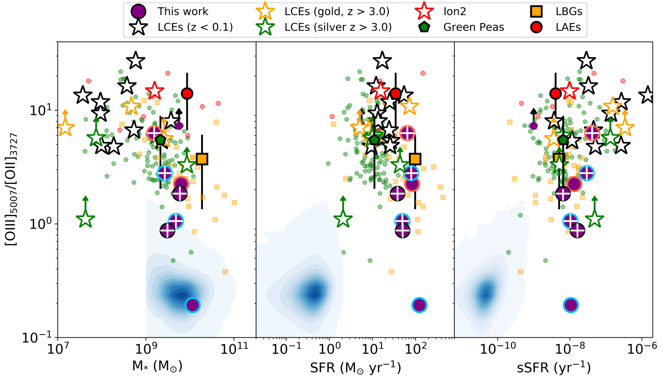
Figure 9. O32 as a function of M_* , SFR, and sSFR for galaxies in our MOSFIRE sample as well as low and high redshift comparison samples. Plotted symbols are the same as in Figure 6. Purple circles with blue borders indicate the three galaxies having u -band flux consistent with f_{esc}(\text{LyC}) > 0.0 as estimated in Section 4.4. The two purple circles with red borders indicate galaxies where upper limits on u -band flux provide non-zeros upper limits on f_{esc}(\text{LyC}) . The remaining three purple circles are galaxies where f_{esc}(\text{LyC}) is consistent with zero even within the photometric uncertainty. Galaxies in our sample have M_* comparable to low mass LBGs and high mass green peas, though up to 1 dex more massive than confirmed high- z LCEs. These results are likely reflective of relatively high stellar mass limits imposed for reliable photometric detections at high redshift (i.e. our desire to target bright galaxies). SFRs of our sample are comparable to LBGs, which are typically more star forming than green peas and LCEs. Finally, in terms of sSFR, galaxies in our sample are quite similar to confirmed LCEs.
