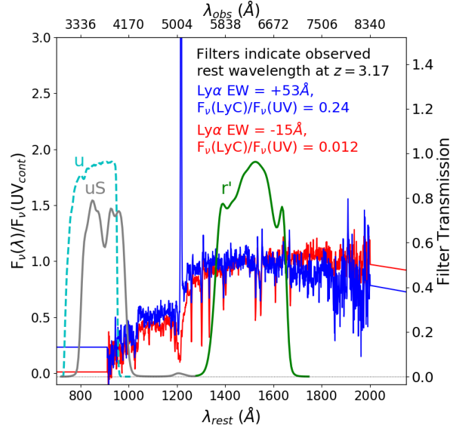
Figure 1. Composite Lyman break galaxy (LBG) spectra from Shapley et al. (2003) demonstrating contribution from LyC photons in the u band. In blue and red we show the stacked spectra for the highest and lowest quartiles in Ly \alpha EW from LBGs in Shapley et al. (2003) , respectively. Raw transmission curves for CFHTLS uS and r' filters are shown with wavelength coverage indicating the observed restframe wavelengths for galaxies at a redshift of z = 3.17 (observed wavelengths are shown on the top x-axis). At z = 3.17 , the r' band probes the restframe UV continuum around 1500 \text{ \AA} , a wavelength regime commonly used in LyC escape studies (e.g. Steidel et al. 2018 ). We also show the CLAUDS u band, used to estimate f_{esc}(\text{LyC}) in Section 4.4, which has many advantages over the uS band in regards to studying z \sim 3 LCEs (see Section 2.1.1).
