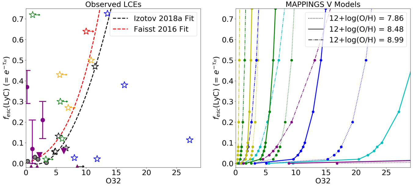
Figure 10. A comparison of the empirical relations between O32 and f_{esc}(\text{LyC}) suggested by Izotov et al. (2018b) and Faisst (2016) (left) with the theoretical predictions calculated using MAPPINGS V (right). On the left, LCEs at z \approx 0.05 from Izotov et al. (2016) and Izotov et al. (2018b) are shown as black, open stars as in Figures 6 and LCEs from Izotov et al. (2018a) are shown with blue, open stars. Lower redshift LCEs are indicated with grey circles. The open red star indicates the high redshift LCE, Ion2 (de Barros et al. 2016) and orange and green open stars show “gold” and “silver” subsamples of LCEs from the LACES survey (Fletcher et al. 2018). Observations for our sample are shown with purple symbols. Circles with error bars show galaxies with nonzero f_{esc}(\text{LyC}) from CLAUDS u -band photometry, downward triangles show upper limits on f_{esc}(\text{LyC}) based on CLAUDS u -band uncertainty, and small, upwards triangles show galaxies with f_{esc}(\text{LyC}) = 0.0 even when uncertainty in u is considered. The empirical fits presented in Izotov et al. (2018b) and Faisst (2016) and shown by black and red dashed lines, respectively. The fit of Faisst (2016) includes Ion2 and all black LCEs except for the one at the highest O32 and the fit of Izotov et al. (2018b) excludes Ion2 and includes all black, open stars. Blue open stars were reported more recently than either fit, and thus were not included. On the right, coloured lines show the outputs of the MAPPINGS V code at fixed Z with colours indicating different q_{ion} , identical to Figure 8. Different line styles for MAPPINGS V results correspond to different 12 + \log_{10}(O/H) as indicated in the legend.
