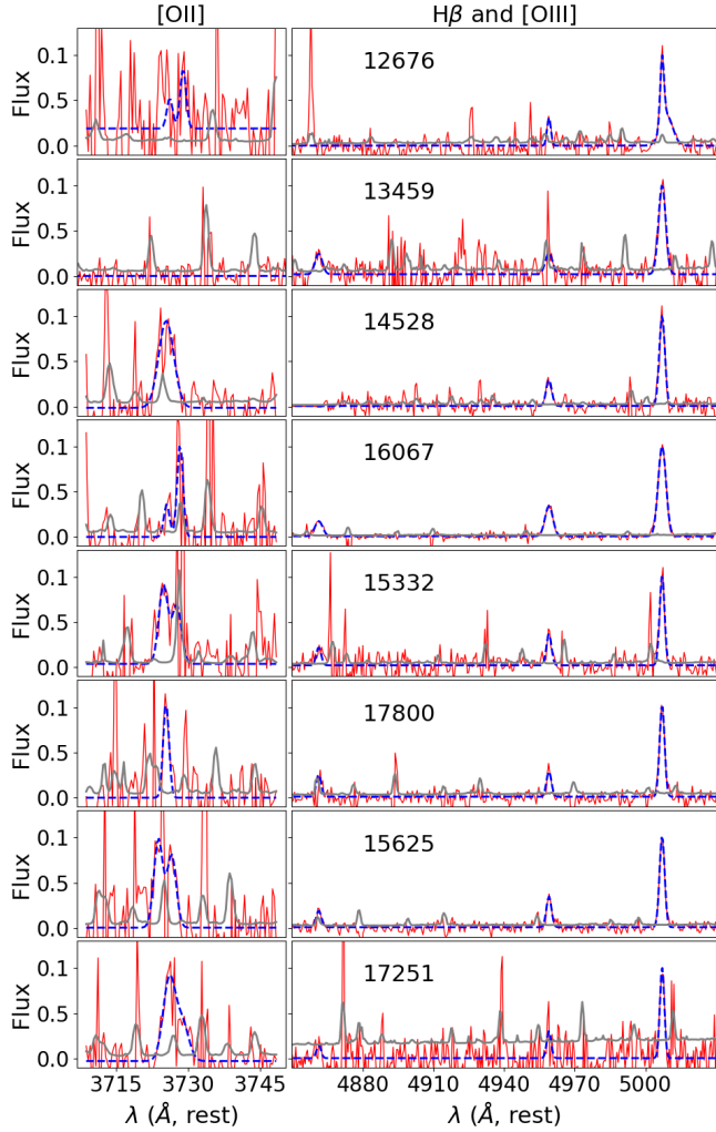
Figure 3. MOSFIRE spectra for \mu S selected z \sim 3 galaxies in our sample. Red lines show the observed spectra whereas blue dashed lines show our emission line fits as described in Section 4.1. The grey lines show the error spectrum. For all galaxies shown here, the [OII] doublet is observed in the H-band while H\beta and the [OIII] doublet both fall in the K-band. H-band data are plotted normalised by the maximum flux in our [OII] line fits, and, similarly, K-band data are plotted normalised by the peak flux of our [OIII] and H\beta line fit. Dust corrected line fluxes are given in Table 2.
