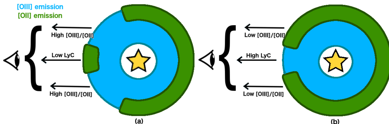
Figure 11. A conceptual picture of the differing geometric effects on observed LyC and scattered line emission from H II regions with holes. Blue indicates the hot, diffuse, [OIII] ( \lambda 5007 \text{ \AA} ) emitting inner regions while green indicates cool, dense, [OII] ( \lambda \lambda 3727 \text{ \AA} ) emitting outer regions. Giammanco et al. (2005) and Pellegrini et al. (2012), as well as our own MAPPINGS V analysis, have shown that a high gas density results in a lowered observed O32 value. (a): A low overall covering fraction of dense gas with the chance alignment of a small, dense clump that obscures the ionizing photon source(s). This would result in low f_{esc}(\text{LyC}) and high O32 (e.g. Izotov et al. 2018a). b: A high overall covering fraction of dense gas with the chance alignment of a small hole in front of the source(s) of ionizing photons. This would result in a high f_{esc}(\text{LyC}) and a low O32 (e.g. our sample). See Reddy et al. (2016), Fletcher et al. (2018), and Steidel et al. (2018) for further discussion on the implication of clumpy geometry on f_{esc}(\text{LyC}) .
