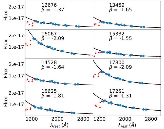
Figure 4. Exponential fits to the restframe photometric data (ZFOURGE) for galaxies in our sample. The y-axes indicate flux in units of \text{ergs s}^{-1} \text{ cm}^{-2} \text{ Å}^{-1} . Model fits, indicated by the solid black lines, are of the form F(\lambda) \propto \lambda^\beta . Data from photometric bands used in our fits are shown in blue while data below rest-frame \sim 1200 \text{ Å} (shown in red), below which the galaxy SED deviates significantly from an exponential behavior as a result of Ly \alpha absorption. The final fitted values of \beta are indicated in each panel.
