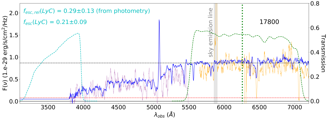
Figure 5. An illustration of our method of estimating f_{esc}(LyC) from CLAUDS u band photometry for galaxy 17800. CLAUDS u and r transmission curves (with atmospheric transmission, optics throughput, and CCD quantum efficiency accounted for) are shown by cyan and green dashed lines, respectively, with transmission given by the right y-axis. Corresponding observed F_\nu in the u and r bands are shown by the horizontal red and black dashed lines, respectively. The composite spectrum, constructed from stacked LBG spectra of Shapley et al. (2003), is normalised based on the r band flux and is shown by the solid blue line. Our LRIS spectrum, which has been smoothed using a tophat filter with a width of 20 Å, for the blue and red arms are shown in purple and orange, respectively (note that the quoted f_{esc}(LyC) is not measured from the LRIS spectrum). The estimated value for photometric f_{esc}(LyC) is annotated in the upper left. Finally, we indicate \lambda_{rest} = 1500 Å with a green, vertical dotted line.
