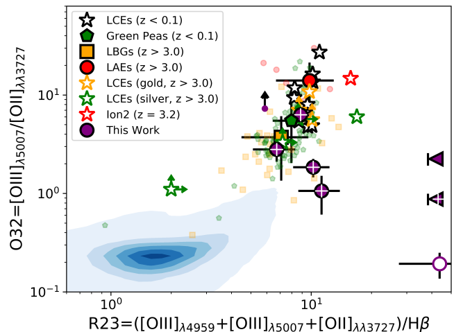
Figure 6. R23 vs O32 for our sample in comparison with various samples of high and low redshift star-forming galaxies. For most comparison samples, small symbols indicate individual galaxies and corresponding large, opaque symbols show averages for each sample. The exception is LyC emitting galaxies shown as white stars. Those with black edges are low- z galaxies from Izotov et al. (2016), Izotov et al. (2018a), and Izotov et al. (2018b), the red edged white star is the high- z galaxy Ion2 (de Barros et al. 2016; Vanzella et al. 2016), and orange and green edged white stars are z > 3.0 galaxies from the “gold subsample” and “silver subsample”, respectively, of the LACES survey (Fletcher et al. 2018). Star-forming SDSS galaxies from (Zahid et al. 2013) are shown by the blue density contours. Galaxies in our MOSFIRE sample with detections of [OII] ( \lambda\lambda 3727 Å), [OIII] ( \lambda 4959 Å), [OIII] ( \lambda 5007 Å), and H \beta are shown with large purple circles. Circles with white crosses indicate confirmed Ly \alpha emitters. Filled triangles represent those galaxies without H \beta observations indicating only O32 values and not R23 upper-limits. The small purple circle indicates the upper limit on O32 for galaxy 13459 (not detected in [OII] \lambda\lambda 3727 Å). The open purple circle represents galaxy 17251, which shows evidence of being an ongoing merger (see Figure 2 and Section 5.1.1). Shocks associated with mergers may explain both the high R23 and low O32 values observed in this galaxy.
