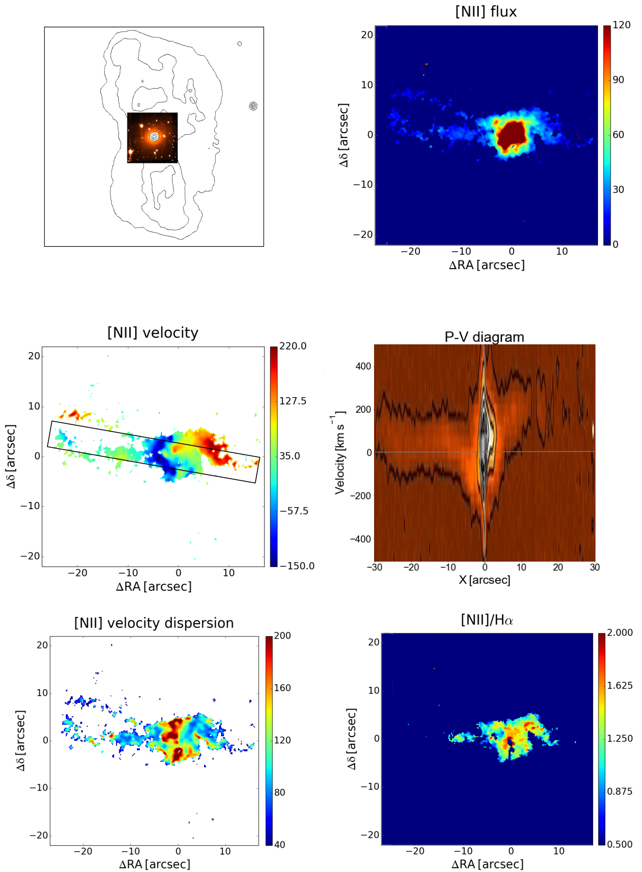
Fig. 11. 3C 386, FR II, 1'' = 0.35 kpc.
