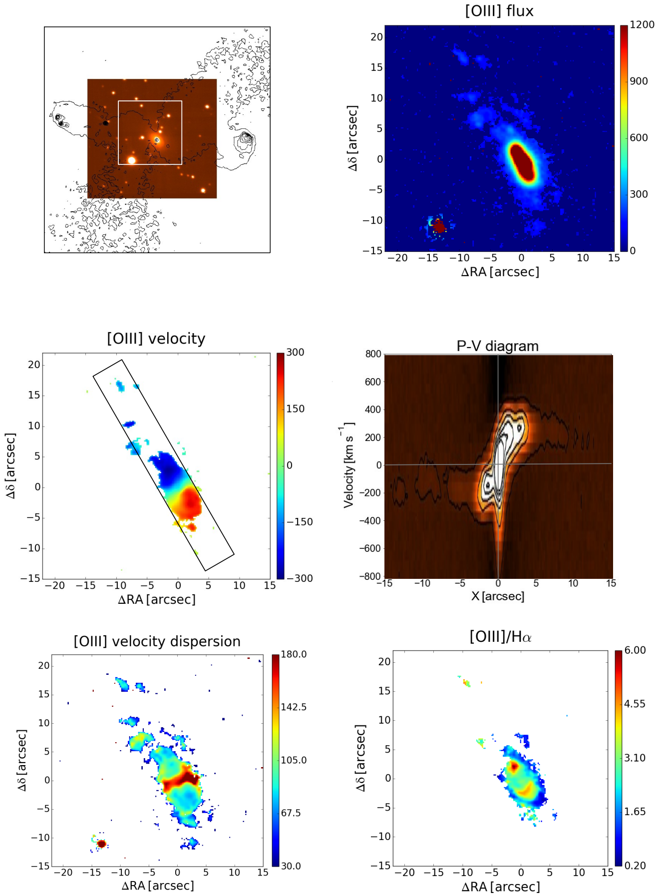
Fig. 12. 3C 403, FR II/HEG, 1'' = 1.15 kpc.
