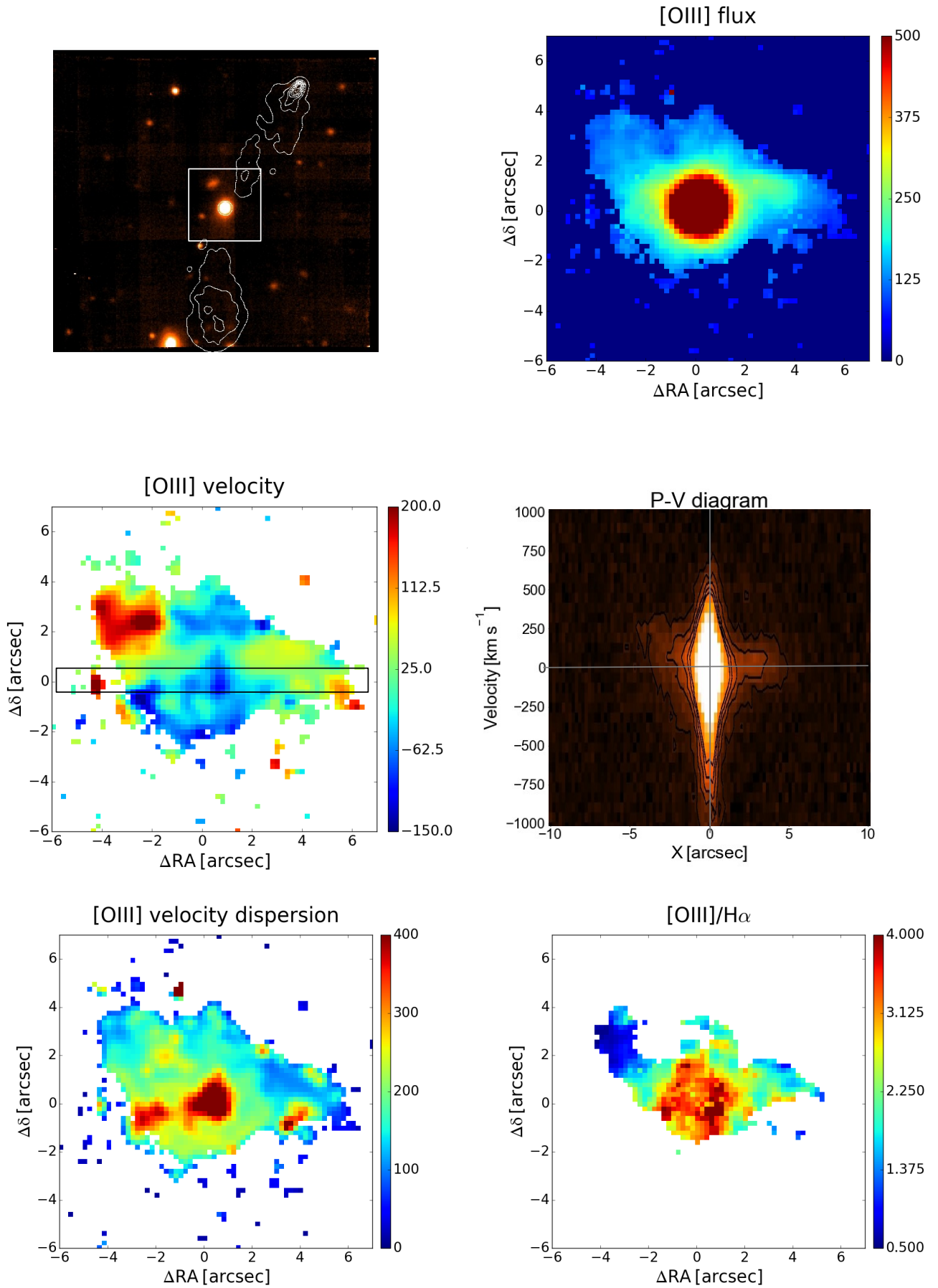
Fig. 3. 3C 018, FR II/BLO, 1'' = 3.17 kpc. Same as Fig. 2.
