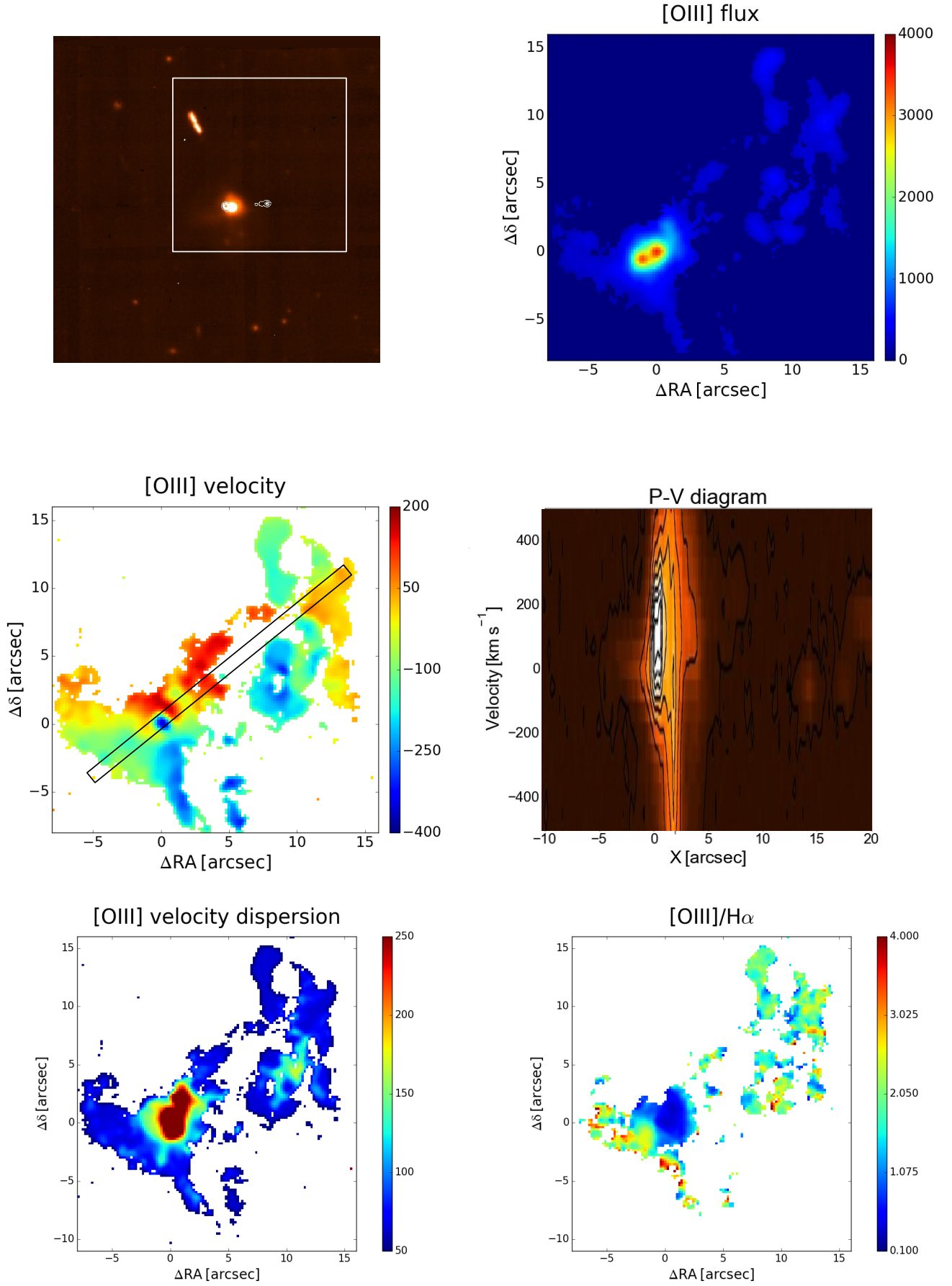
Fig. 19. 3C 459, FR II/BLO, 1'' = 3.58 kpc.
