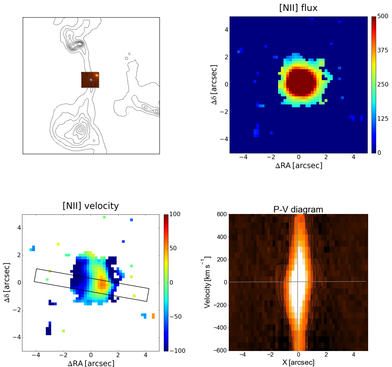
Fig. 6. 3C 040, FR I/LEG, 1'' = 0.37 kpc. Top left: radio contours overlaid onto the optical continuum image. Top right: [N II] emission line image. Bottom: velocity field from the [N II] line and position velocity diagram extracted from the synthetic slit shown overlaid onto the velocity field.
