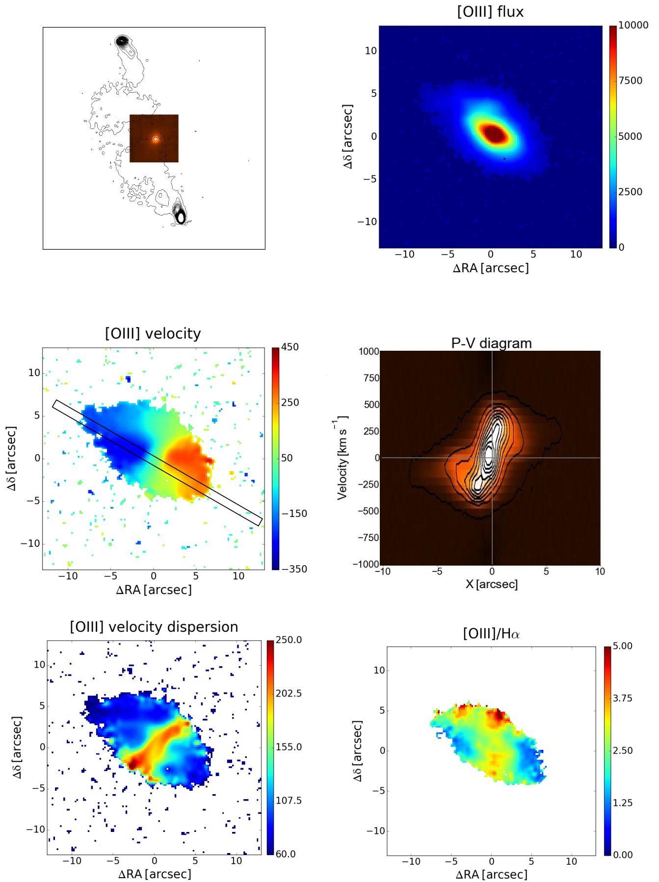
Fig. 5. 3C 033, FR II/HEG, 1'' = 1.17 kpc. Same as Fig. 2.
