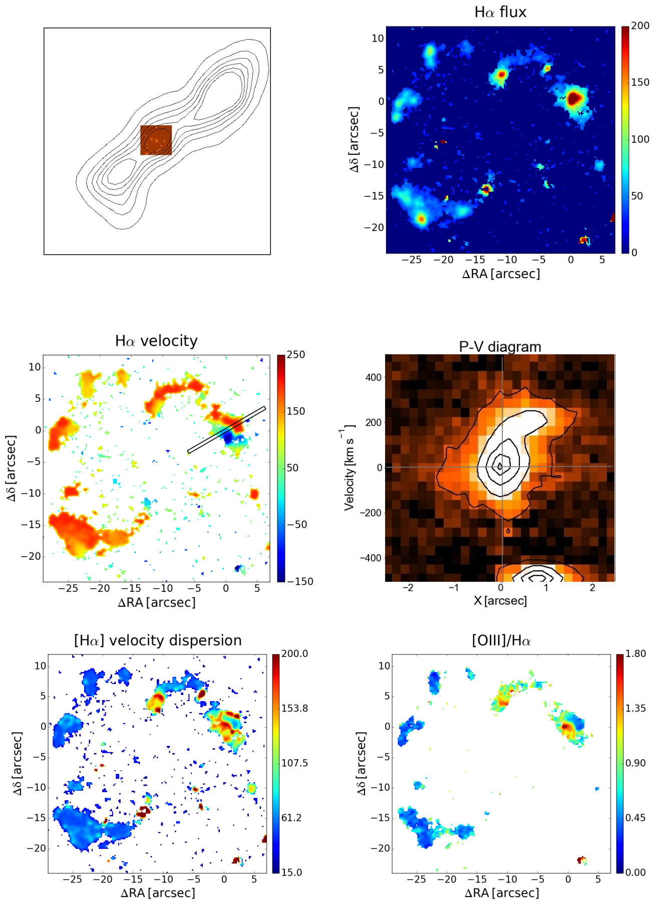
Fig. 13. 3C 403.1, FR II/LEG, 1'' = 1.07 kpc.
