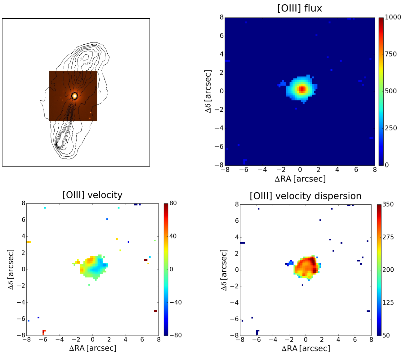
Fig. 4. 3C 029, FR I/LEG, 1'' = 0.89 kpc. Top left: radio contours overlaid onto the optical continuum image. Top right: [O III] emission line image. Bottom: velocity field from the [O III] line and velocity dispersion. Fluxes are in 10^{-18} \text{erg s}^{-1} \text{cm}^{-2} \text{arcsec}^{-2} , velocities are in \text{km s}^{-1} units.
