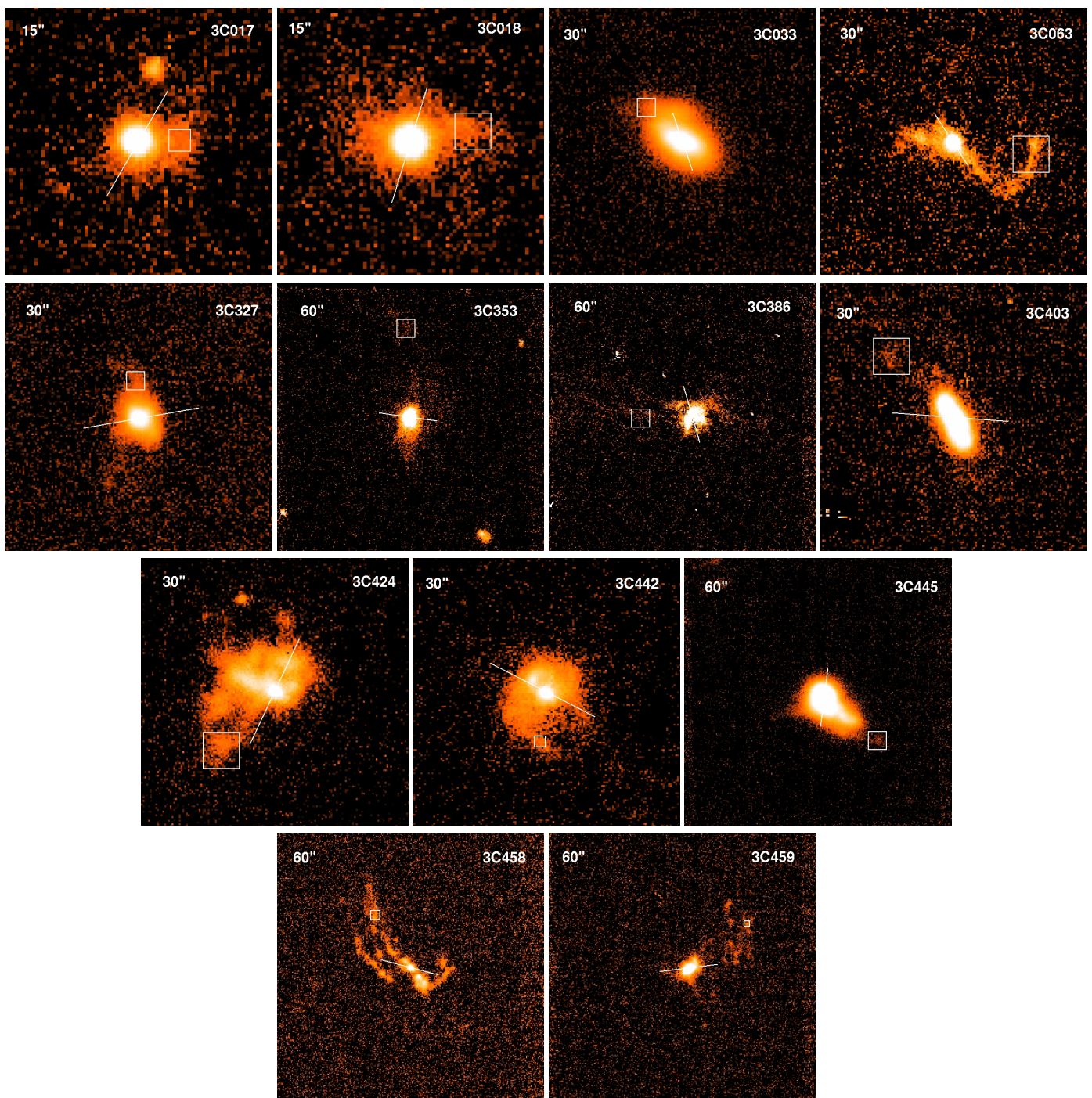
Fig. 20. Emission line images (in logarithmic scale) of the 13 radio galaxies observed in MURALES with extended emission lines. The fields of view are indicated in the upper left corner of each image. The white segments are parallel to the radio axes, the with boxes mark the synthetic aperture from which we extracted the off-nuclear spectra.
