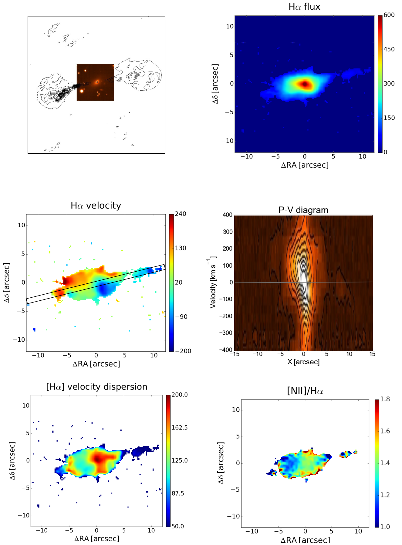
Fig. 9. 3C 348, FR I/ELEG, 1'' = 2.71 kpc.
