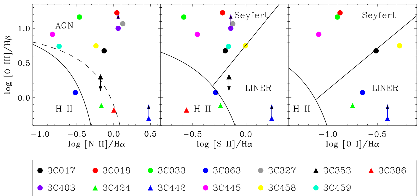
Fig. 21. Location of the 13 FR II radio galaxies with extended line emission in the spectroscopic diagnostic diagrams. Circles (triangles) correspond to source classified as HEGs (LEGs) based on their nuclear emission line ratios (Buttiglione et al. 2010). The solid lines separate star-forming galaxies, LINERs, and Seyferts (Kewley et al. 2006).
