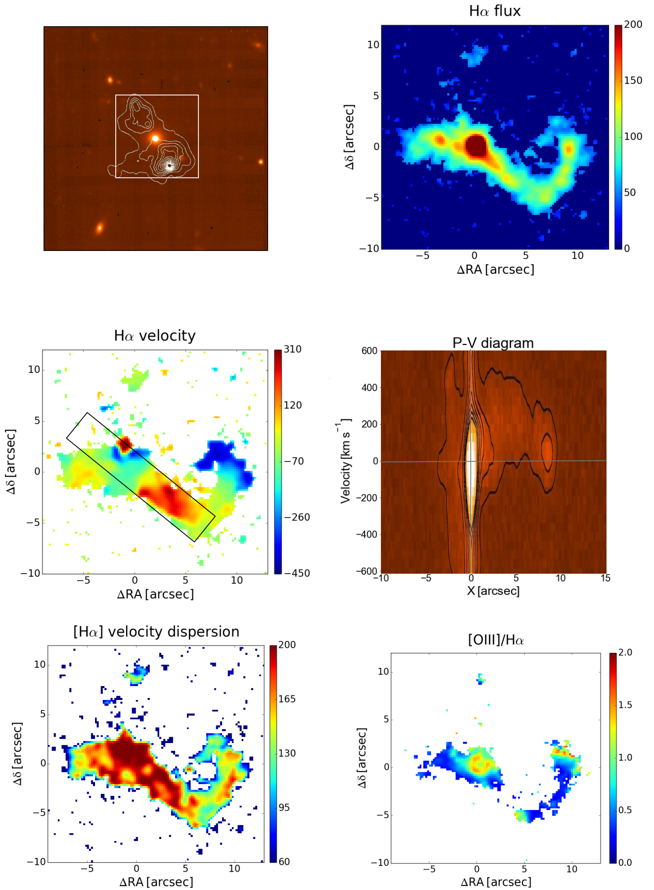
Fig. 7. 3C 063, FR II/HEG, 1'' = 2.99 kpc. Same as Fig. 2
