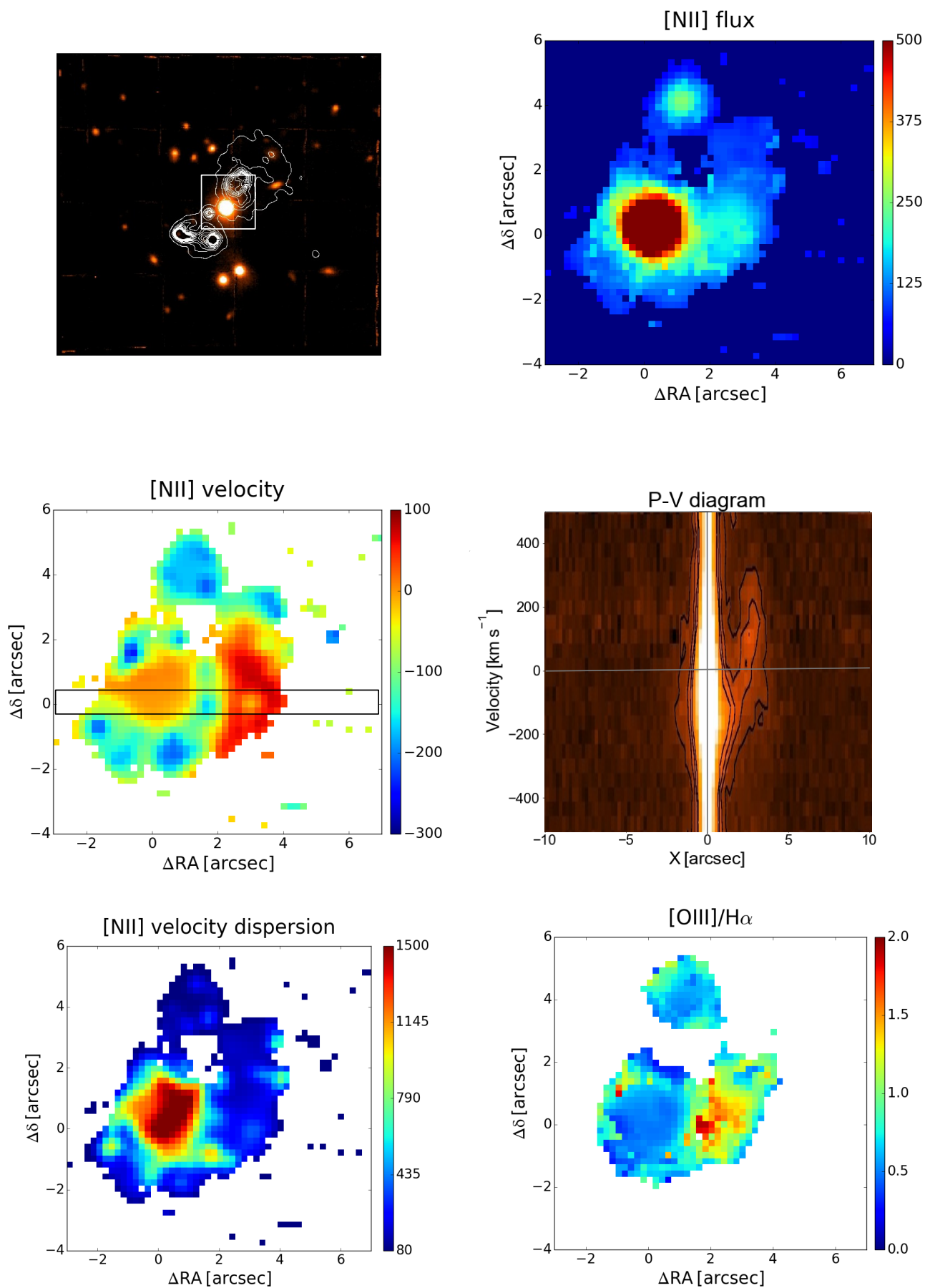
Fig. 2. 3C 017, FR II/BLO, 1'' = 3.58 kpc. Top left: radio contours (in white) overlaid onto the optical continuum image over the MUSE field of view. Top right: [N II] emission line image extracted from the white square marked in the left panel. Middle left: gas velocity obtained from the [N II] line. Middle right: position-velocity diagram extracted from the synthetic slit shown overlaid onto the velocity field. Bottom: velocity dispersion and map of the [O III]/H \alpha line ratio. Fluxes are in 10^{-18} erg s -1 cm -2 arcsec -2 , velocities are in km s -1 units. Article number, page 5 of 27
