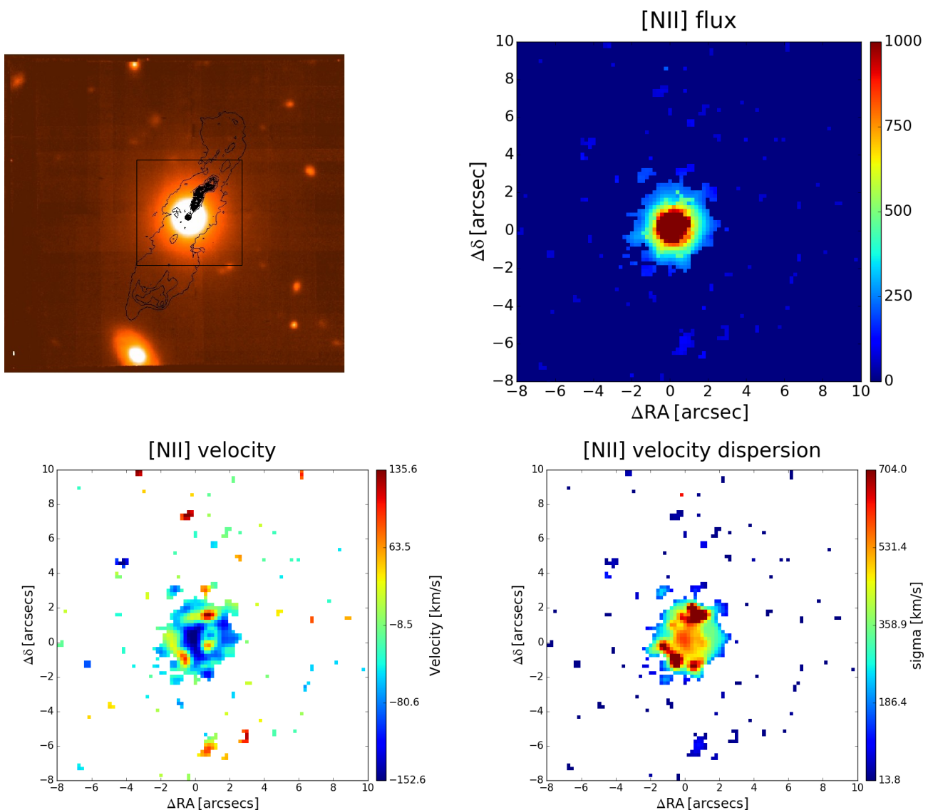
Fig. 1. 3C 015, FR I/LEG, 1'' = 1.40 kpc. Top left: radio contours (black) overlaid onto the optical continuum image in the 5800 and 6250 Å rest frame range. The size of the image is the whole MUSE field of view, 1' \times 1' . Top right: [N II] emission line image extracted from the black square marked in the left panel. Fluxes are in 10^{-18} \text{erg s}^{-1} \text{cm}^{-2} \text{arcsec}^{-2} . Bottom: velocity field from the [N II] line and velocity dispersion. Velocities are in \text{km s}^{-1} units.
