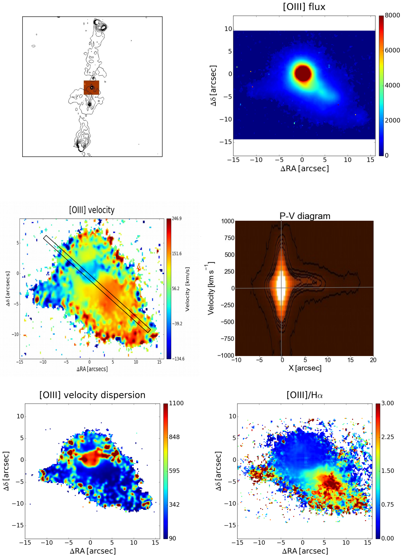
Fig. 16. 3C 445, FR II/BLO, 1'' = 1.09 kpc.
