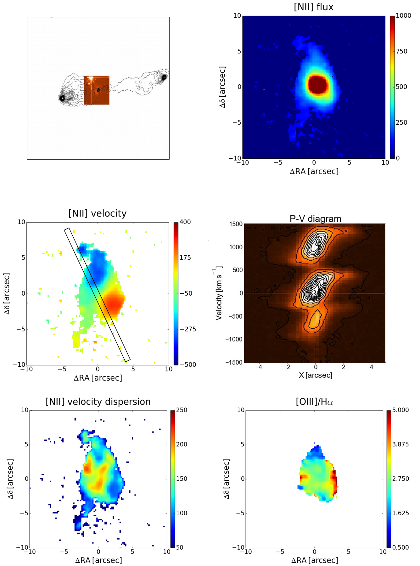
Fig. 8. 3C 327, FR II/HEG, 1'' = 1.94 kpc. Same as Fig. 2
