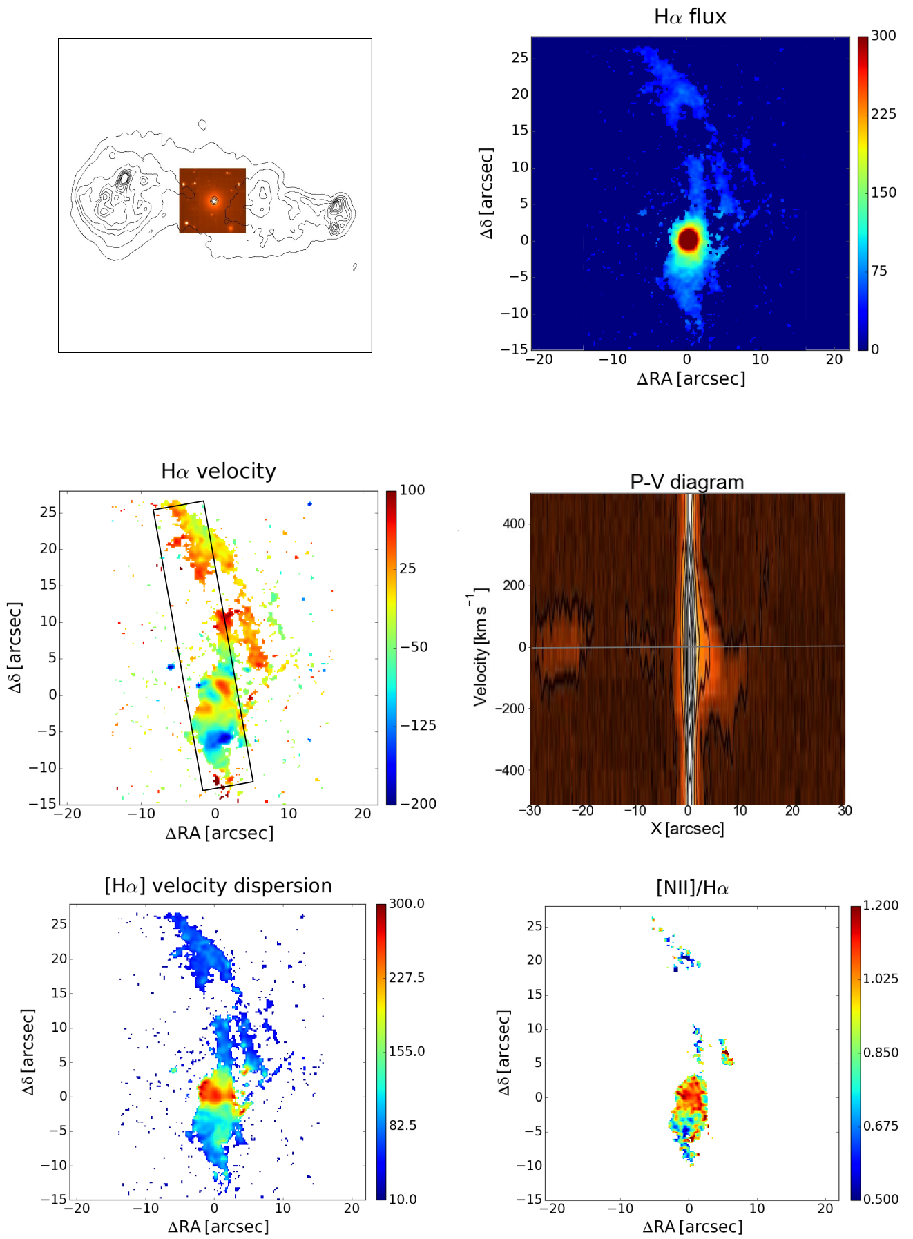
Fig. 10. 3C 353, FR II/LEG, 1'' = 0.60 kpc.
