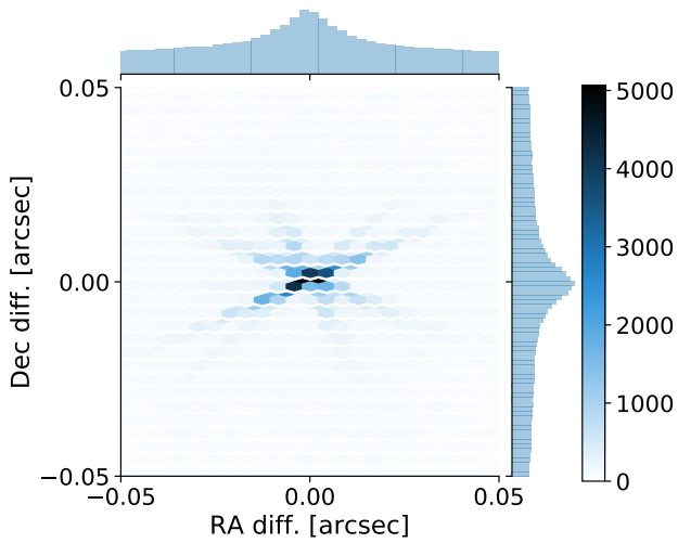
Figure 8. Offsets of masterlist positions to GAIA reference for objects with GAIA g magnitude larger than 18.
