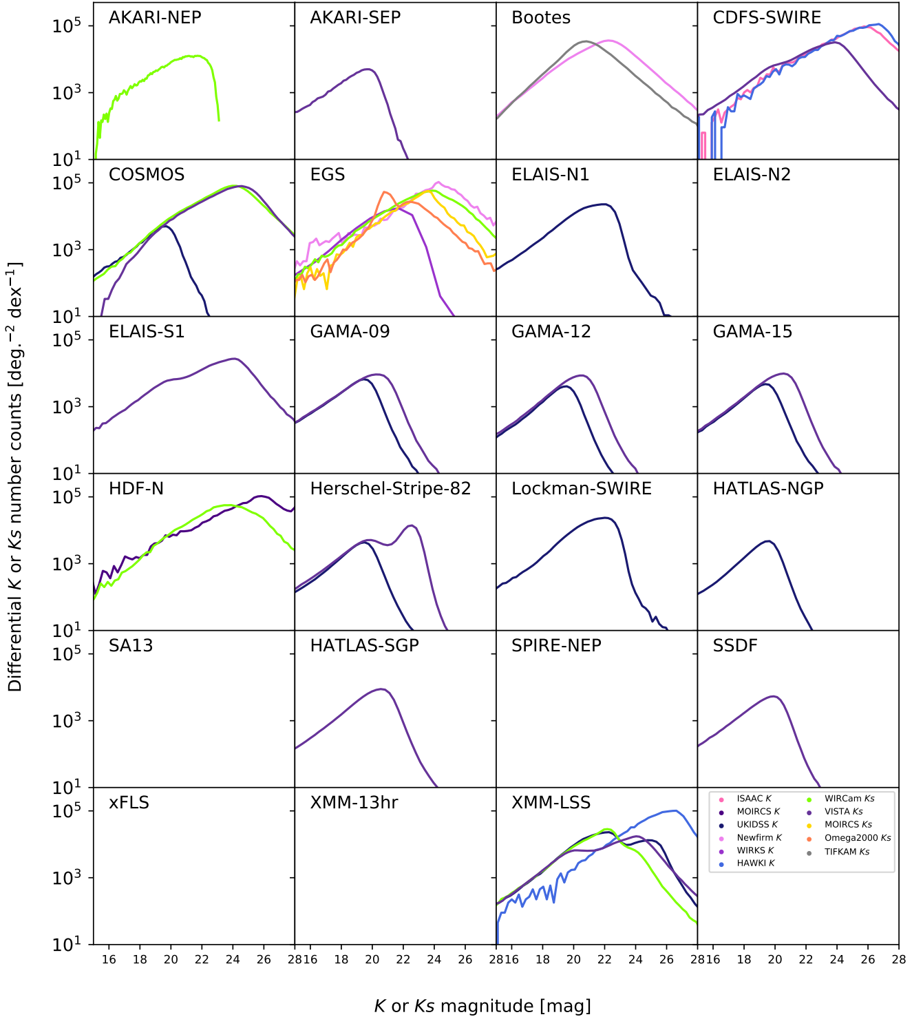
Figure 26. The differential K , or K_s (total magnitude) number counts for the most frequently encountered wide area K , or K_s broad band fluxes available in the catalogue. Occasionally, where a survey has regions in the field to different depths there are multiple peaks. These are computed using the area over which a given band is available on a given field. There are five fields without any K or K_s data. These are ELAIS-N2, SA13, SPIRE-NEP, xFLS, and XMM-13hr.
