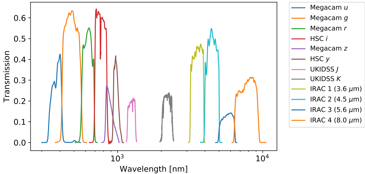
Figure 2. Filter transmission curves for a sample of filters present on the example field ELAIS-N1. Some of the optical bands have multiple measurements from different instruments with similar filters. We only show one for each band to aid clarity. These responses include quantum efficiency of the camera and atmospheric extinction as measured by the respective telescopes. Wavelength coverage varies significantly across the HELP fields. Figures for each individual field are provided in the notebooks.
