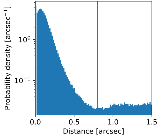
Figure 7. Number density of objects from the masterlist within a given distance from a GAIA object with g magnitude above 18. For bright stars there are large numbers of artefacts. This figure demonstrates that 0.8 arcsec is effective as a standard cross match distance. Taking all objects within 0.8 arcsec will include the majority of true matches (peak at left) and a minority of background erroneous matches (linear slope). This value is chosen for every catalogue based on the minimum in the above figure. For the majority of catalogues 0.8 arcsec (vertical line on plot) is appropriate.
