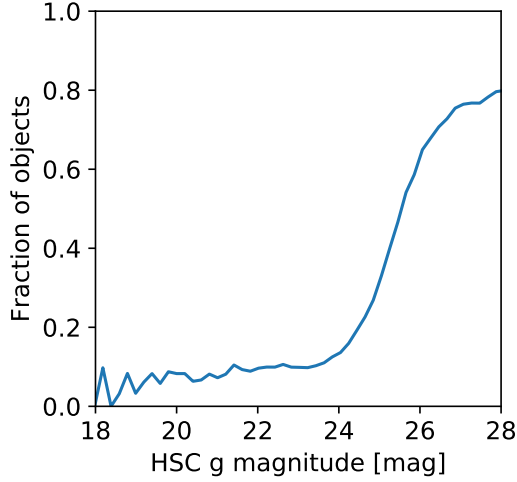
Figure 10. Fraction of HSC objects which are flagged as merged (associated to multiple other objects) but rejected as a counterpart based on the closest match criteria as a function of HSC g magnitude. These objects are unmatched and only have HSC fluxes. We expect the faintest HSC objects to be unmatched since HSC is often the deepest survey available over most of the area it exists.
