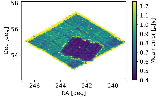
Figure 18. Map of the example ELAIS-N1 field showing the mean error on the IRAC i1 flux over order 10 HEALPix cells. The mean error, which can be used as a proxy for depth, makes it possible to take account of selection effects over large areas with highly inhomogeneous observation depths. The smaller and deeper SERVS area is clearly visible against the wider and shallower SWIRE area.
