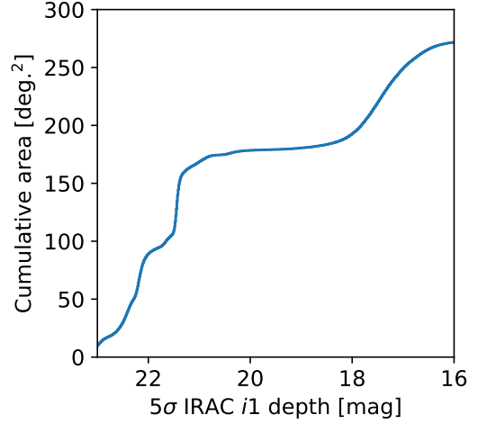
Figure 23. The area of HELP coverage with 5\sigma point-source IRAC i1 band depth above a given value. IRAC i1 is available over 273 deg. 2 . Building the \chi_{ID}+ priors on these regions requires flux prediction techniques that will be discussed in the upcoming paper by Oliver et al. Figures 21 to 23 play a key role in the selection of objects for HELP processing and are a necessary component of modelling selection.
