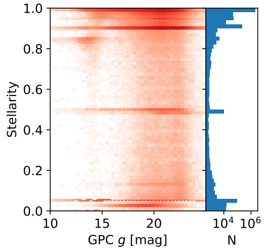
Figure 11. The distribution of stellerity index, which should reflect point-sourceness (definitely point like = 1, definitely extended = 0) with GPC1 g flux for GAIA objects. Approximately one percent are incorrectly labeled as extended.
