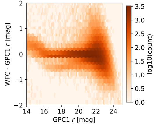
Figure C1. Comparison between PanSTARRS GPC1 r band magnitudes and INT-WFC r band magnitudes on the example field ELAIS-N1. We see errors increasing for fainter objects.
