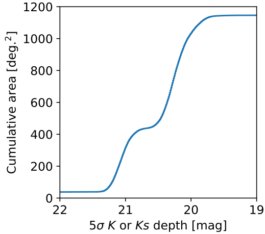
Figure 22. The area of HELP coverage with any 5\sigma point-source K or Ks depth above a given value. The depth map product has the mean errors for all K and Ks bands allowing us to query the lowest value on every HEALpix cell.
