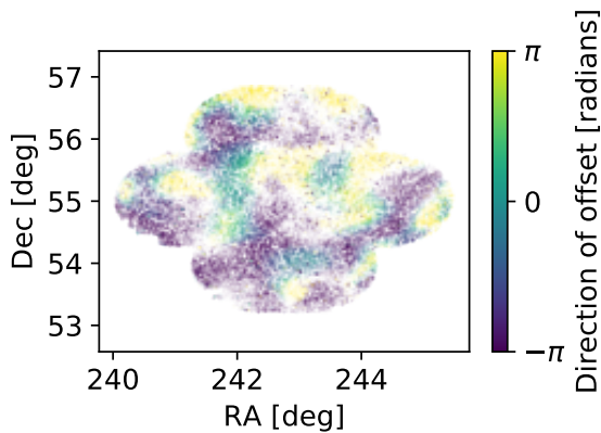
Figure 9. Direction of residual astrometric offsets between HSC positions and the GAIA reference frame, after correction for mean offset, for the example field ELAIS-N1. Colour indicates the direction and intensity indicates the size of residual offset.
