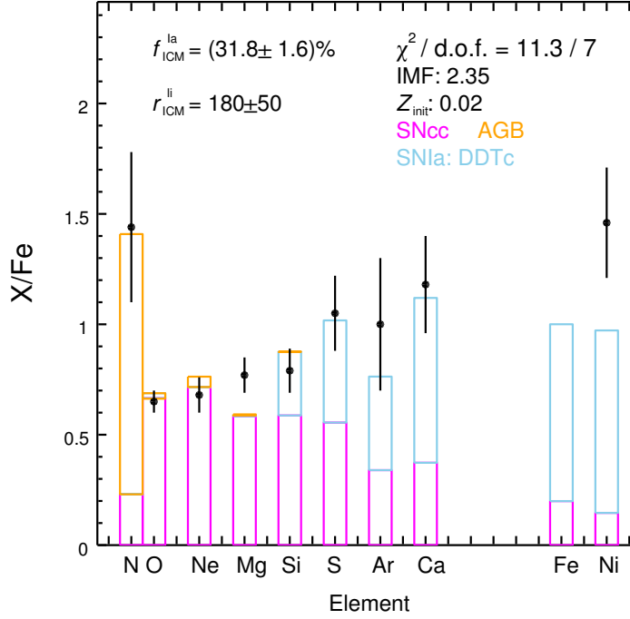
Figure 1. The chemical enrichment of the hot plasma in NGC 5044 observed with XMM-Newton . The abundance ratios are measured with the cie model in SPEX v3.04. Under a standard initial mass function (IMF) with a slope of -2.35 [10] and an initial metallicity ( Z_{\text{init}} = 0.02 , i.e. solar composition) of progenitors, a suitable mixture of different enrichment channels are required to fit the observed abundance ratios. Nitrogen is mainly enriched via the stellar winds of AGB stars. Core-collapse supernovae (SNcc) are the main elemental factory of the so-called \alpha -elements (e.g., O, Ne, and Mg). Type Ia supernovae (SNIa) dominate the enrichment of the Fe-peak elements (e.g., Fe and Ni). This figure, originally shown in [11], is reproduced with permission.
