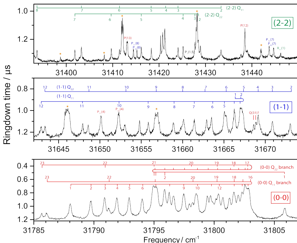
Figure 2: Q-branch regions of the 0-0 band (bottom panel, assignments in red), 1-1 band (middle, blue) and 2-2 band (top, green). Lines from the 0-0 band are labelled in red in the middle and upper panels. Lines from the 1-1 are labelled in blue in the upper panel. The features indicated with stars are of unidentified origin.
