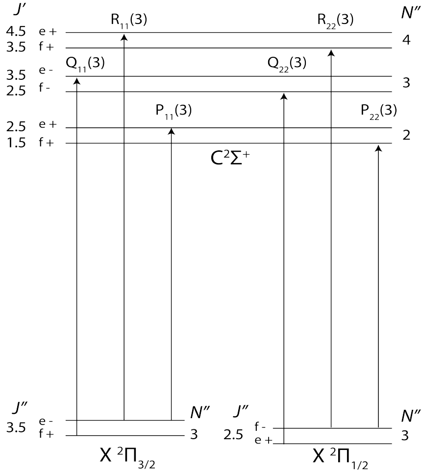
Figure 1: Schematic illustrating the six rovibronic bands of the C^2\Sigma^+ - X^2\Pi band of CH for the chosen energy levels, e/f refer to electronic symmetry, +/- refer to total parity.
