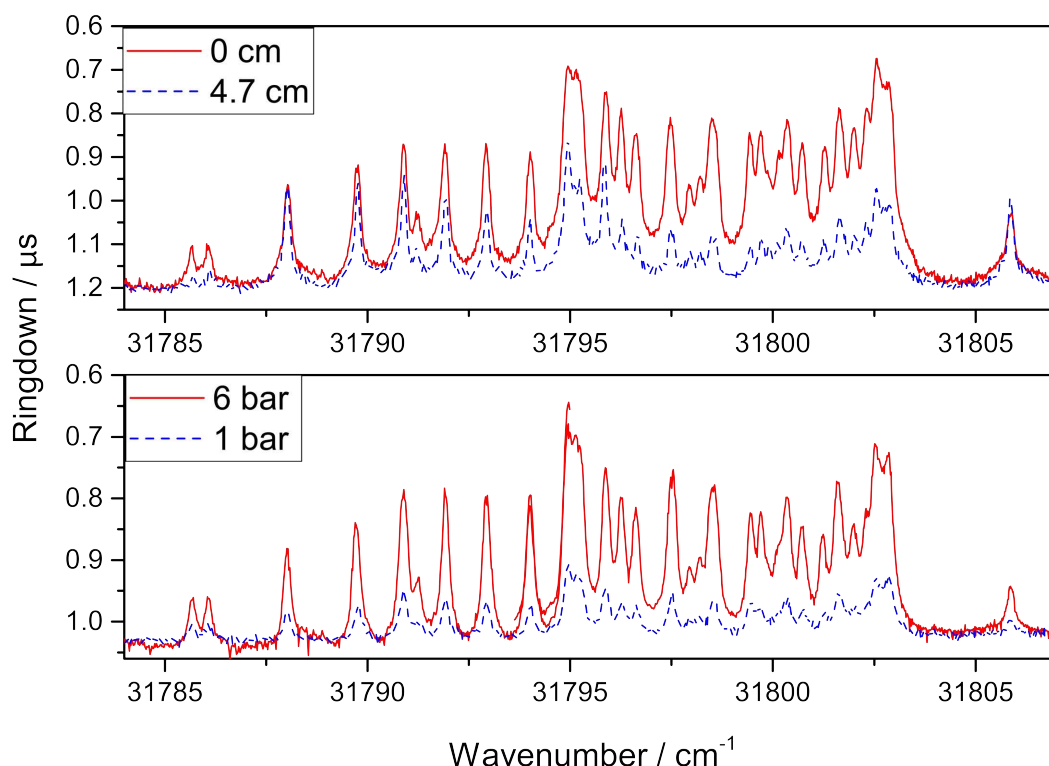
Figure 3: The Q-branch region of the 0-0 band of the C-X transition at different experimental conditions. Top panel compares a CRDS measurement close to the nozzle orifice (red) and 4.7cm down (blue). The bottom panel compares a high backing pressure of \text{C}_2\text{H}_2/\text{Ar} of 6 bar (red) with a lower pressure of 1 bar (blue).
