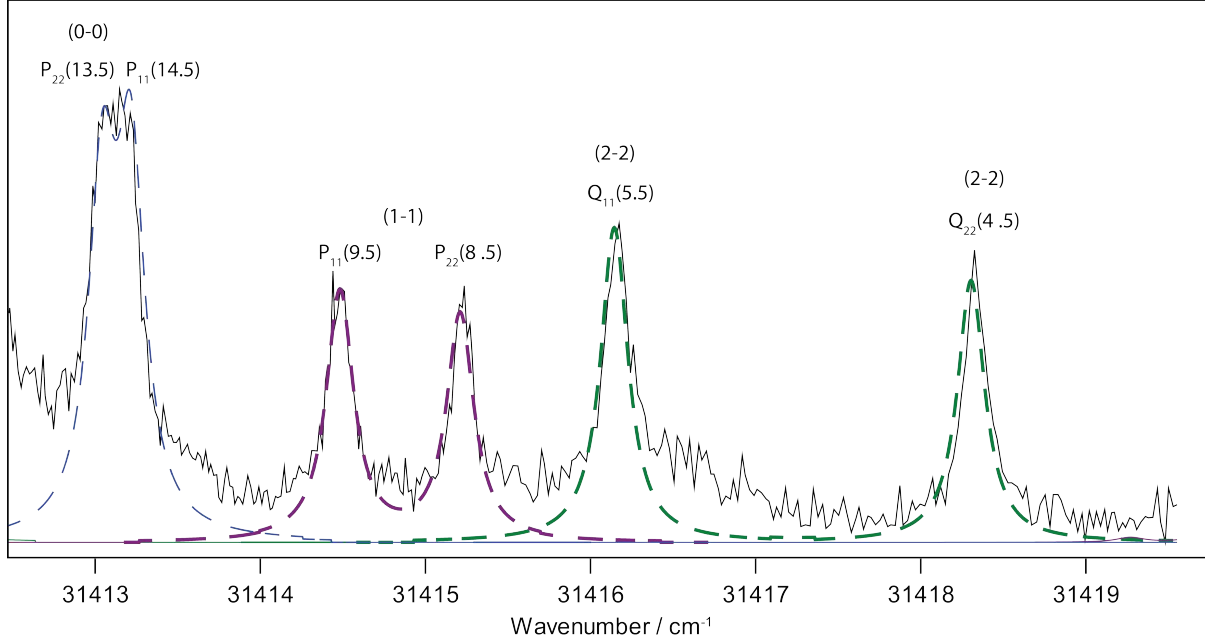
Figure 5: A zoom of the Q-branch region of the 2-2 band of the \text{C}^2\Sigma^+ - \text{X}^2\Pi transition of CH showing the line profiles of transitions from all three vibronic bands with near equal intensity and line width in a single recording. Simulated line widths (dashed lines) are Lorentzians with 0.2 \text{ cm}^{-1} FWHM as simulated in PGOPHER.
