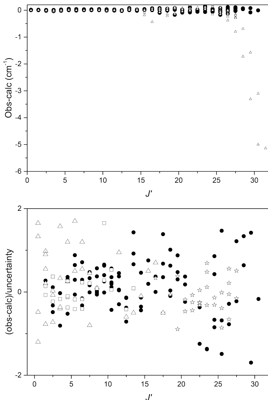
Figure 4: Residual plots for the 0-0 vibronic band. Upper: comparison of residuals of all data presented here when using molecular constants determined here (solid circles) and the constants presented in Masseron et al. [4] (open triangles). Lower: weighted residuals from the fit presented for all lines in this work (solid circles), from Heimer [21] (open stars), Ubachs et al. [23] (open triangles) and from Bembenek et al. [24] (open squares).
