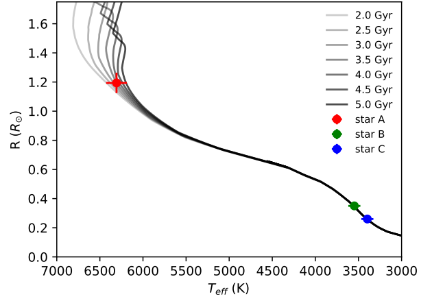
Figure 3. The H-R diagram for EPIC 249624646 (star A) and its two stellar companions (star B and star C) together with BaSTI isochrones ranging from 2.0 to 5.0 Gyr and with [Fe/H] = -0.1.
