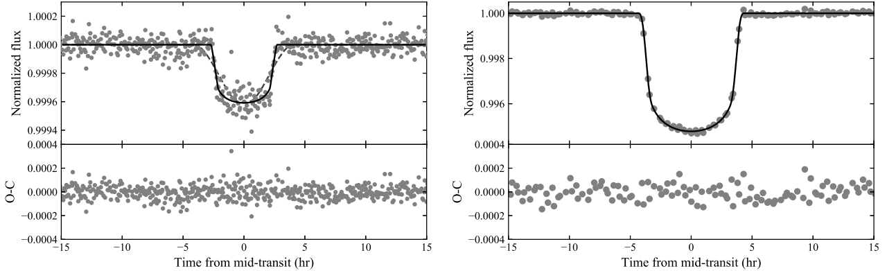
Figure 6. Phasefolded transit light curves of EPIC 249624646b (left) and EPIC 249624646c (right) observed with K2, together with the best-fitting model from the joint analysis of the photometry and spectroscopy (solid line). The bottom plot shows the residuals. The values of the corresponding best-fit parameters are displayed in Table 4. The dashed line on the left plot indicates the modelled light curve in the case of the shallow transit signal being a false positive caused by star B. In order to reproduce the observed depth in the combined light of star A and B, this would require star B to be an eclipsing binary diluting star A with a transit depth of 15% – 30%. This would lead to a very V-shaped transit, which is not what we observe. For the deep transit (right plot), even a total eclipse of star B is not sufficient to reproduce the signal.
