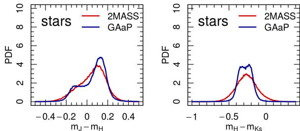
Fig. 5. Comparison between the colours of KV450 stars and the same sources measured by 2MASS. The reduction in scatter of the distribution indicates that the KV450 NIR data have significantly reduced uncertainties.
