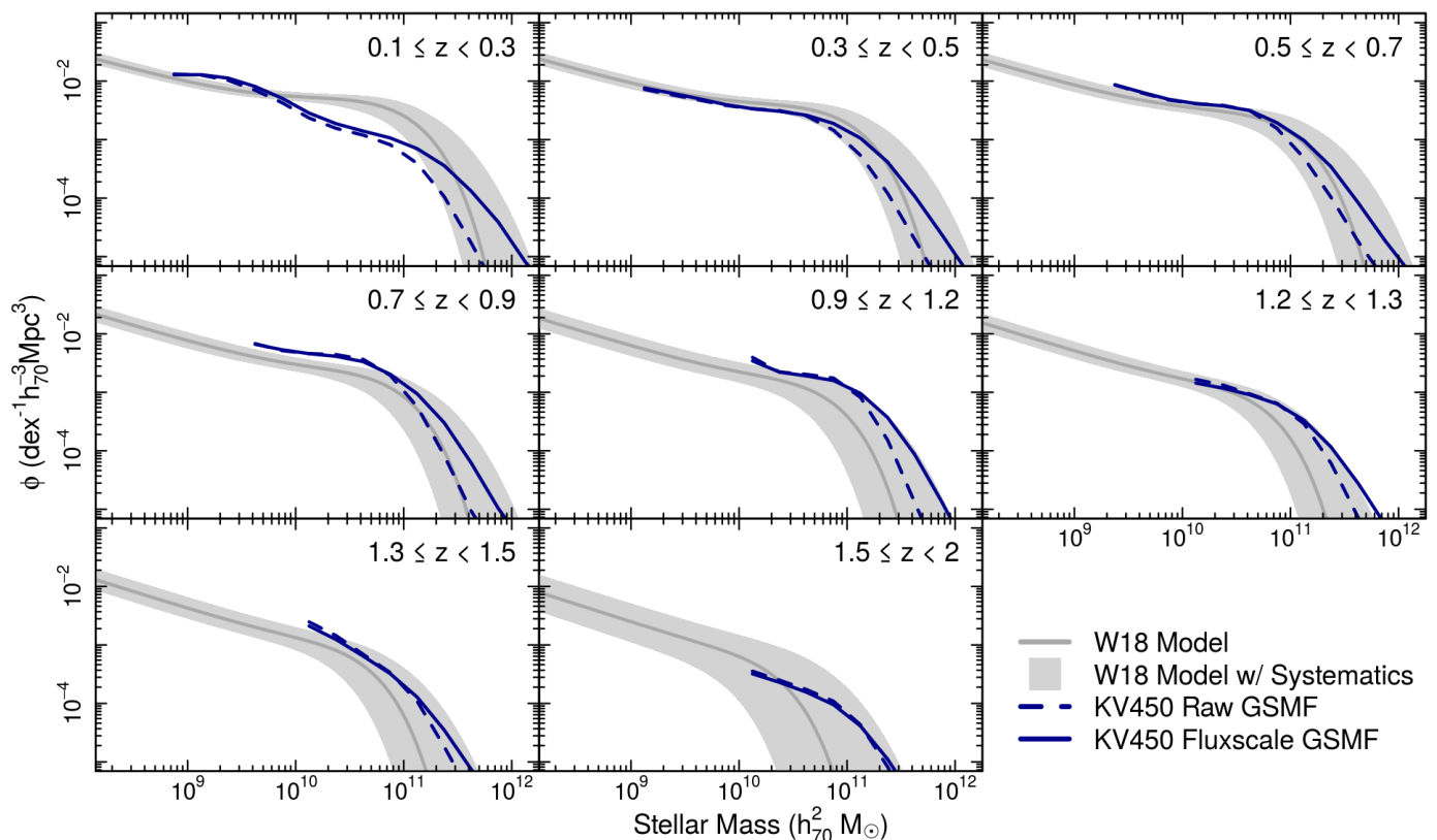
Fig. 11. Galaxy stellar mass functions for the KV450 dataset, shown with (blue, solid) and without (blue, dashed) the fluxscale factor incorporated, compared to the mass function model given in Wright et al. (2018) (dark grey). KV450 lines are shown only over the range where we believe the mass function to be volume complete. To ensure a fair comparison, we also show the model mass function when allowing for uncertainty in photometric redshift ( |\Delta z| \leq 0.02 ) and Eddington bias ( |\Delta M_*| \leq 0.2 ) in grey. The KV450 mass function shows a significant deviation from the expectation in the lowest redshift bin, which we attribute to a bias against selecting the largest-angular-size galaxies in our analysis (see Section 5). In all other bins the agreement with the model is exceptional given the simplicity of the analysis performed, and inspires considerable confidence in the fidelity of our mass estimates.
