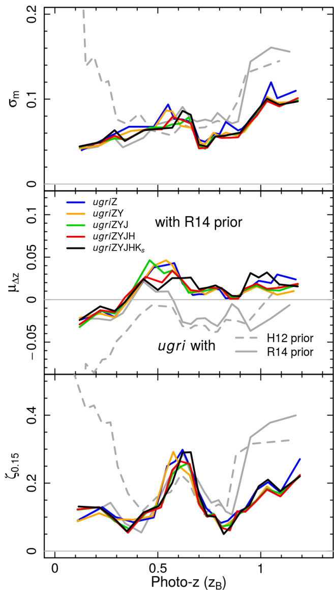
Fig. 8. Variation in the photo- z vs spec- z distribution parameters as a function of photo- z , for the 4-band KiDS-450 dataset with two different priors ( grey lines ), and as a function of NIR photometric information for the KV450 dataset ( coloured lines ). The three panels show the spread in the distribution, determined by a running normalised-median-absolute-deviation from the median ( \sigma_m ; top ), the median bias in the photo- z distribution ( \mu_{\Delta z} ; middle ), and the fraction of sources with |\Delta z|/(1+z_{\text{spec}}) > 0.15 ( \zeta_{0.15} ; bottom ). The addition of the Raichoor et al. (2014) prior to the 4-band data causes significantly better behaviour at low z_B , while the addition of NIR data improves the population consistency and scatter in particular at high z_B .
