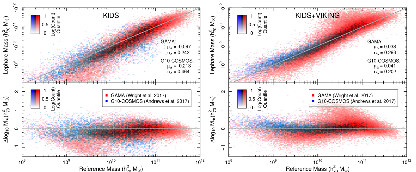
Fig. 9. Comparison between stellar mass estimates from both KiDS-450 ( left ) and KV450 ( right ) with those from both the GAMA and G10-COSMOS samples, for those sources which overlap. KiDS-450 masses here are derived using the KiDS-450 photo- z and only ugri photometry. Both KiDS datasets are shown with masses which have been corrected using our fluxscale parameter. Sources in the comparison samples are selected for comparison only if their masses have been estimated using spectroscopic redshifts. The figure demonstrates the significant improvement in mass estimates that is made when using 9-band photometric information. In particular, significant reduction on the scatter of the deep G10-COSMOS dataset is particularly important. Scatter in the highest-mass GAMA sources is due to the updated photo- z prior, which is optimised for sources fainter than many high-mass GAMA galaxies.
