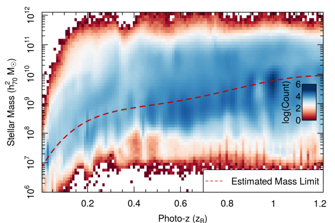
Fig. 10. Distribution of all KV450 galaxy stellar mass estimates as a function of photo- z . The data is shown as a 2D-histogram with logarithmic scaling. The distribution is fairly consistent with what is expected of a magnitude limited galaxy sample, although the incompleteness at low- z is worth noting. The distribution is fairly uniform above the mass limits (red dashed line). Below the limits we see signs of systematic incompleteness and redshift focussing (caused by the typically noisier data there).
