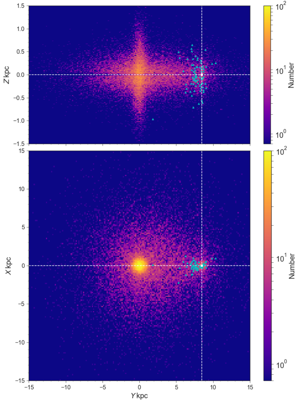
Figure 2: Source-count maps of DWDs detected by LISA ( \text{SNR} > 7 ) in the Galactocentric Cartesian coordinate system: in the Y-Z plane (top panel) and in the Y-X plane (bottom panel). The white square identifies the position of the Sun in our mock Galaxy, (0, 8.5 \text{ kpc}, 0) . Blue triangles represent the position of EM counterparts detected with Gaia and/or LSST. Figure adopted from Korol et al. (2019).
