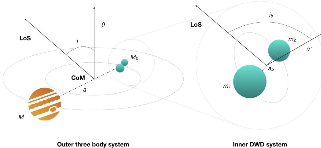
Fig. 1. Geometry of the outer three-body system (DWD+planet/BD) and inner compact two-body system (DWD). The quantities \hat{u} and \hat{u}' denote the directions perpendicular to the outer and inner orbital planes, respectively. The acronyms LoS and CoM stand instead for line of sight and centre of mass (of the whole three-body system).
