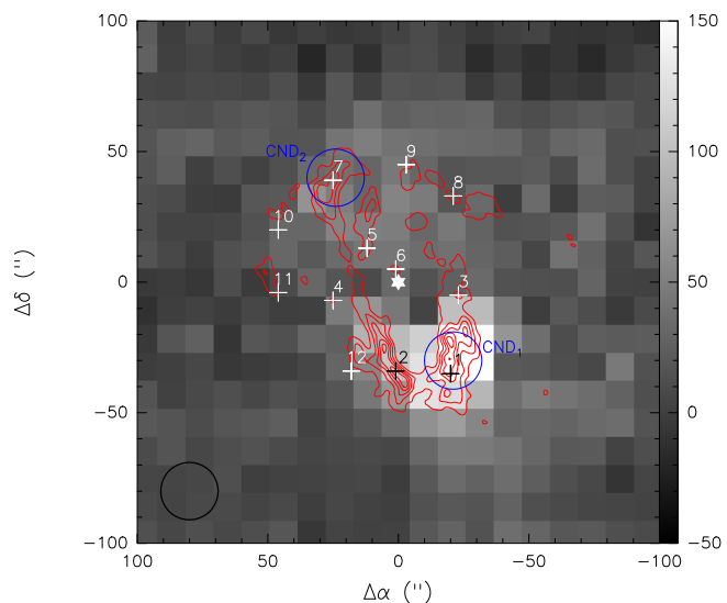
Fig. 6. Comparison between the integrated intensity maps of 988 GHz H_2O in gray and CN(2–1) (contours, Martín et al. (2012)). The integrated velocity range of the H_2O map is [-180, 140] km s -1 . The wedge at the right shows the H_2O intensity gray scale in K km s -1 . Crosses and their numbers show positions, where spectra used in the kinematic study were extracted over the 22'' beam. These positions correspond to selected CN(2–1) and H_2CO(3_{30}-2_{20}) emission peaks on the CN (Martín et al. 2012). The white star shows the position of Sgr A* and origin of the offsets. The HIFI beam of 22'' at 988 GHz is shown in the left corner. Contour levels of the CN map start at 3\sigma and increase in 4\sigma steps. 22'' blue circles show the CN D1 and CN D2 positions selected for our study of the water excitation (see Section 5). The CN D1 and CN D2 positions were observed towards the southwest and northeast lobes, respectively, of the CN (Requena-Torres et al. 2012).
