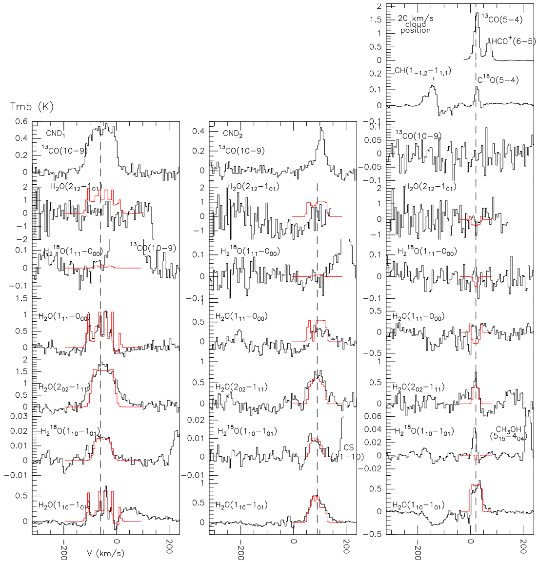
Fig. 7. Observational and simulated \text{H}_2\text{O} and \text{H}_2^{18}\text{O} line profiles. ( Left panel ) Observational spectra (black histograms) of 4 and 2 transitions of \text{H}_2\text{O} and \text{H}_2^{18}\text{O} , respectively, for the \text{CND}_1 position. The modeled water line profiles obtained using a two component model are shown with red histograms. We also show the ^{13}\text{CO}(10-9) line profile. ( Central panel ) Observational spectra (black histograms) of 4 and 2 transitions of \text{H}_2\text{O} and \text{H}_2^{18}\text{O} , respectively, for the \text{CND}_2 position. The modeled water line profiles obtained utilizing a two component model are shown with red histograms. ^{13}\text{CO}(10-9) and \text{CS}(11-10) line profiles are also shown, but the \text{CS}(11-10) line (near the \text{H}_2^{18}\text{O}(1_{10}-1_{01}) line) appears as a consequence of the HIFI double sideband. ( Right panel ) Observational spectra (black histograms) of 4 and 2 transitions of \text{H}_2\text{O} and \text{H}_2^{18}\text{O} , respectively, for the 20 \text{ km s}^{-1} cloud position. The modeled water line profiles are shown with red histograms. ^{13}\text{CO}(10-9) , \text{C}^{18}\text{O}(5-4) , ^{13}\text{CO}(5-4) , \text{CH}_3\text{OH}(5_{15}-4_{04}) , \text{CH}(1_{-1,2}-1_{1,1}) and \text{HCO}^+(6-5) spectral features are also shown, with the last three lines coming from the HIFI double sideband. The \text{H}_2^{18}\text{O}(1_{10}-1_{01}) line is blended with the ^{13}\text{CH}_3\text{OH}(1_{62}-1_{61}) line (this line also is due to the HIFI double sideband).
