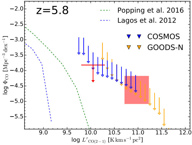
Figure 4. VLA COLDz CO( J=2\rightarrow 1 ) luminosity function at \langle z \rangle = 5.68 and 5.86 in the COSMOS (blue and red arrows) and GOODS-North (orange arrows and red boxes) fields, respectively. The blue and orange arrows show upper limits under the unlikely assumption that any candidates not independently confirmed to be CO( J=1\rightarrow 0 ) emission would correspond to CO( J=2\rightarrow 1 ) emission, for the same binning in L'_{\text{CO}} as in Fig. 2. Red arrows and boxes consider only independently confirmed CO( J=2\rightarrow 1 ) candidates. The dashed lines show model predictions.
